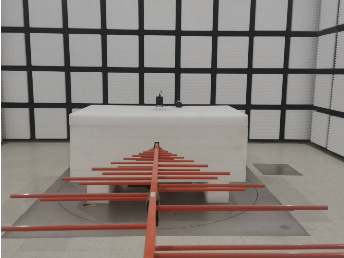
Radiated Emission Below 1GHz View-U2B
