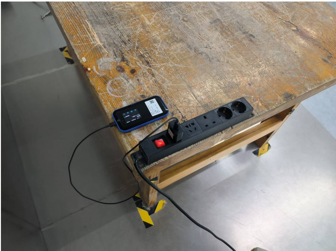
Conducted Emissions Side View-U2B
