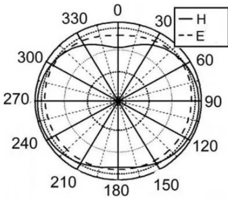
27.145 MHz radiation pattern
