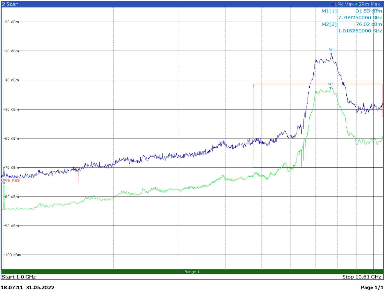
Figure 7.6-8: Radiated spurious emissions 1 to 10.61 GHz (RSS Limits), with antenna in vertical polarization
