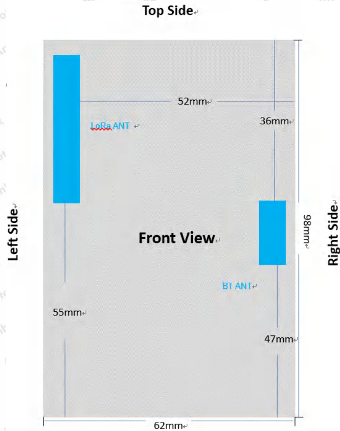
EUT FRONT VIEW
