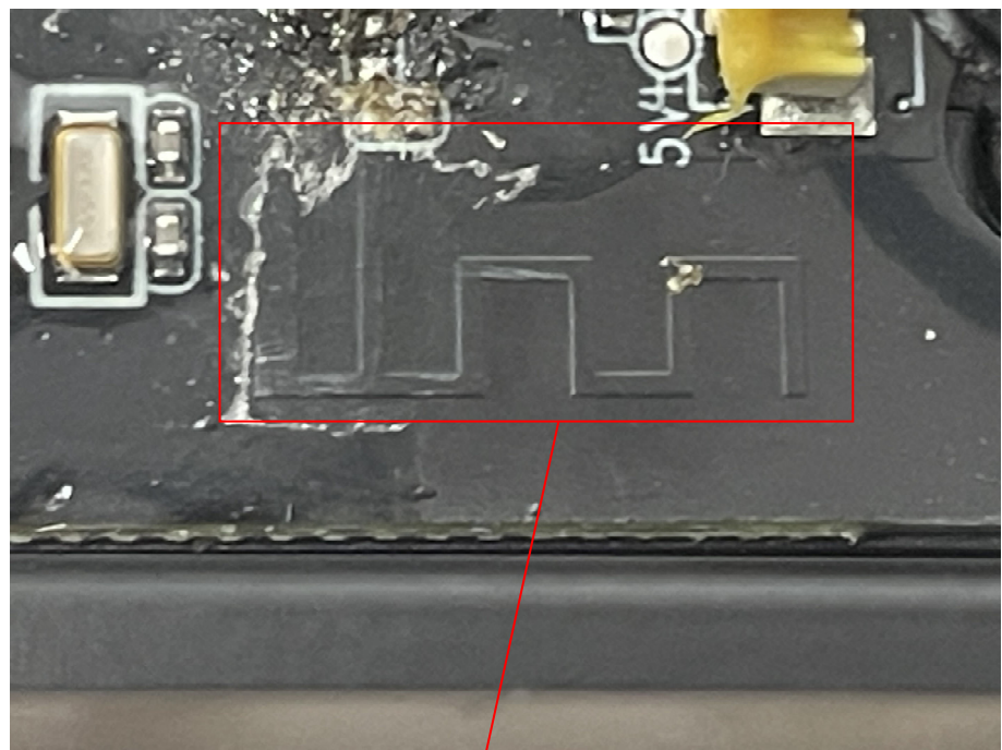
HS6621 Bluetooth Antenna
