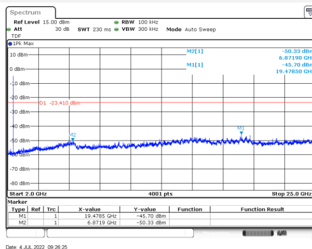
GFSK (BLE 1Mbps) LOW CHANNEL, SPURIOUS 2 GHz ~ 25 GHz
