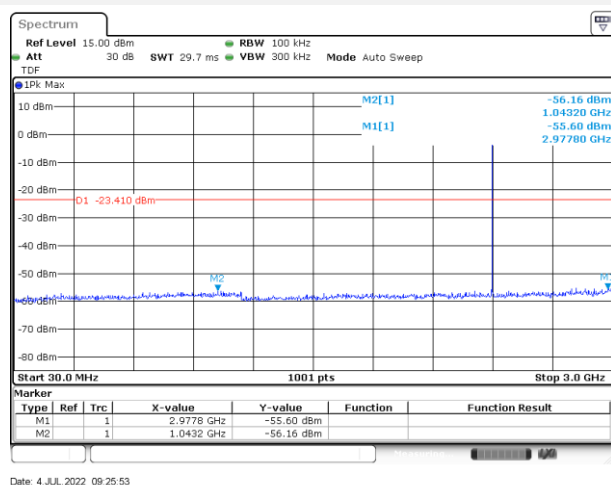
GFSK (BLE 1Mbps) LOW CHANNEL, SPURIOUS 30 MHz ~ 3 GHz
