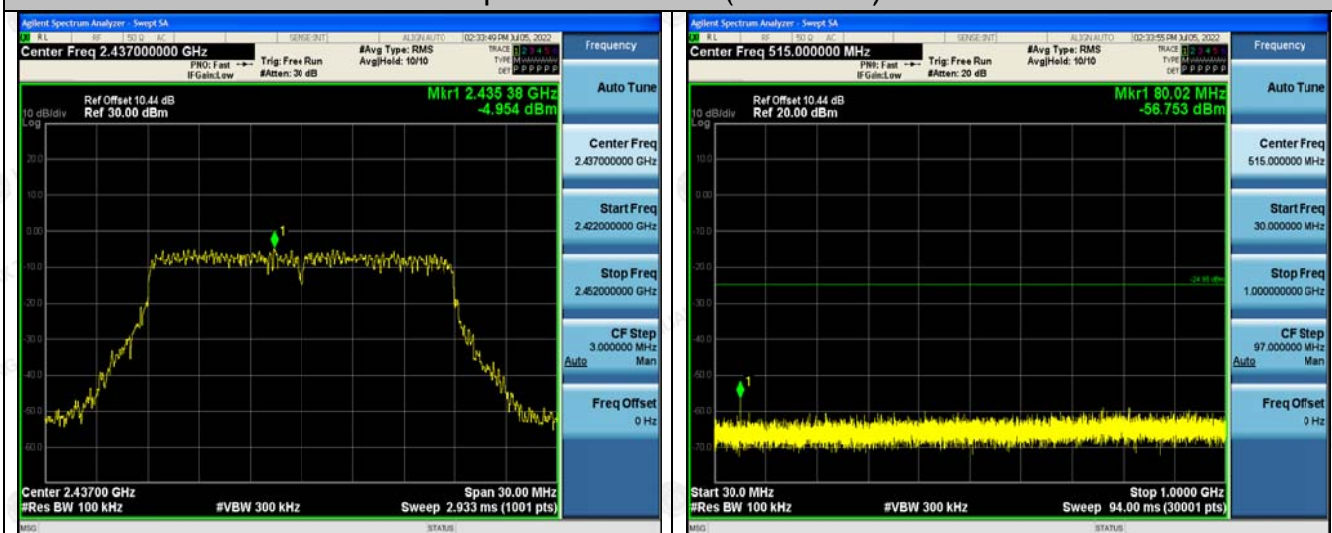
Spurious emission(2437MHz)
