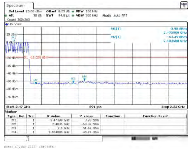
2DH5(2480)-Hopping on
