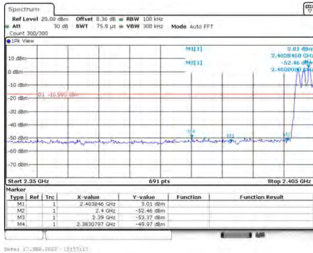
2DH5(2402)-Hopping on
