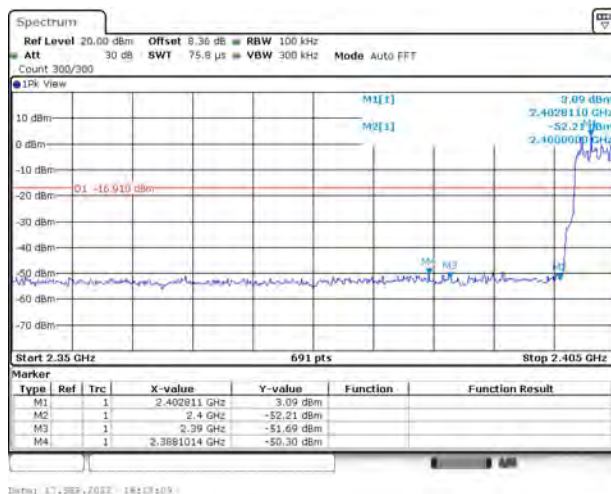
3DH5(2402)-Hopping on
