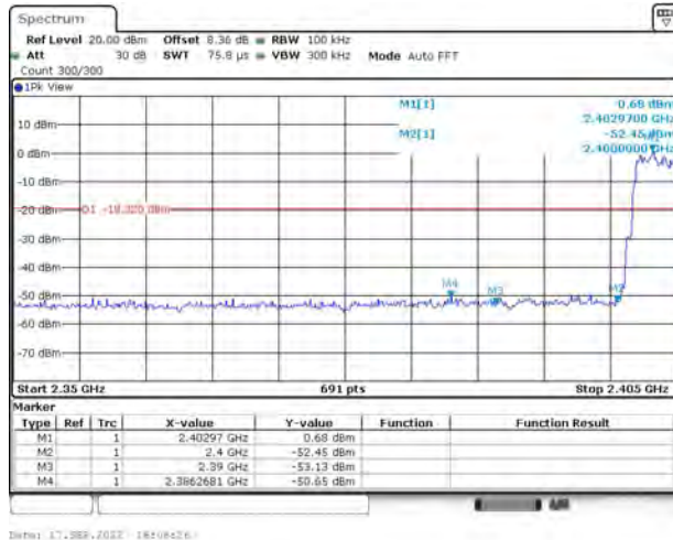
3DH5(2402)-Hopping on
