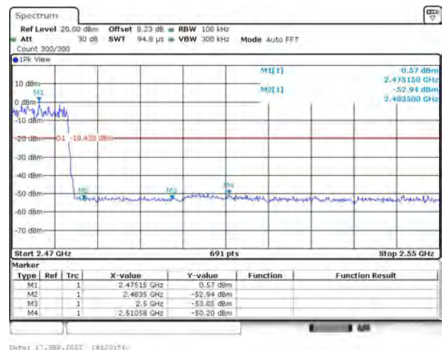
3DH5(2480)-Hopping on
