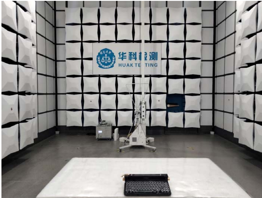
Model: FINEDAY KEYBOARD 3.0 Radiated Emissions
