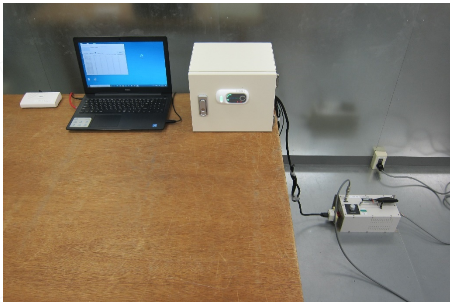
Conducted emissions
