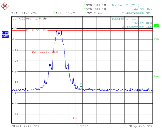
2M BLE: Band edge-right side
