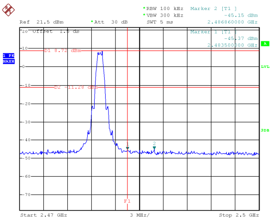
1M BLE: Band edge-right side
