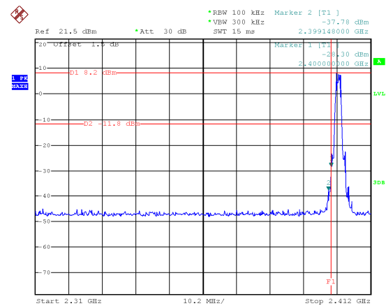
2M BLE: Band edge-left side
