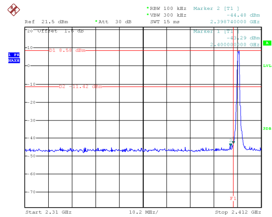
1M BLE: Band edge-left side
