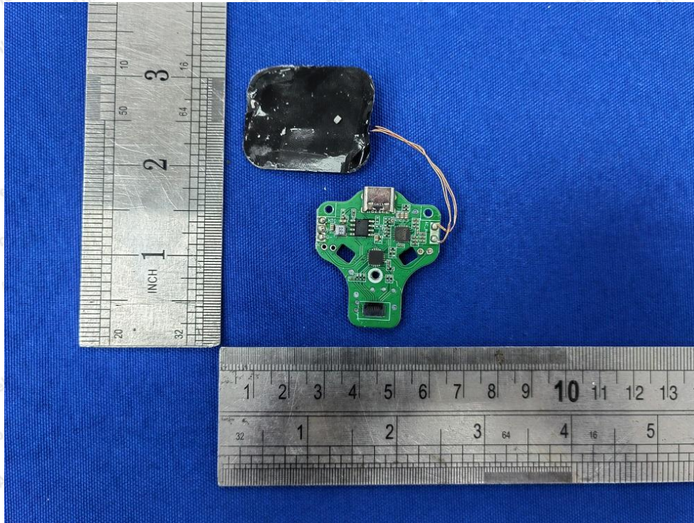
Wireless charging Receive antenna
