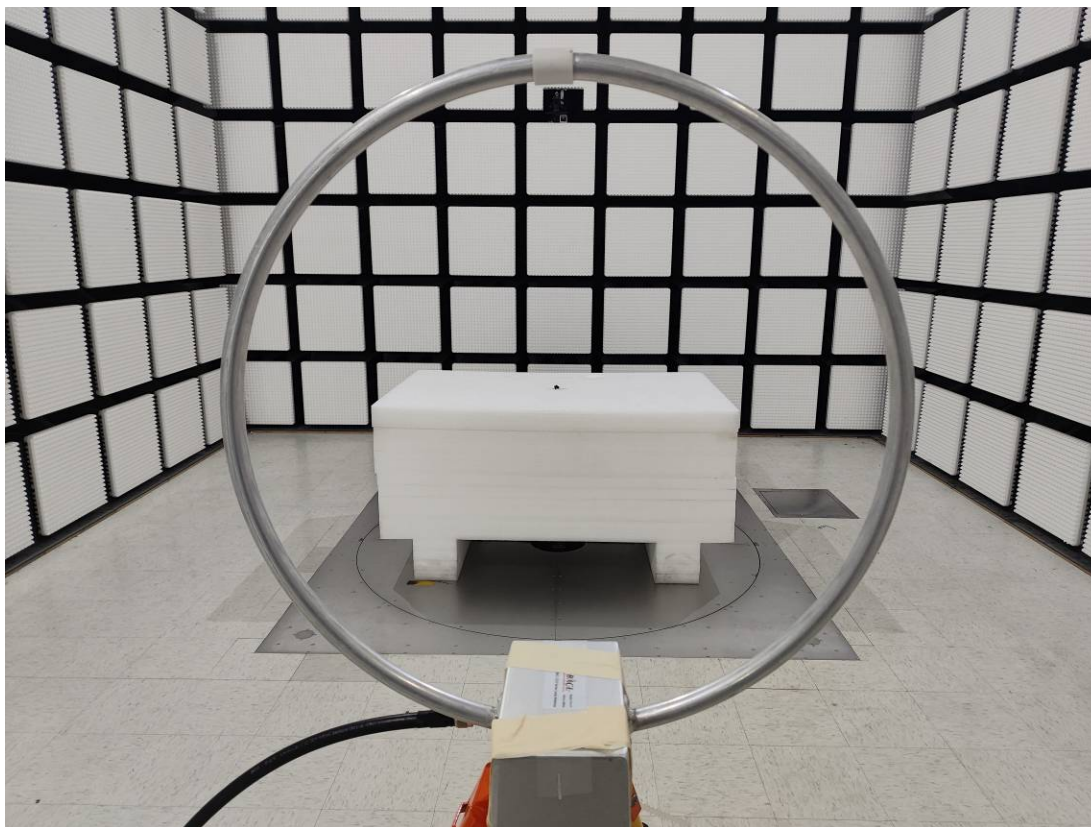
Radiated Emission Below 1GHz View Parallel-left ear
