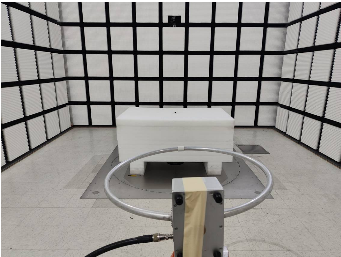
Radiated Emission Below 1GHz View Ground-parallel-left ear
