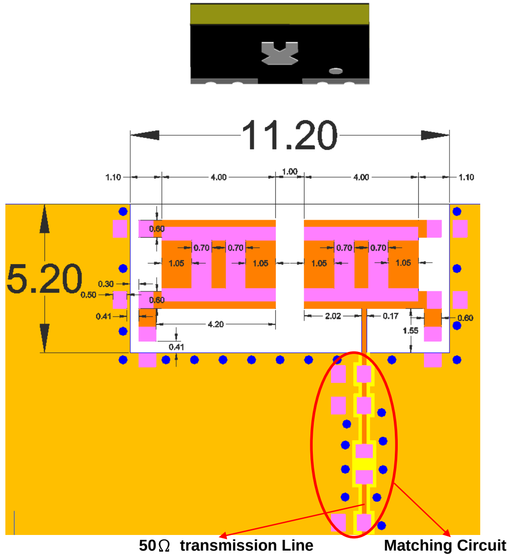
FootPrint (Unit : mm)
