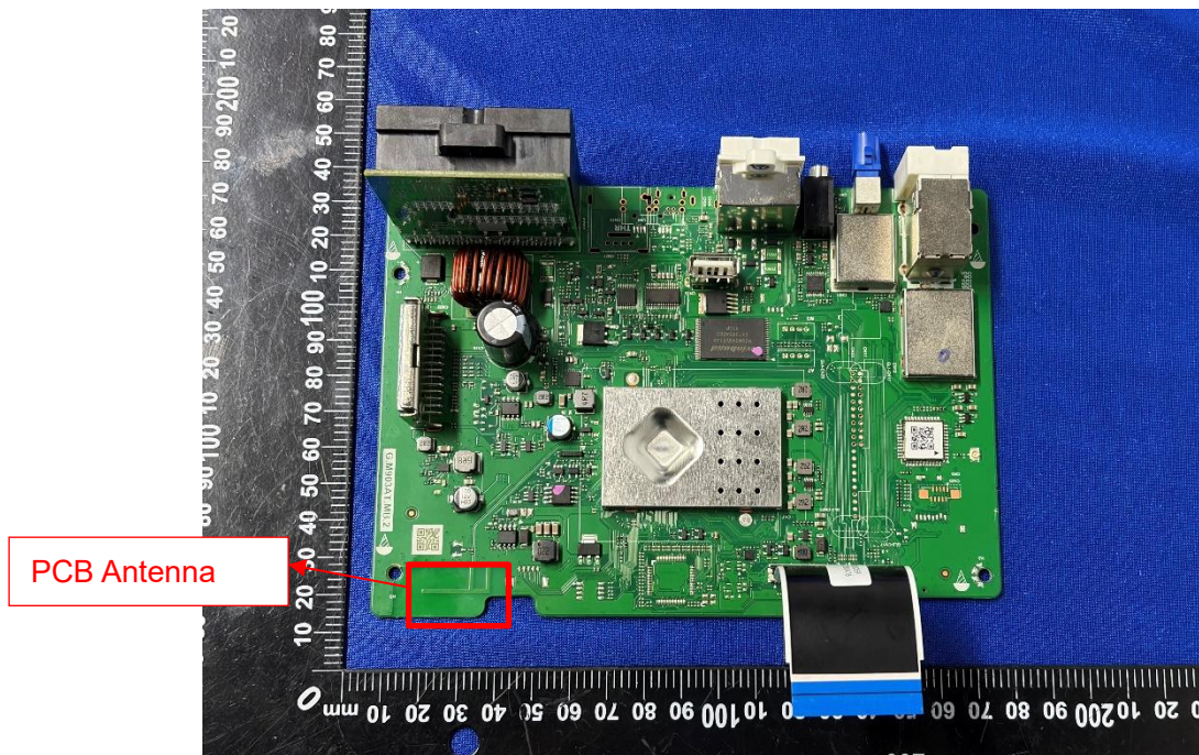
MAIN BOARD TOP VIEW (WITH SHIELDING)
