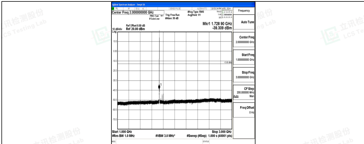
Band4_1.4MHz_QPSK_20175_1RB#0_1000~3000_1000~3000
