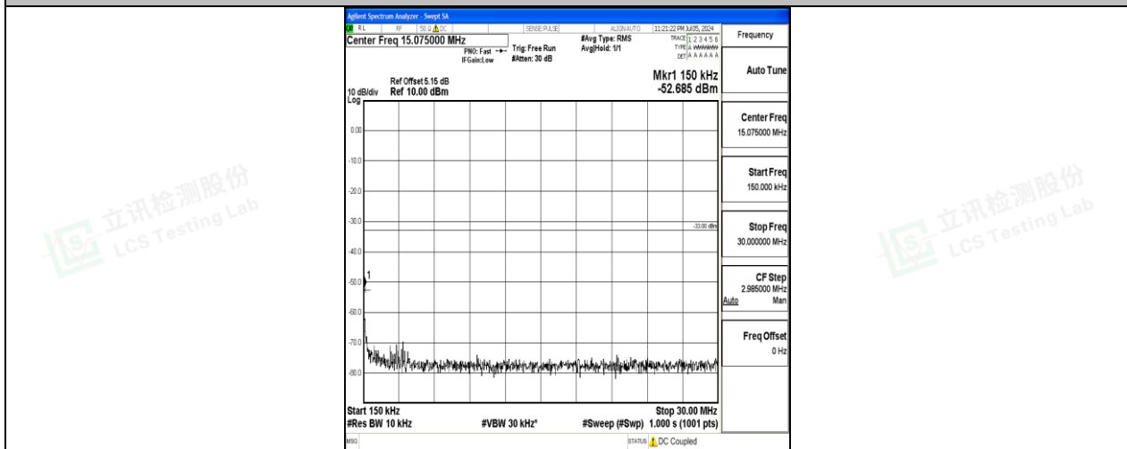
Band4_3MHz_16QAM_19965_1RB#0_0.15~30_0.15~30
