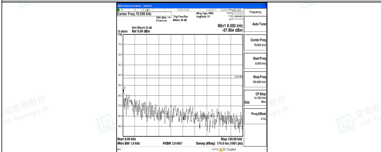
Band4_3MHz_16QAM_19965_1RB#0_0.009~0.15_0.009~0.15
