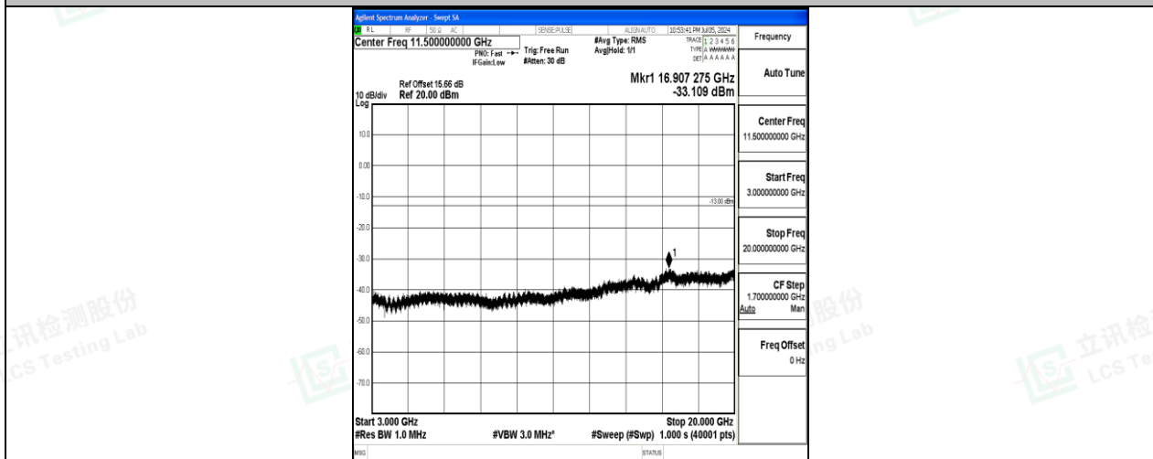
Band4_1.4MHz_QPSK_20175_1RB#0_3000~20000_3000~20000
