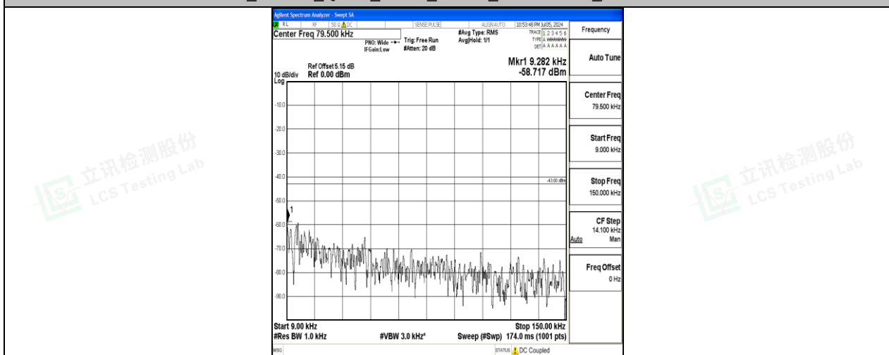
Band4_1.4MHz_16QAM_20175_1RB#0_0.009~0.15_0.009~0.15
