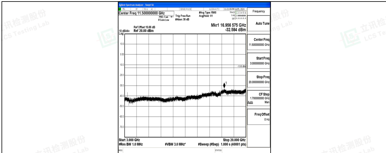
Band4_3MHz_QPSK_19965_1RB#0_3000~20000_3000~20000
