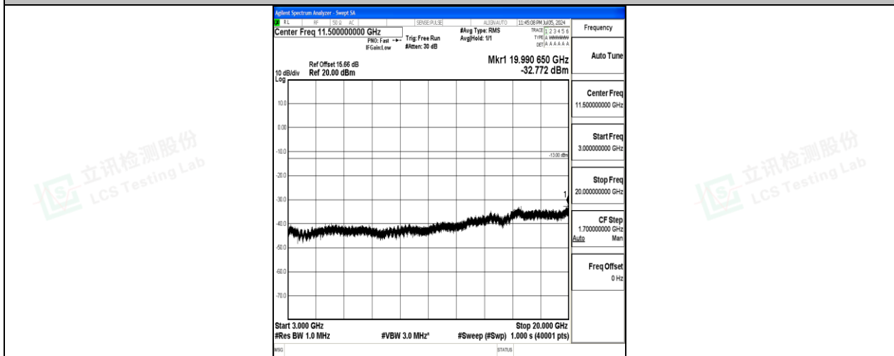
Band4_5MHz_QPSK_20375_1RB#0_3000~20000_3000~20000
