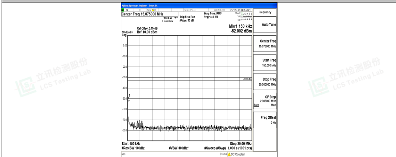
Band4_15MHz_QPSK_20325_1RB#0_0.15~30_0.15~30
