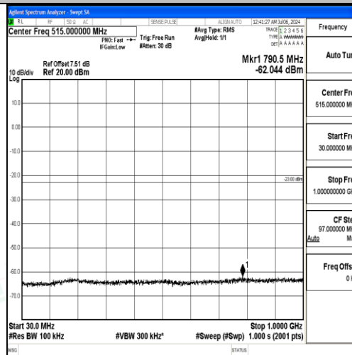
Band4_20MHz_QPSK_20050_1RB#0_30~1000_30~1000
