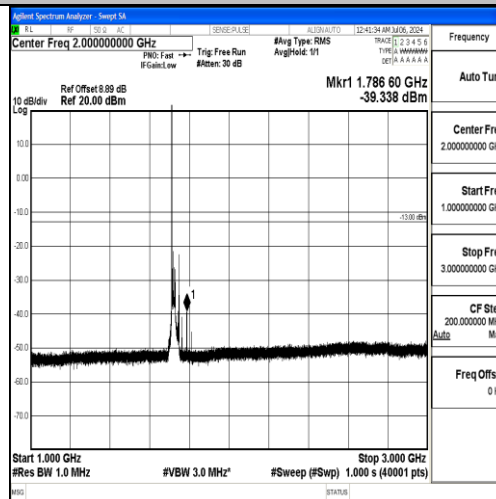
Band4_20MHz_QPSK_20050_1RB#0_1000~3000_1000~3000
