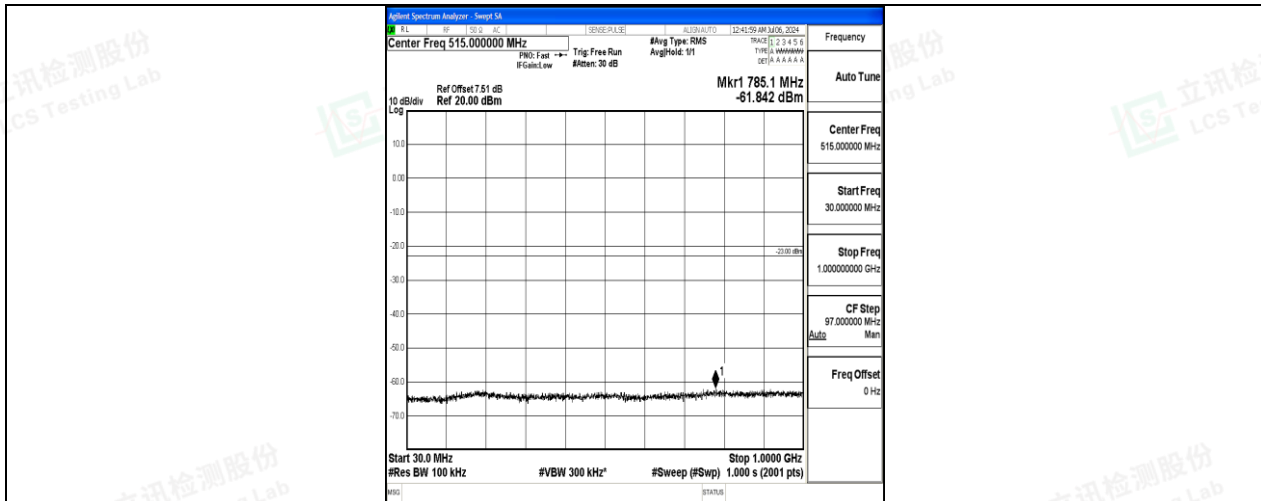
Band4_20MHz_16QAM_20050_1RB#0_30~1000_30~1000
