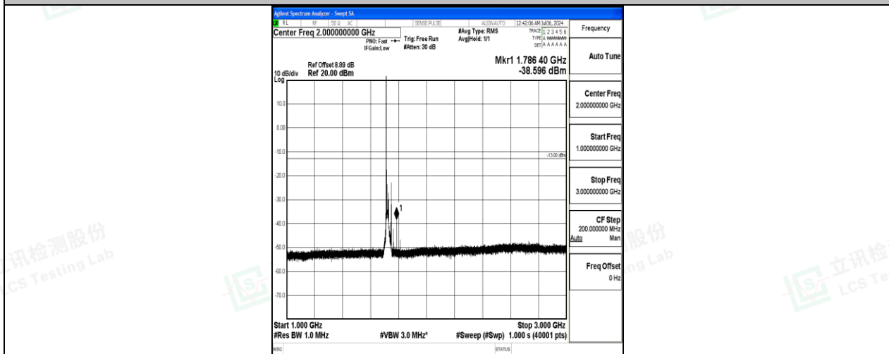
Band4_20MHz_16QAM_20050_1RB#0_1000~3000_1000~3000
