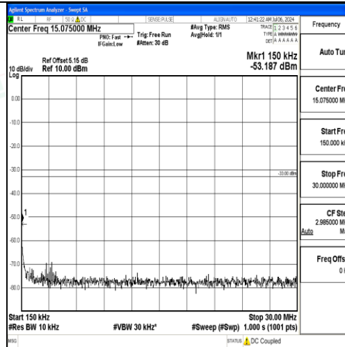
Band4_20MHz_QPSK_20050_1RB#0_0.15~30_0.15~30
