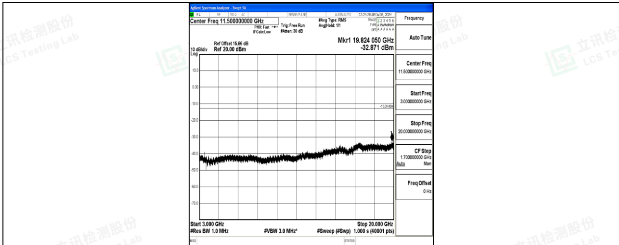
Band4_15MHz_16QAM_20175_1RB#0_3000~20000_3000~20000
