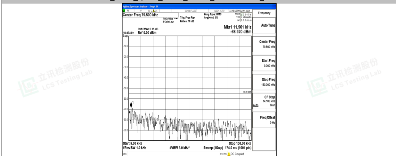
Band7_5MHz_16QAM_21425_1RB#0_0.009~0.15_0.009~0.15
