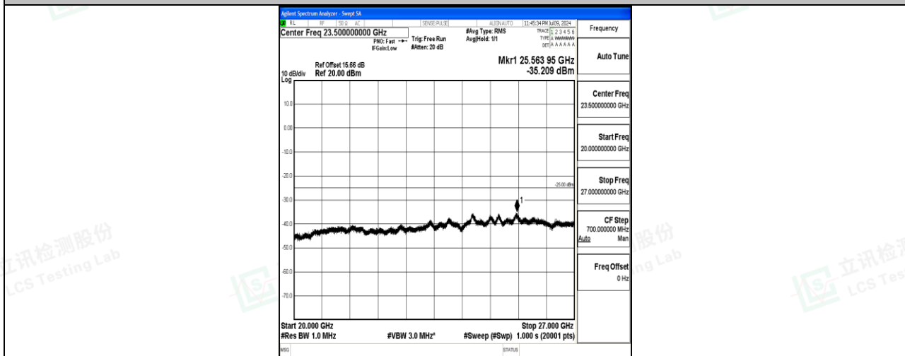
Band7_5MHz_16QAM_21100_1RB#0_20000~27000_20000~27000
