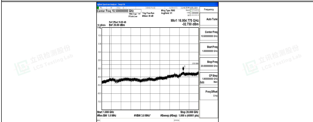
Band7_5MHz_16QAM_21425_1RB#0_1000~20000_1000~20000
