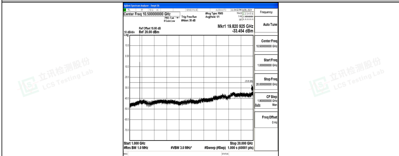
Band7_10MHz_QPSK_21400_1RB#0_1000~20000_1000~20000
