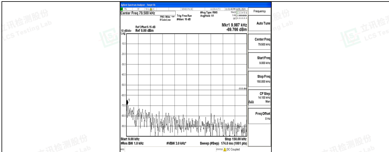
Band7_10MHz_QPSK_20800_1RB#0_0.009~0.15_0.009~0.15
