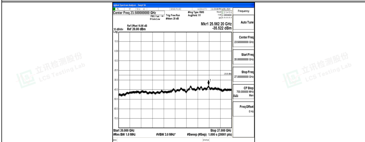
Band7_10MHz_QPSK_21100_1RB#0_20000~27000_20000~27000
