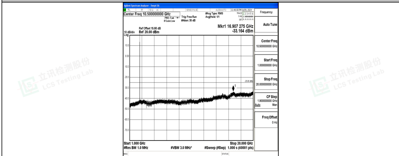
Band7_5MHz_QPSK_21425_1RB#0_1000~20000_1000~20000
