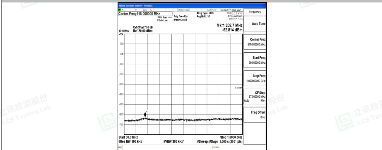
Band7_10MHz_16QAM_20800_1RB#0_30~1000_30~1000
