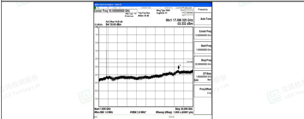
Band7_10MHz_16QAM_21400_1RB#0_1000~20000_1000~20000
