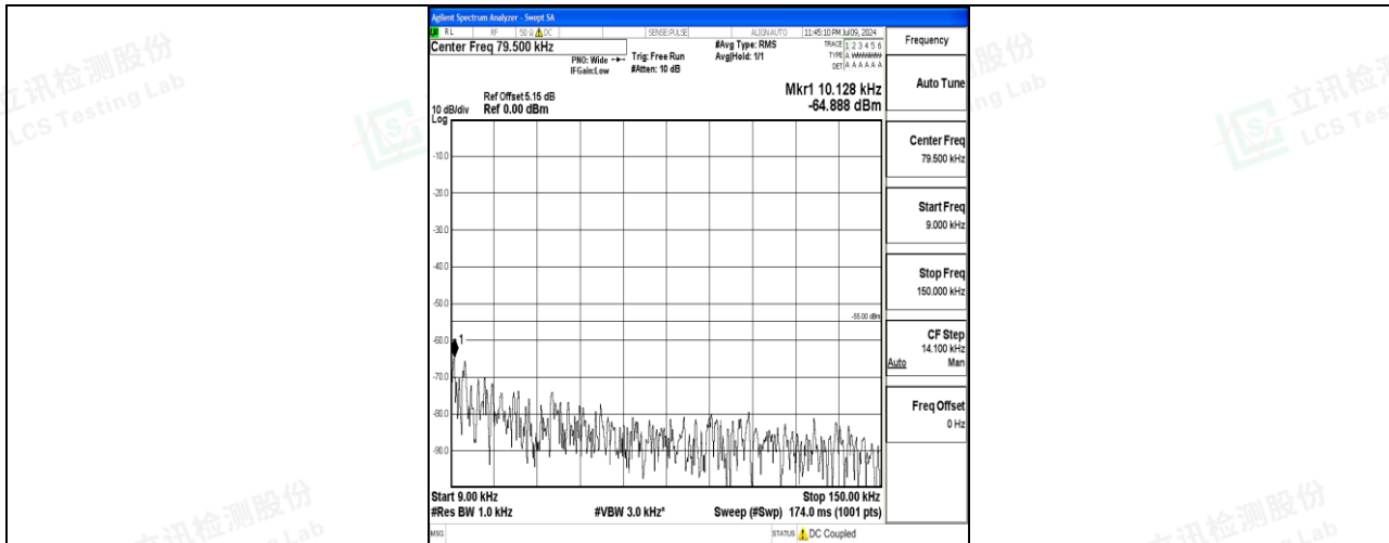
Band7_5MHz_16QAM_21100_1RB#0_0.009~0.15_0.009~0.15
