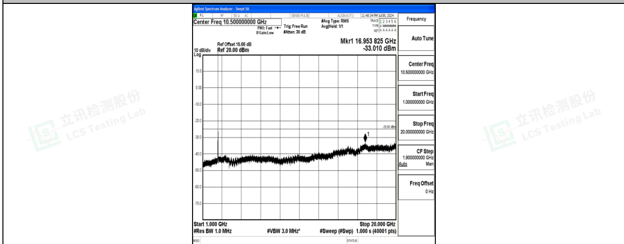
Band7_15MHz_16QAM_20825_1RB#0_1000~20000_1000~20000
