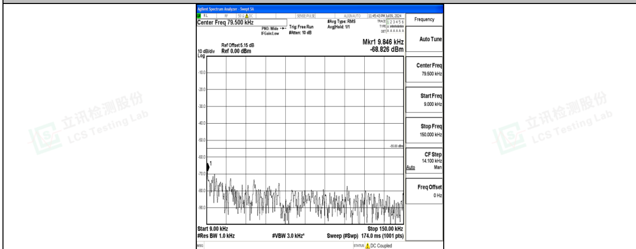
Band7_5MHz_QPSK_21425_1RB#0_0.009~0.15_0.009~0.15
