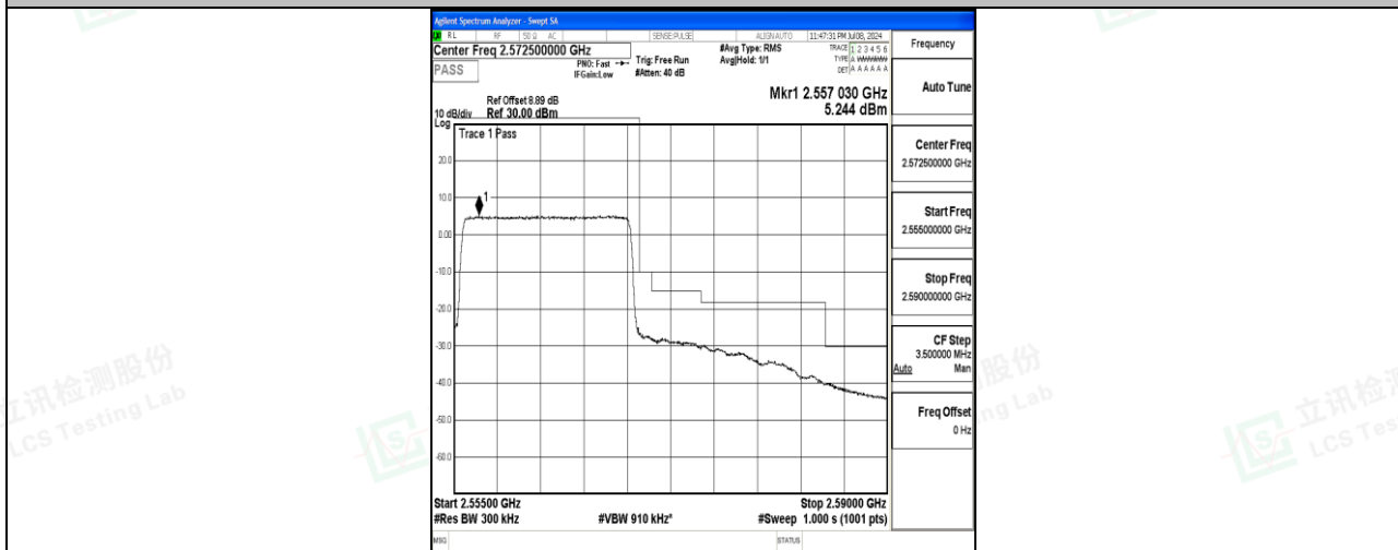
Band7_15MHz_16QAM_21375_75RB#0
