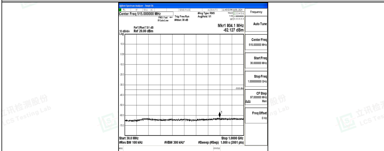
Band7_5MHz_QPSK_21425_1RB#0_30~1000_30~1000
