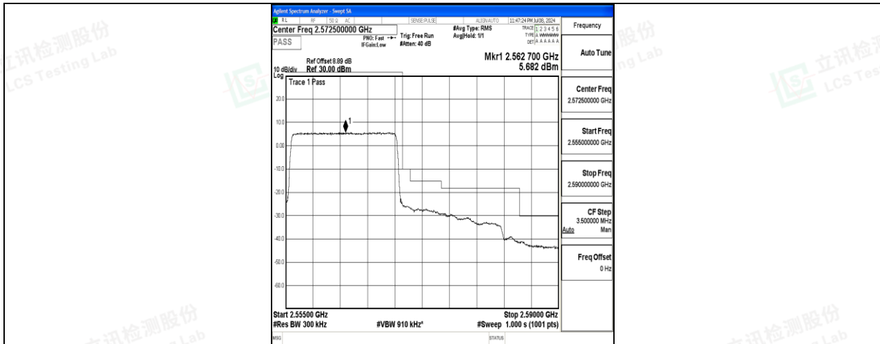
Band7_15MHz_QPSK_21375_75RB#0
