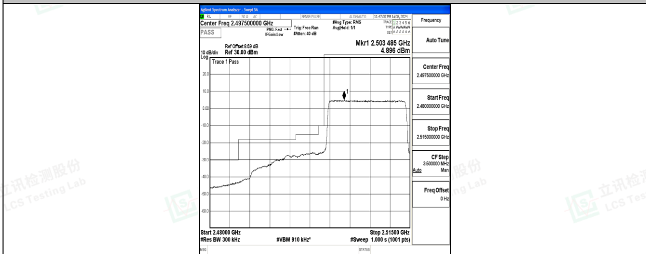
Band7_15MHz_QPSK_20825_75RB#0
