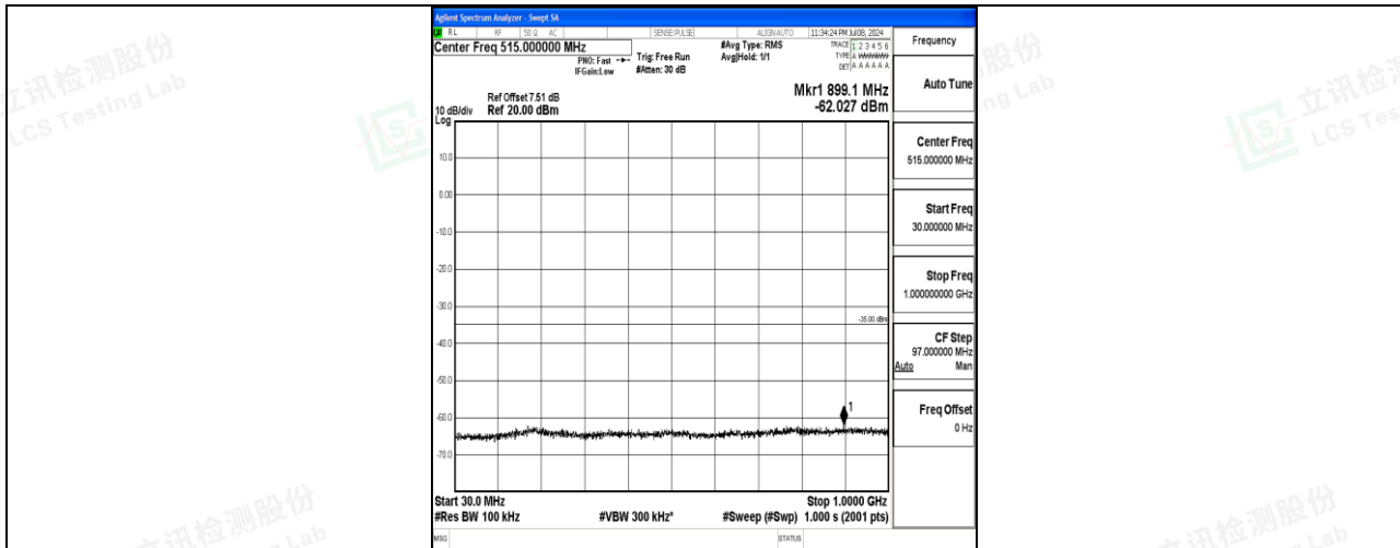
Band7_10MHz_16QAM_21400_1RB#0_30~1000_30~1000
