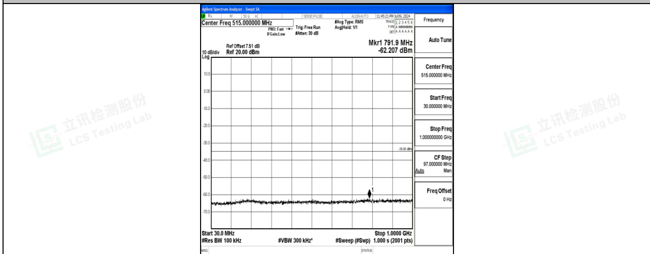
Band7_5MHz_16QAM_21100_1RB#0_30~1000_30~1000
