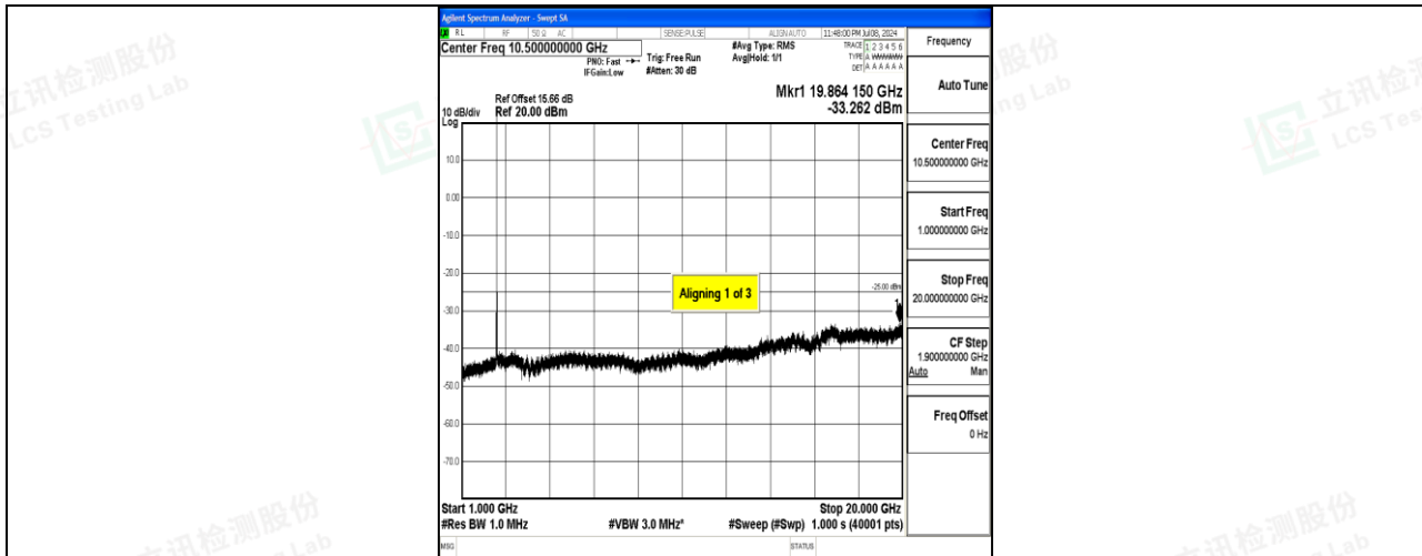
Band7_15MHz_QPSK_20825_1RB#0_1000~20000_1000~20000
