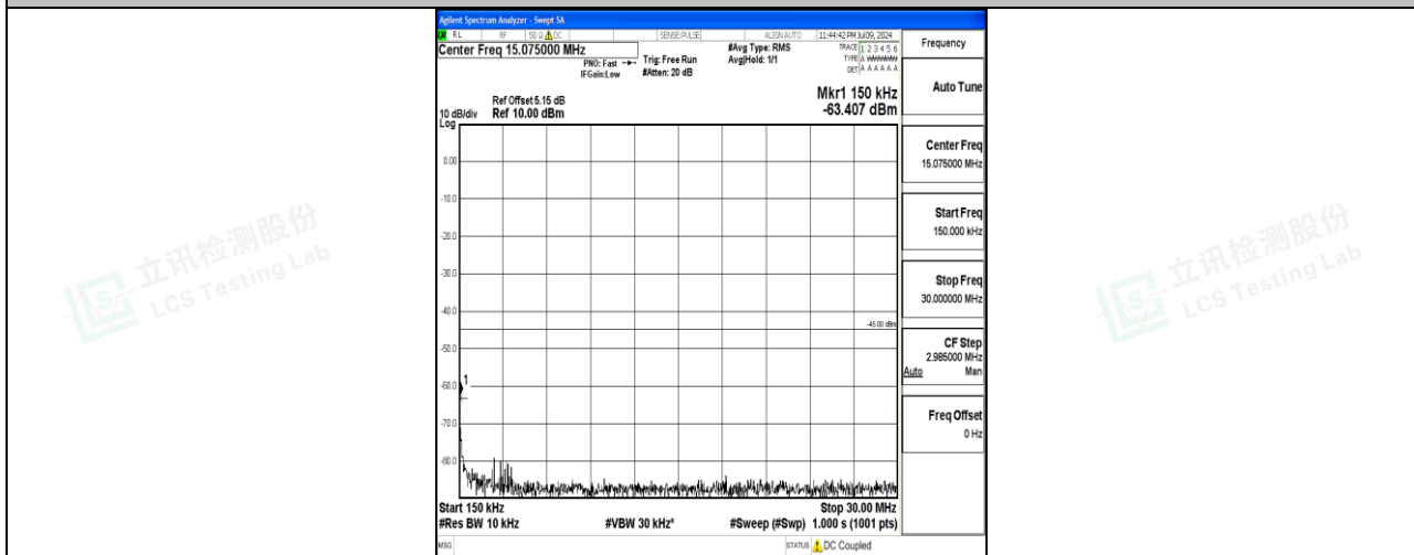
Band7_5MHz_QPSK_21100_1RB#0_0.15~30_0.15~30
