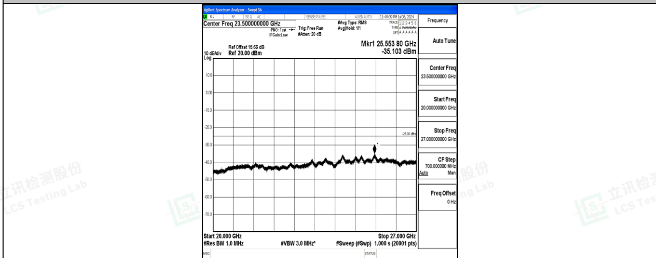
Band7_15MHz_QPSK_20825_1RB#0_20000~27000_20000~27000
