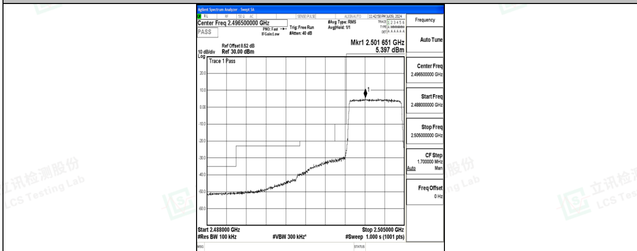
Band7_5MHz_16QAM_20775_25RB#0
