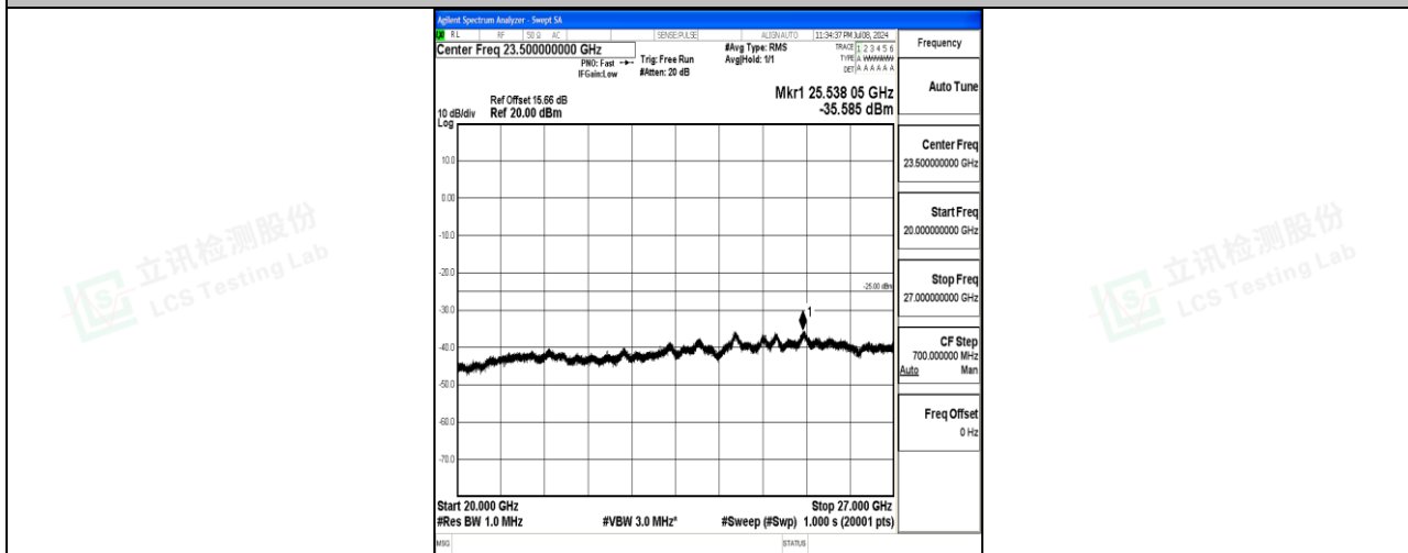
Band7_10MHz_16QAM_21400_1RB#0_20000~27000_20000~27000
