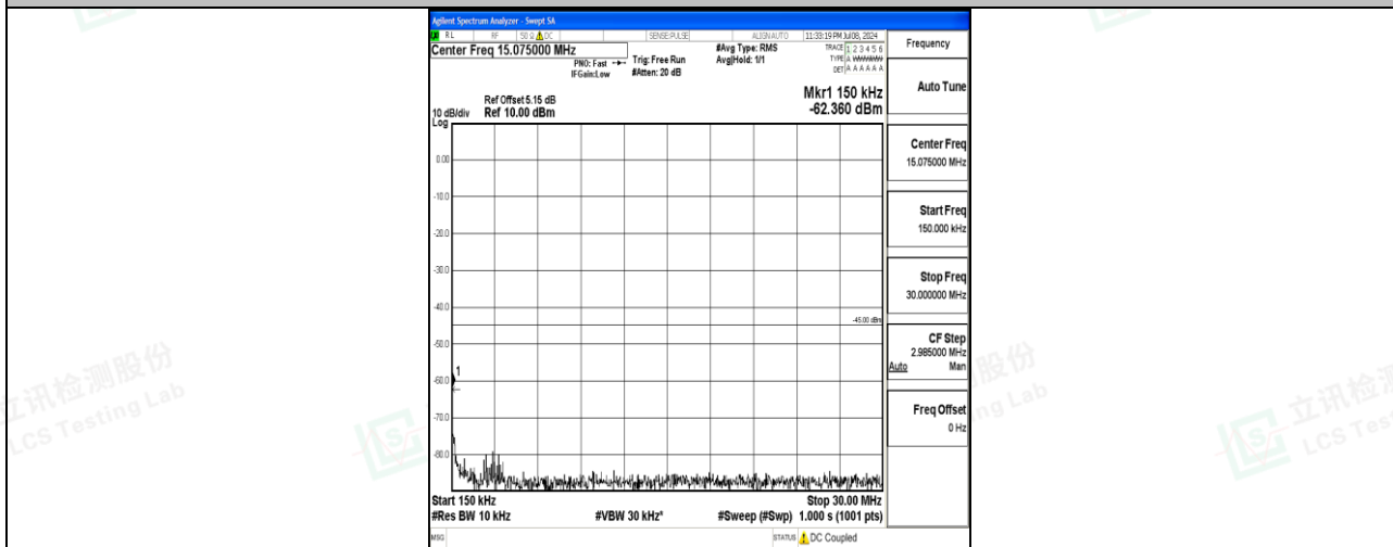
Band7_10MHz_16QAM_21100_1RB#0_0.15~30_0.15~30
