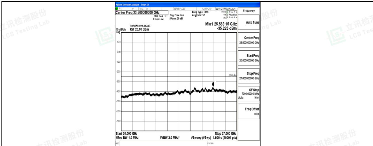
Band7_5MHz_16QAM_20775_1RB#0_20000~27000_20000~27000
