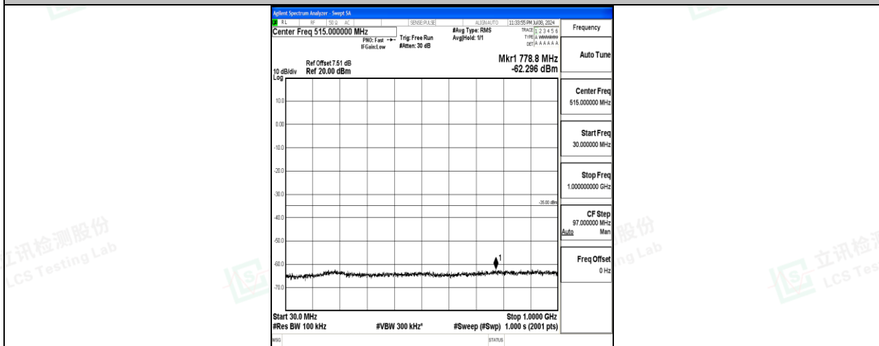
Band7_10MHz_QPSK_21400_1RB#0_30~1000_30~1000
