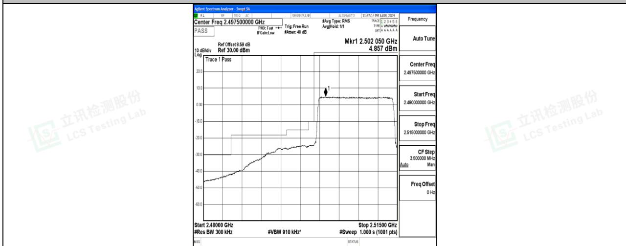
Band7_15MHz_16QAM_20825_75RB#0
