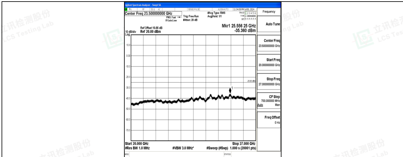
Band7_10MHz_QPSK_21400_1RB#0_20000~27000_20000~27000
