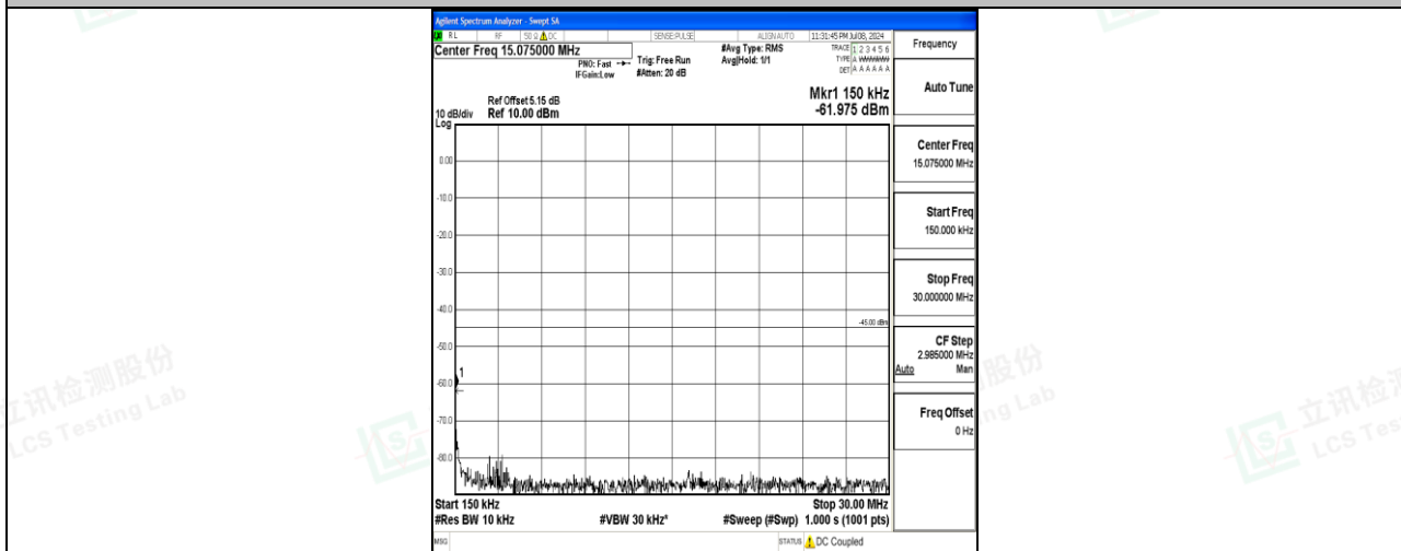
Band7_10MHz_QPSK_20800_1RB#0_0.15~30_0.15~30
