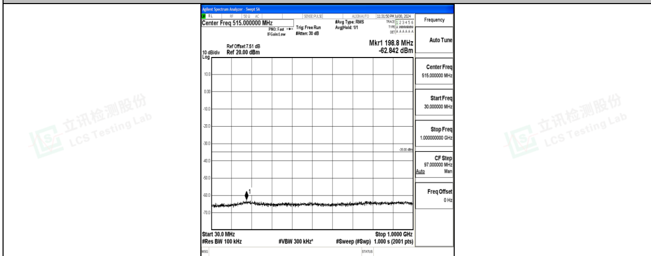
Band7_10MHz_QPSK_20800_1RB#0_30~1000_30~1000
