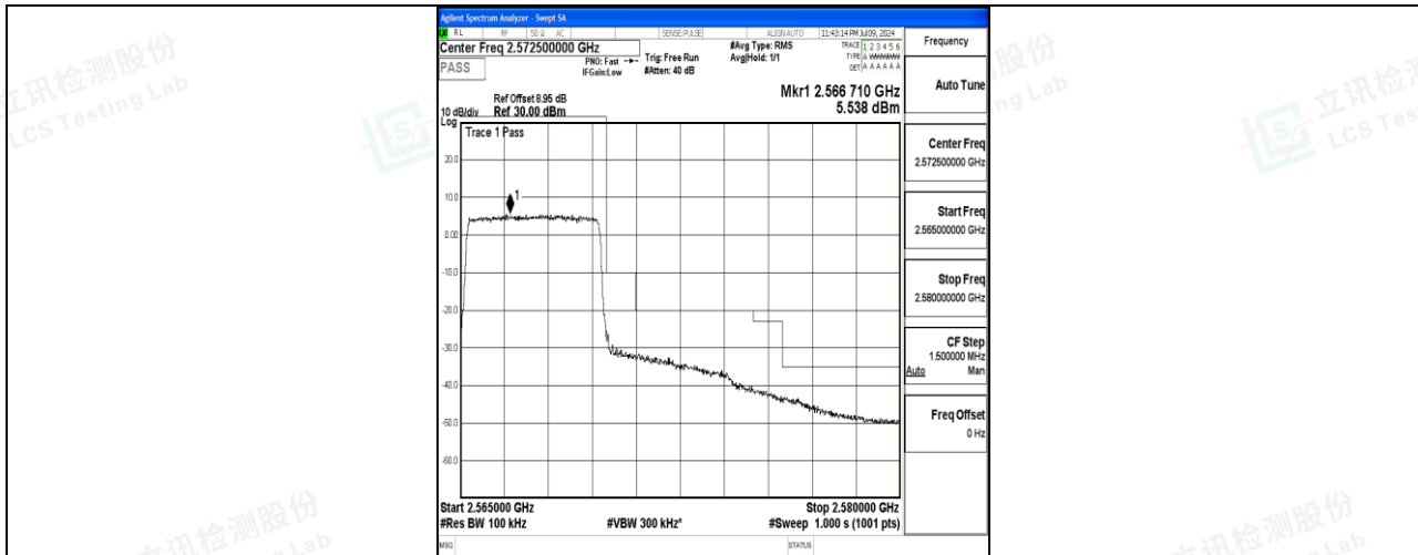
Band7_5MHz_16QAM_21425_25RB#0
