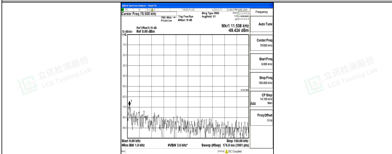
Band7_15MHz_16QAM_20825_1RB#0_0.009~0.15_0.009~0.15
