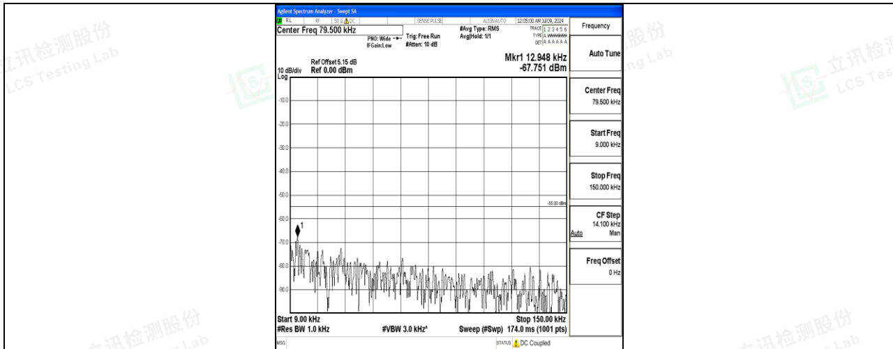
Band7_20MHz_16QAM_21100_1RB#0_0.009~0.15_0.009~0.15
