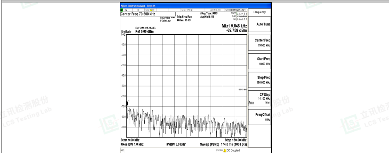
Band7_20MHz_16QAM_21350_1RB#0_0.009~0.15_0.009~0.15
