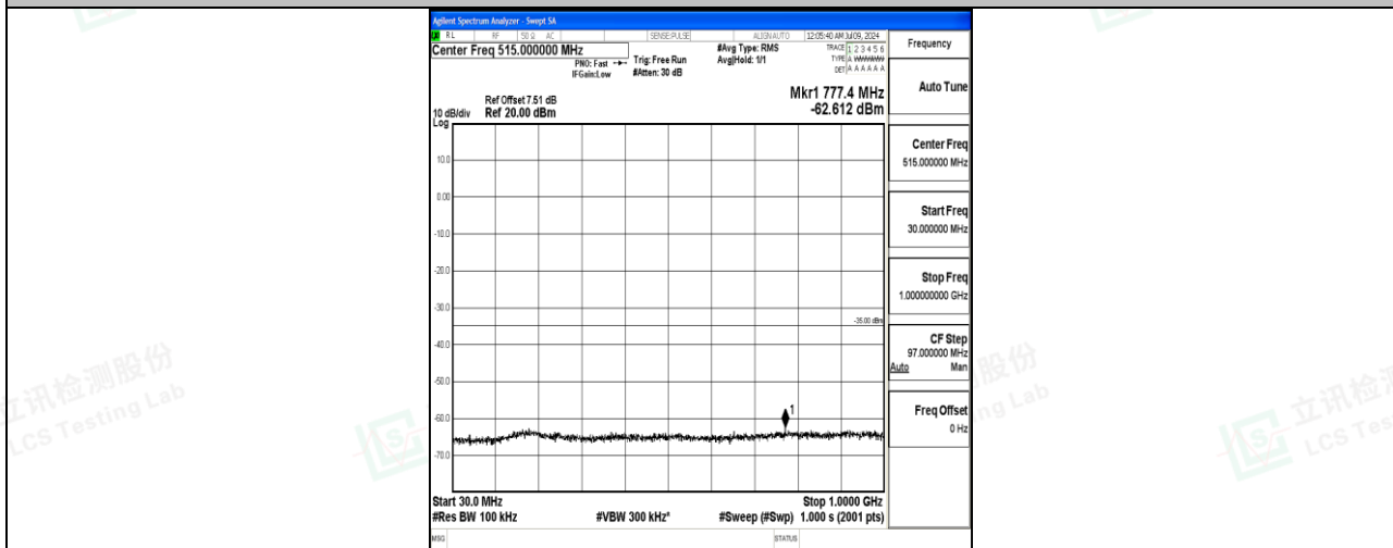
Band7_20MHz_QPSK_21350_1RB#0_30~1000_30~1000
