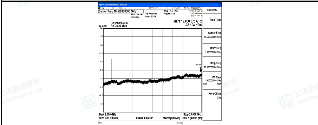
Band7_15MHz_QPSK_21100_1RB#0_1000~20000_1000~20000
