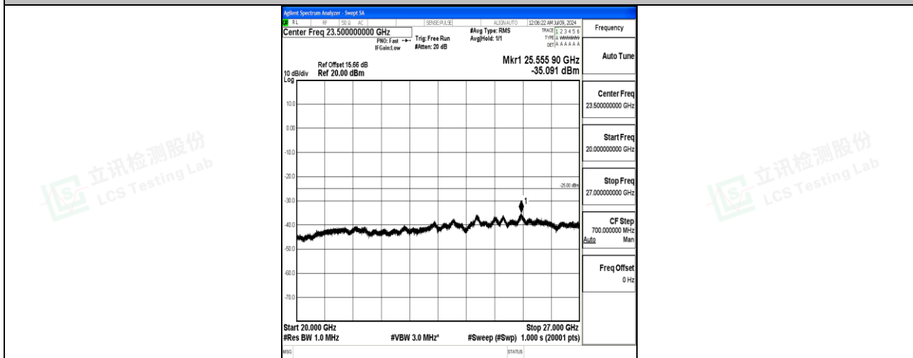
Band7_20MHz_16QAM_21350_1RB#0_20000~27000_20000~27000
