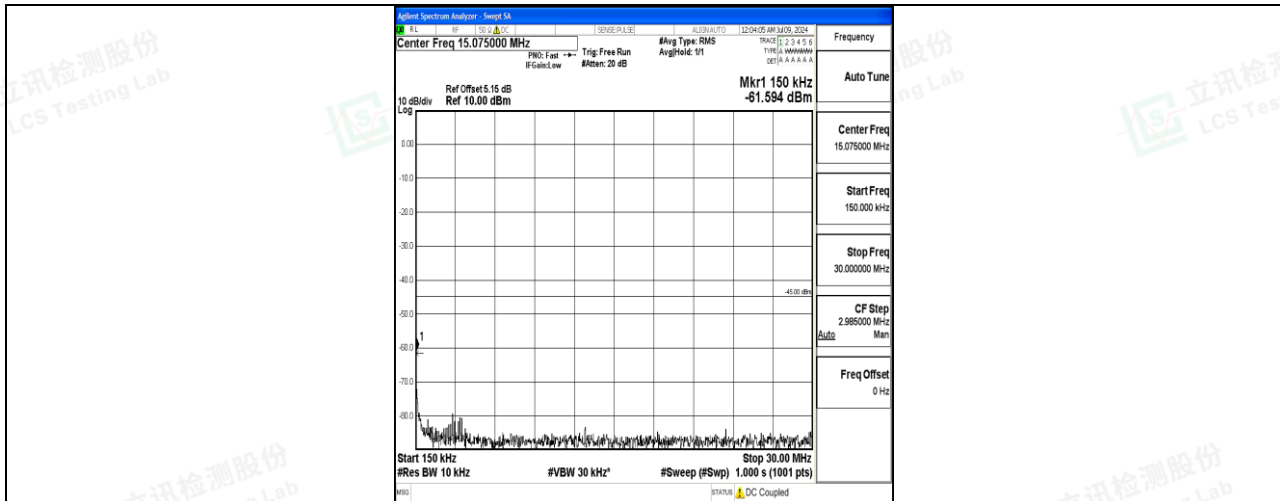
Band7_20MHz_16QAM_20850_1RB#0_0.15~30_0.15~30
