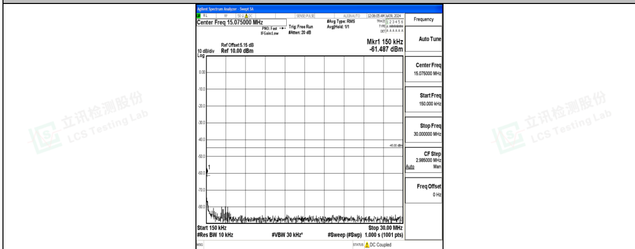
Band7_20MHz_16QAM_21350_1RB#0_0.15~30_0.15~30
