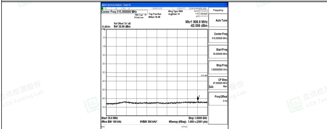
Band7_20MHz_16QAM_20850_1RB#0_30~1000_30~1000
