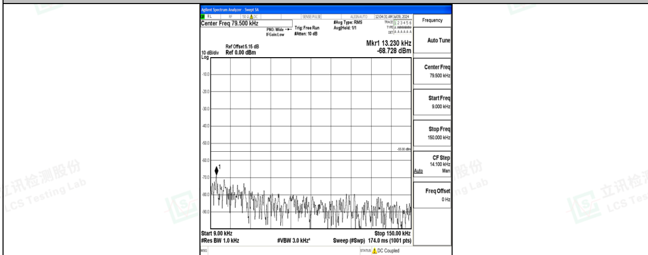
Band7_20MHz_QPSK_21100_1RB#0_0.009~0.15_0.009~0.15
