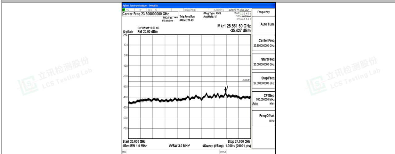
Band7_15MHz_16QAM_21375_1RB#0_20000~27000_20000~27000
