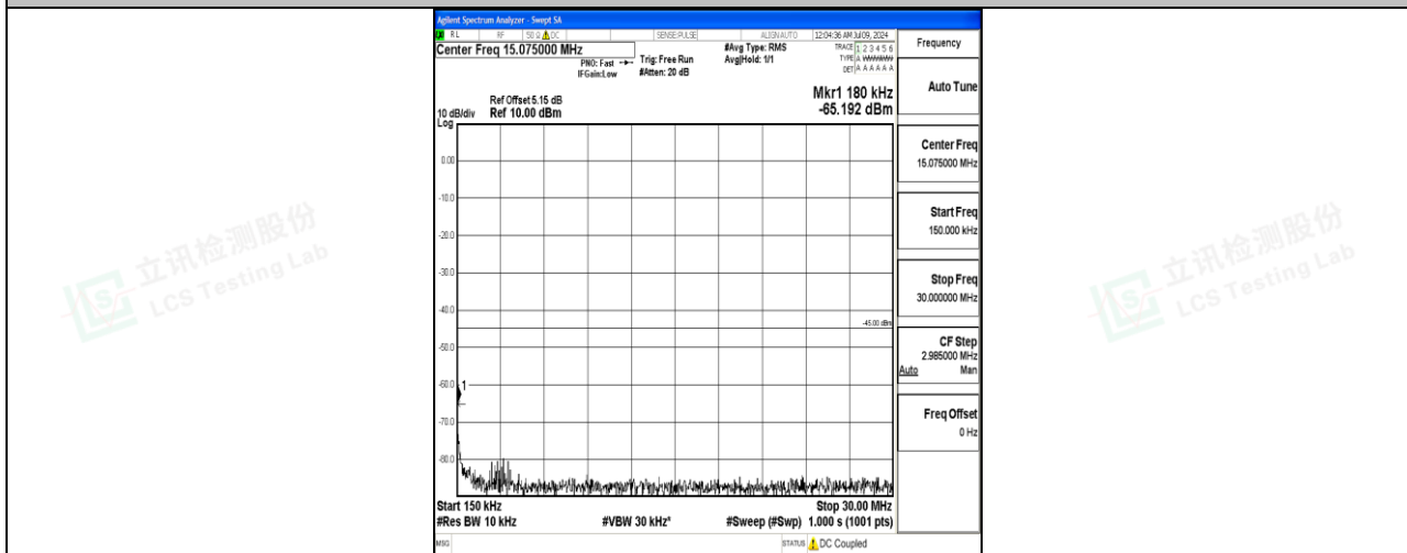
Band7_20MHz_QPSK_21100_1RB#0_0.15~30_0.15~30
