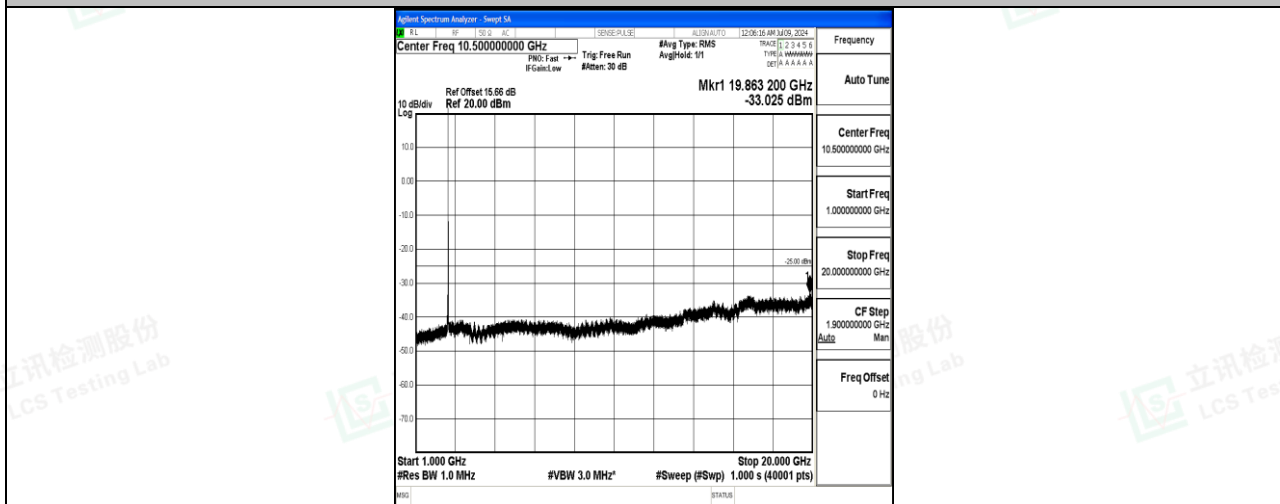
Band7_20MHz_16QAM_21350_1RB#0_1000~20000_1000~20000
