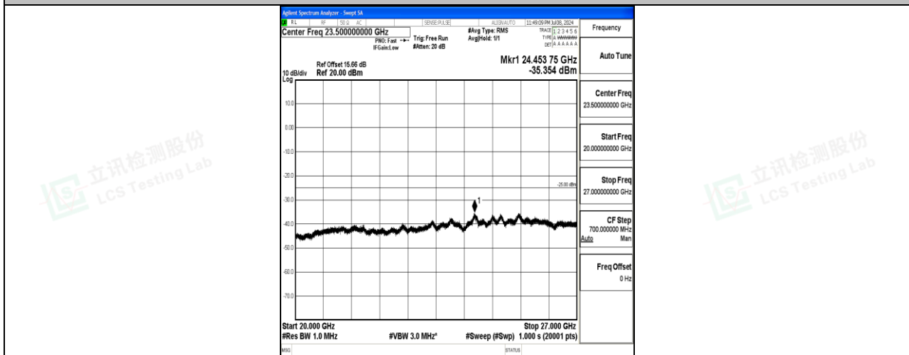
Band7_15MHz_QPSK_21100_1RB#0_20000~27000_20000~27000
