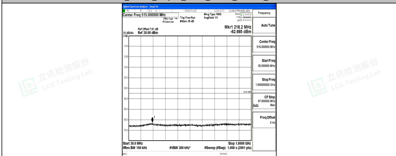
Band7_15MHz_16QAM_21100_1RB#0_30~1000_30~1000
