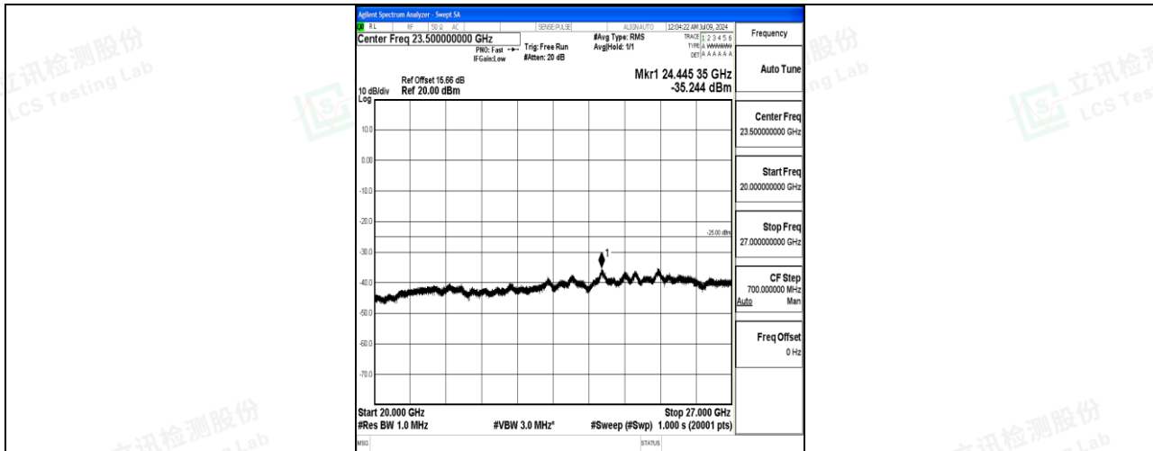
Band7_20MHz_16QAM_20850_1RB#0_20000~27000_20000~27000
