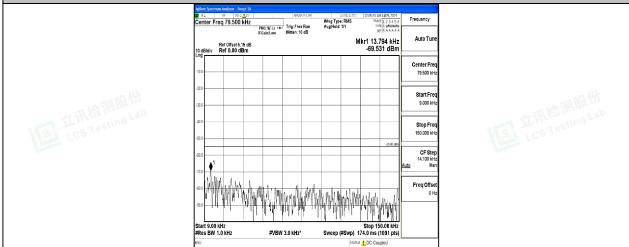
Band7_20MHz_QPSK_21350_1RB#0_0.009~0.15_0.009~0.15
