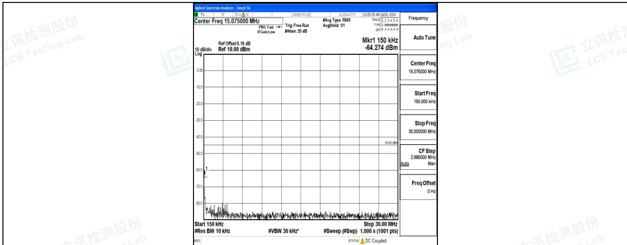
Band7_20MHz_QPSK_21350_1RB#0_0.15~30_0.15~30
