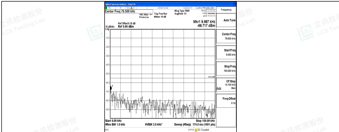
Band7_15MHz_16QAM_21100_1RB#0_0.009~0.15_0.009~0.15
