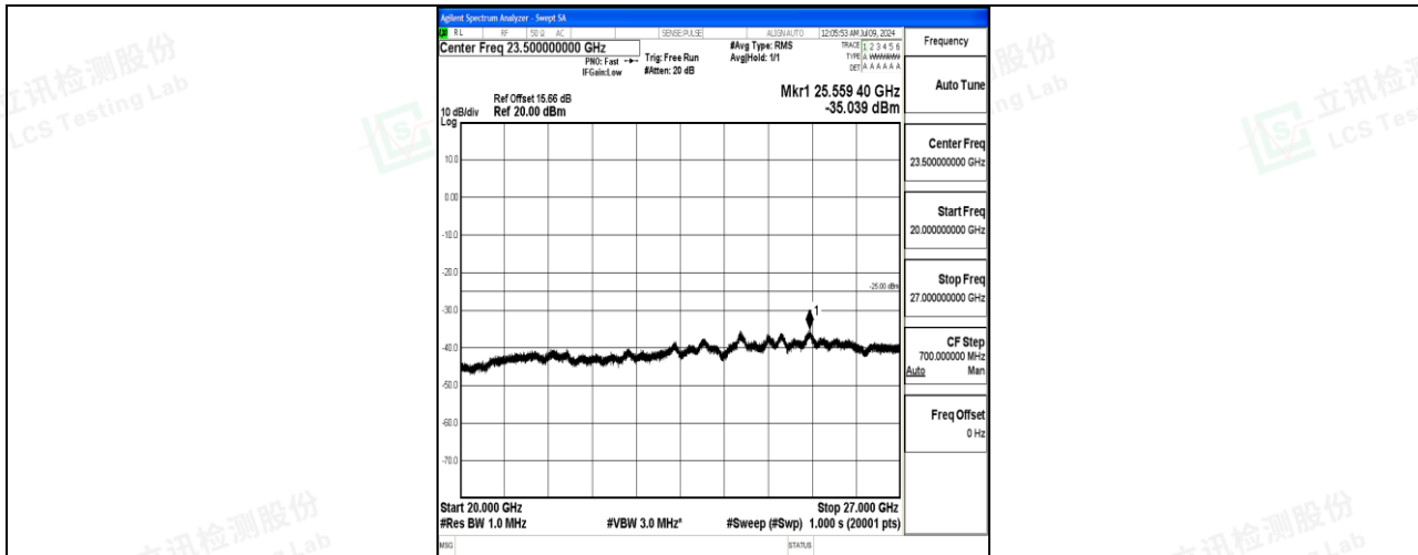
Band7_20MHz_QPSK_21350_1RB#0_20000~27000_20000~27000
