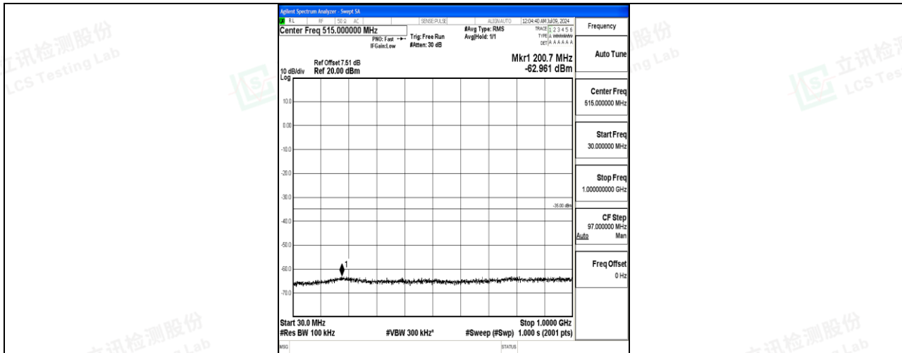
Band7_20MHz_QPSK_21100_1RB#0_30~1000_30~1000
