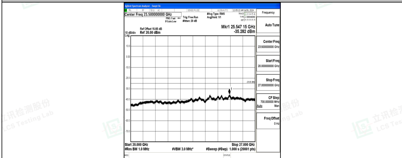
Band7_20MHz_16QAM_21100_1RB#0_20000~27000_20000~27000
