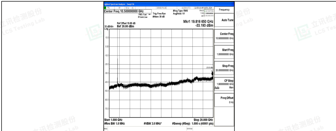
Band7_20MHz_16QAM_21100_1RB#0_1000~20000_1000~20000
