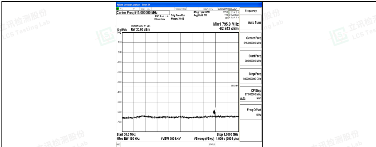
Band7_15MHz_16QAM_21375_1RB#0_30~1000_30~1000
