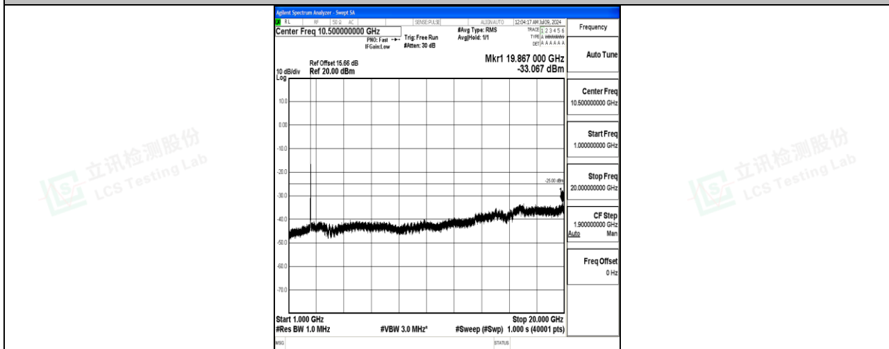
Band7_20MHz_16QAM_20850_1RB#0_1000~20000_1000~20000
