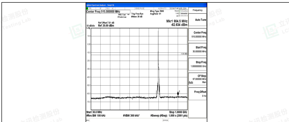
Band17_10MHz_16QAM_23780_1RB#0_30~1000_30~1000
