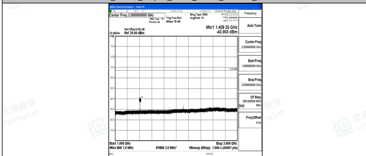
Band17_10MHz_16QAM_23780_1RB#0_1000~3000_1000~3000
