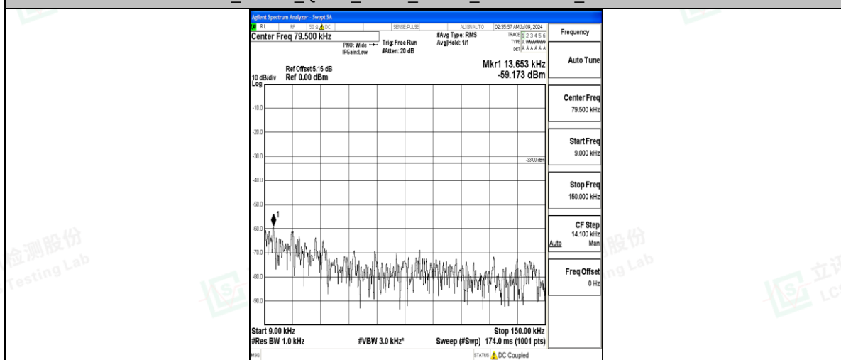
Band17_10MHz_16QAM_23780_1RB#0_0.009~0.15_0.009~0.15
