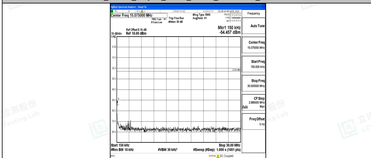
Band17_10MHz_16QAM_23800_1RB#0_0.15~30_0.15~30
