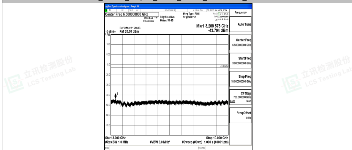
Band17_10MHz_16QAM_23780_1RB#0_3000~10000_3000~10000
