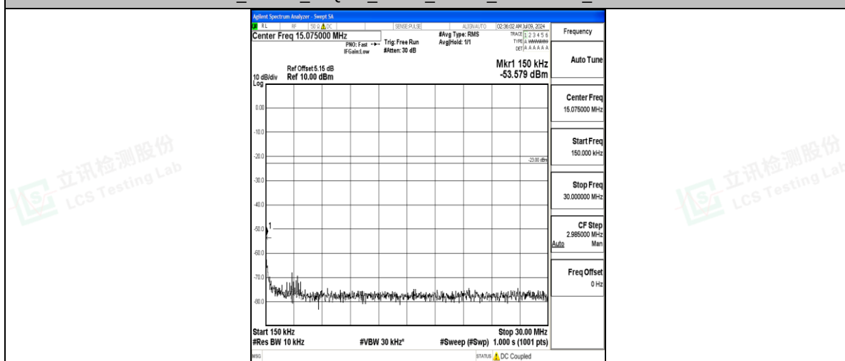
Band17_10MHz_16QAM_23780_1RB#0_0.15~30_0.15~30
