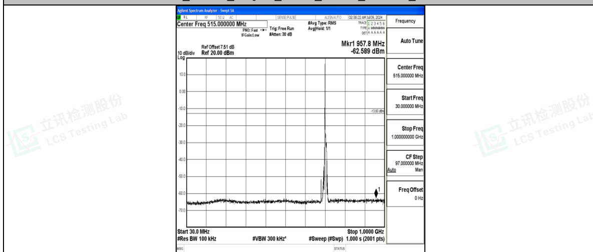
Band17_10MHz_16QAM_23800_1RB#0_30~1000_30~1000
