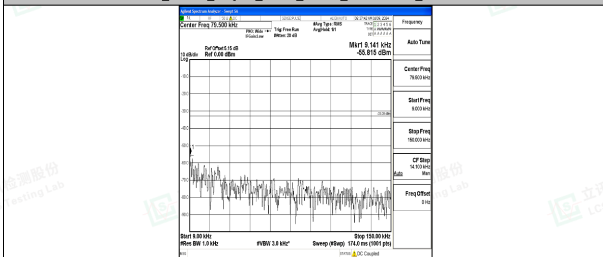
Band17_10MHz_QPSK_23800_1RB#0_0.009~0.15_0.009~0.15
