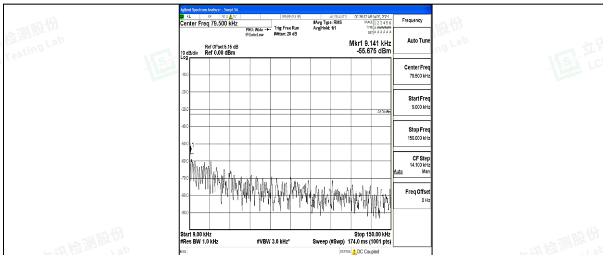
Band17_10MHz_16QAM_23800_1RB#0_0.009~0.15_0.009~0.15
