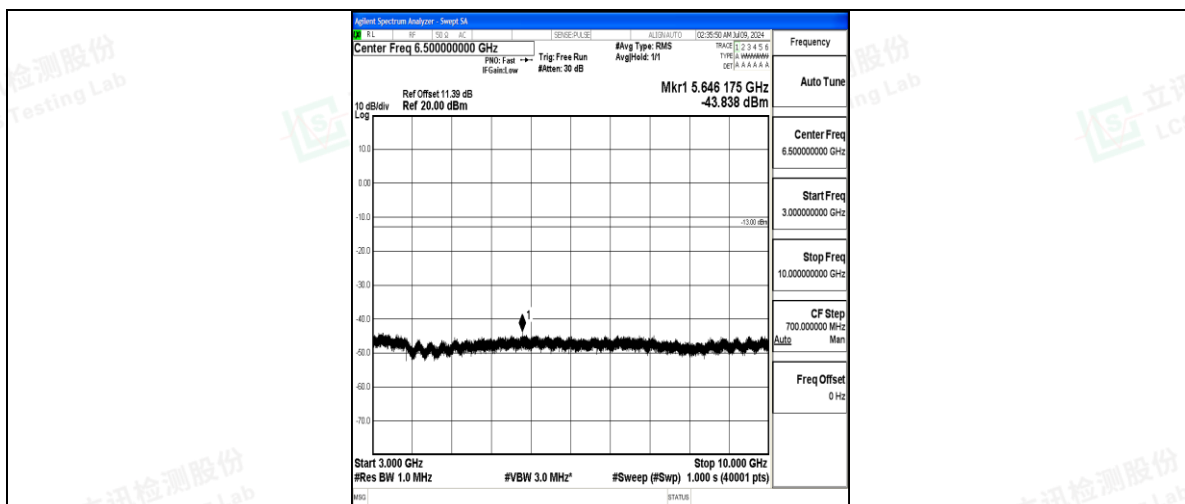
Band17_10MHz_QPSK_23780_1RB#0_3000~10000_3000~10000
