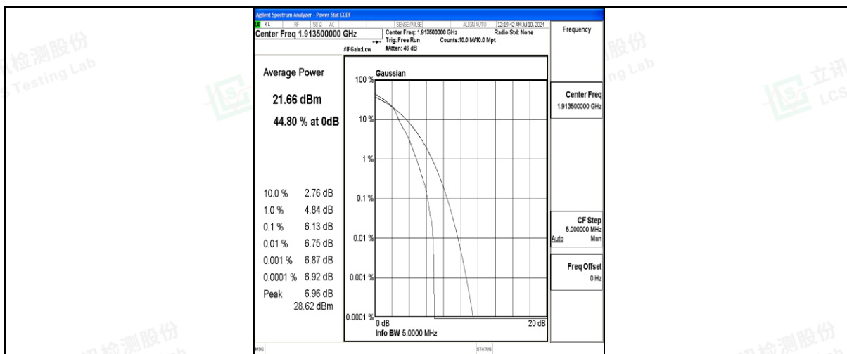
Band25-3MHz-16QAM-26675-1RB#0-PASS
