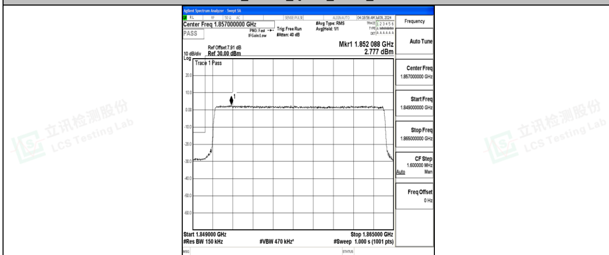
Band25_15MHz_16QAM_26115_75RB#0
