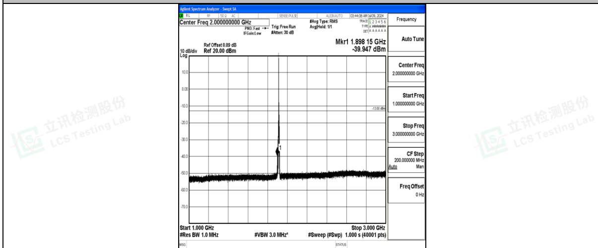
Band25_5MHz_16QAM_26665_1RB#0_1000~3000_1000~3000
