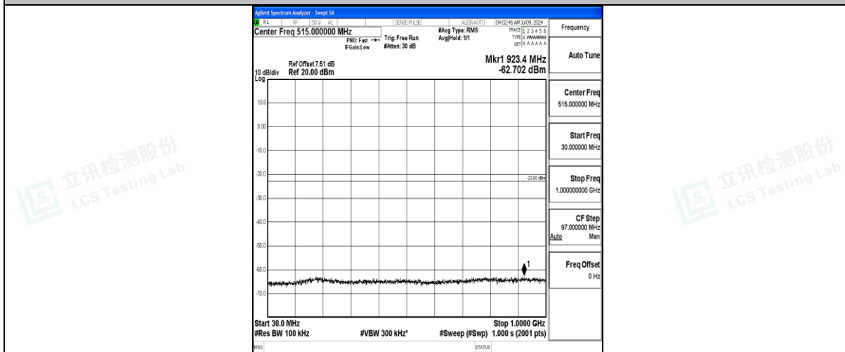
Band25_10MHz_QPSK_26640_1RB#0_30~1000_30~1000
