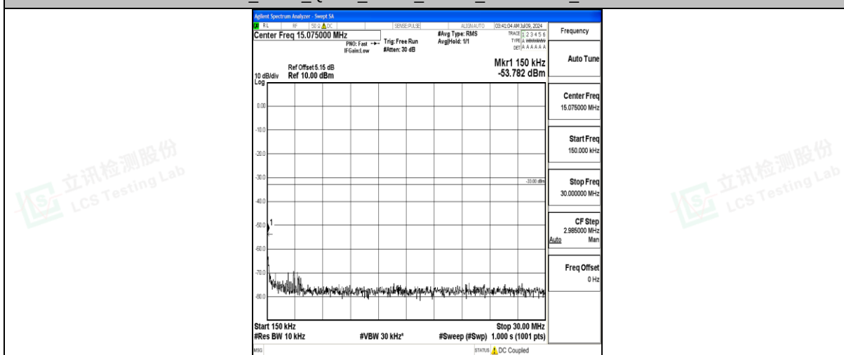
Band25_5MHz_QPSK_26065_1RB#0_0.15~30_0.15~30
