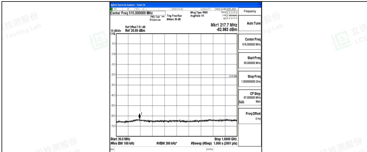
Band25_10MHz_16QAM_26365_1RB#0_30~1000_30~1000
