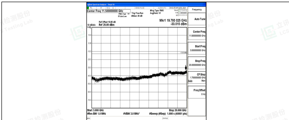
Band25_10MHz_QPSK_26365_1RB#0_3000~20000_3000~20000
