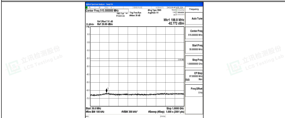
Band25_10MHz_16QAM_26090_1RB#0_30~1000_30~1000
