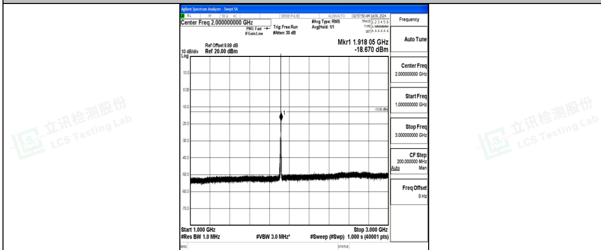
Band25_1.4MHz_16QAM_26683_1RB#0_1000~3000_1000~3000
