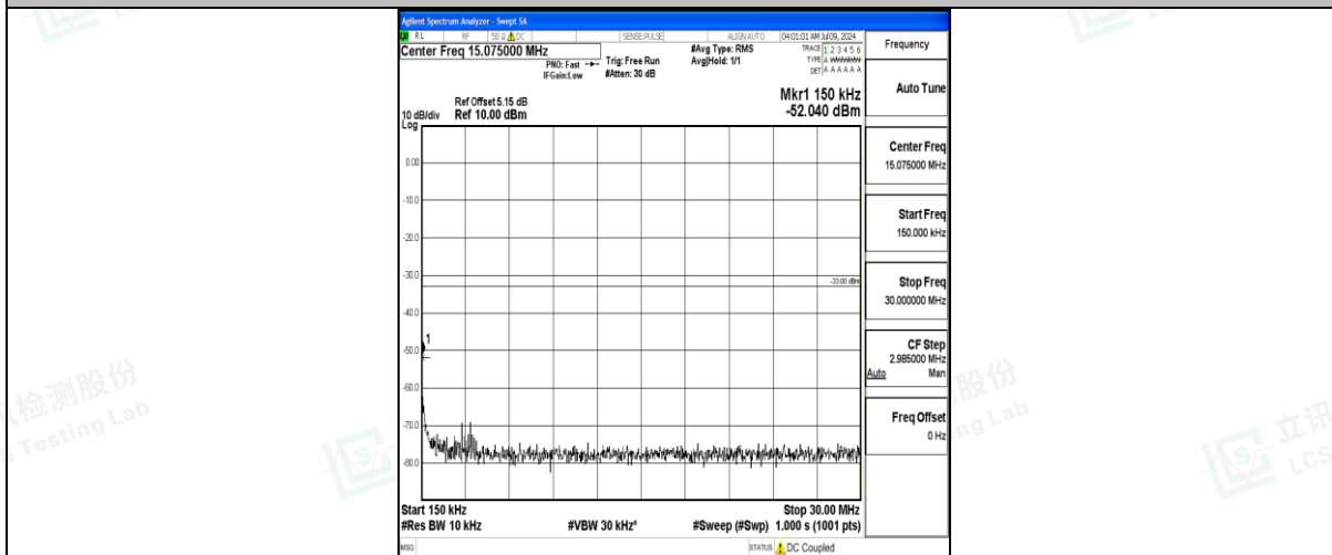
Band25_10MHz_16QAM_26090_1RB#0_0.15~30_0.15~30
