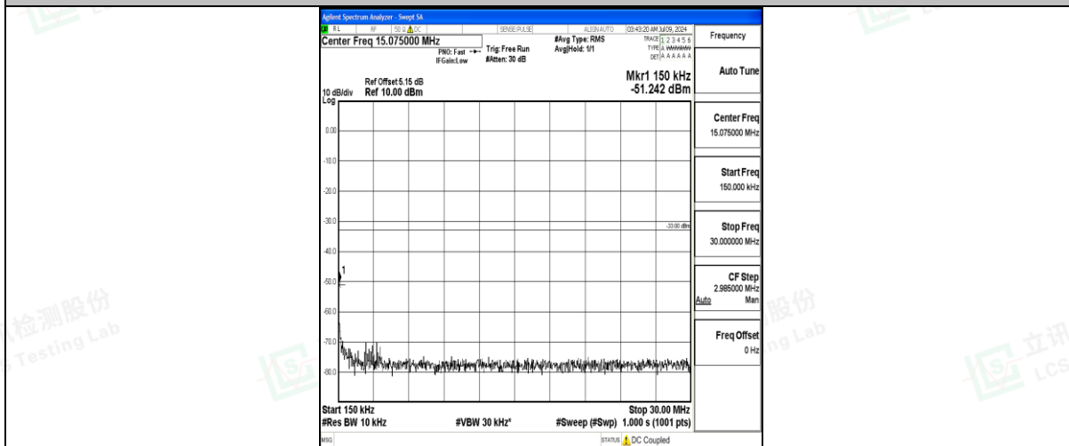
Band25_5MHz_QPSK_26665_1RB#0_0.15~30_0.15~30
