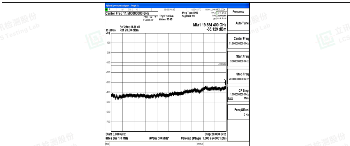
Band25_5MHz_16QAM_26665_1RB#0_3000~20000_3000~20000
