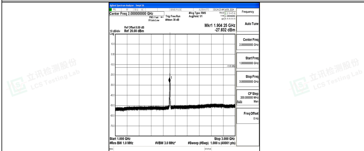
Band25_3MHz_16QAM_26675_1RB#0_1000~3000_1000~3000
