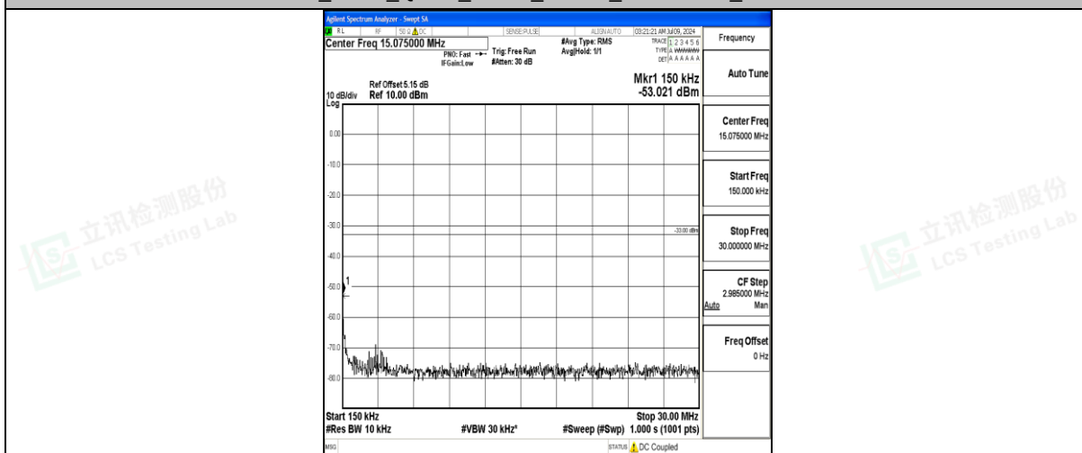
Band25_3MHz_QPSK_26055_1RB#0_0.15~30_0.15~30
