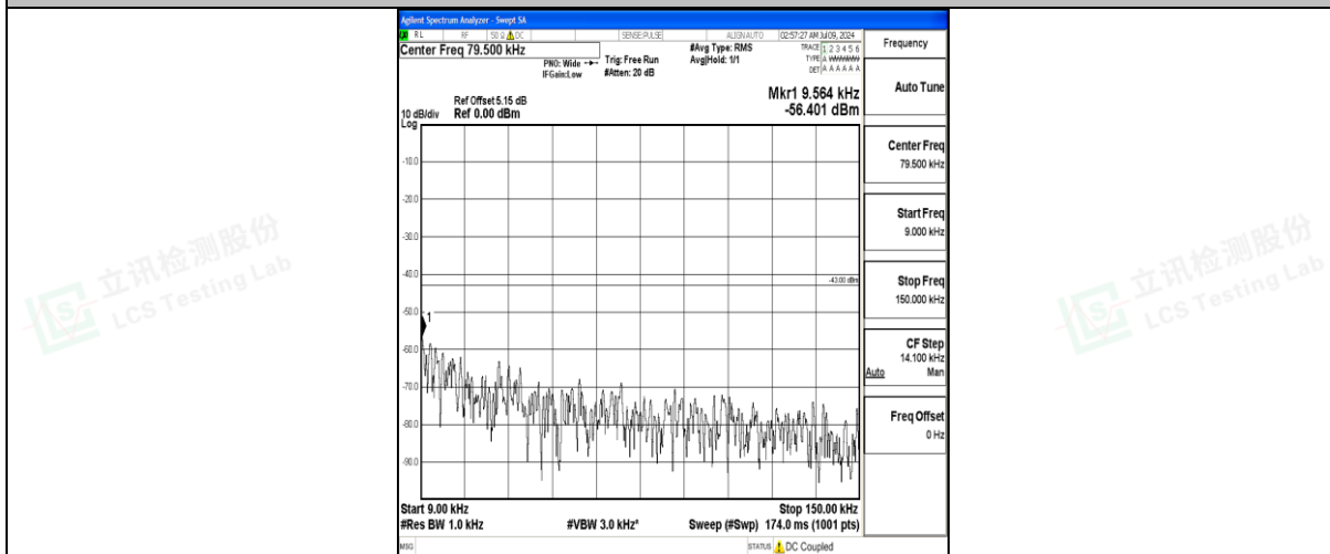
Band25_1.4MHz_16QAM_26683_1RB#0_0.009~0.15_0.009~0.15
