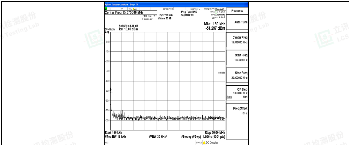
Band25_5MHz_16QAM_26665_1RB#0_0.15~30_0.15~30
