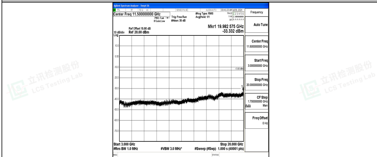
Band25_5MHz_QPSK_26065_1RB#0_3000~20000_3000~20000
