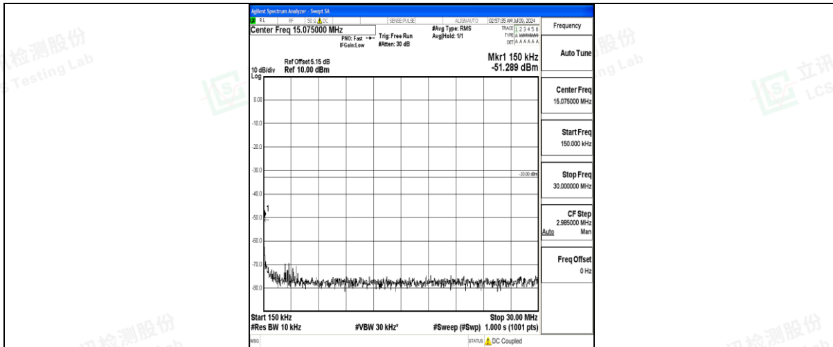
Band25_1.4MHz_16QAM_26683_1RB#0_0.15~30_0.15~30
