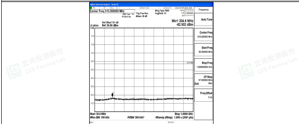
Band25_3MHz_QPSK_26675_1RB#0_30~1000_30~1000
