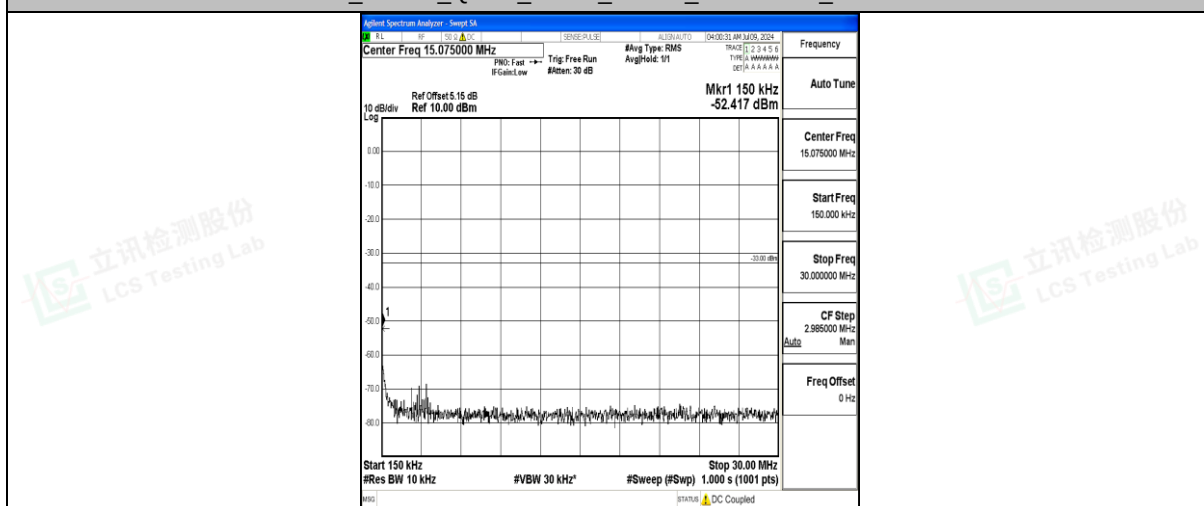
Band25_10MHz_QPSK_26090_1RB#0_0.15~30_0.15~30
