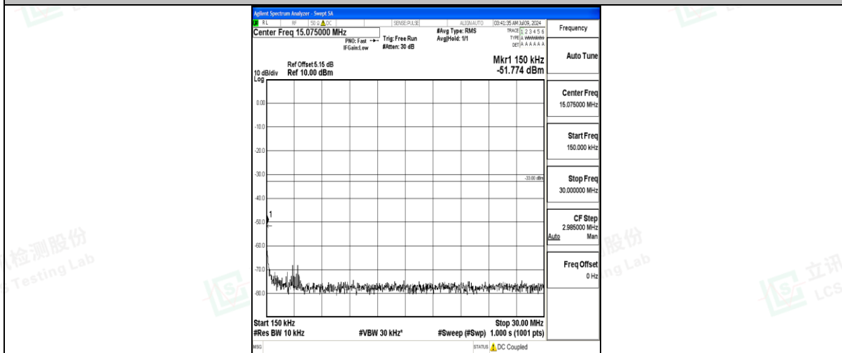
Band25_5MHz_16QAM_26065_1RB#0_0.15~30_0.15~30
