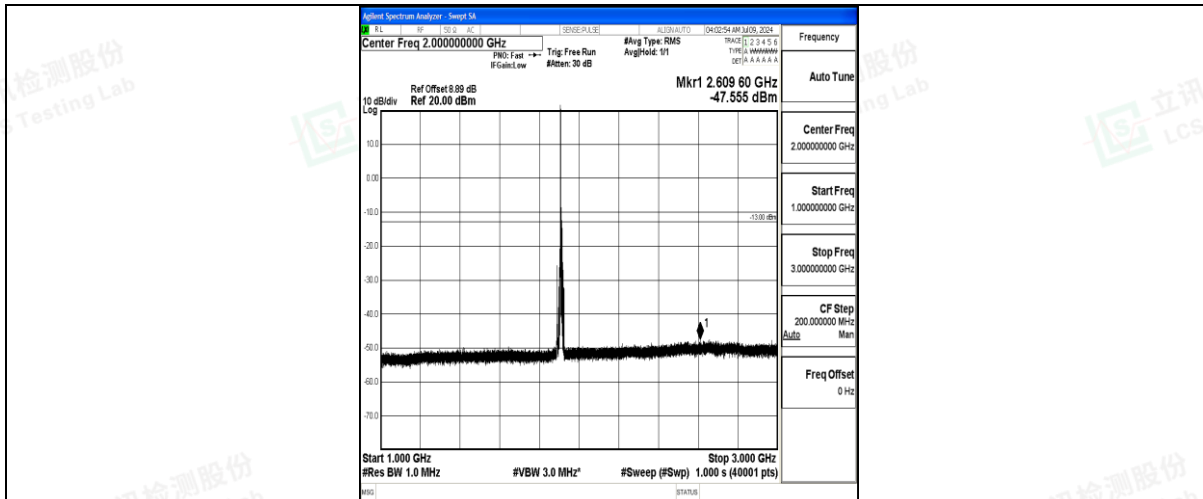
Band25_10MHz_QPSK_26640_1RB#0_1000~3000_1000~3000
