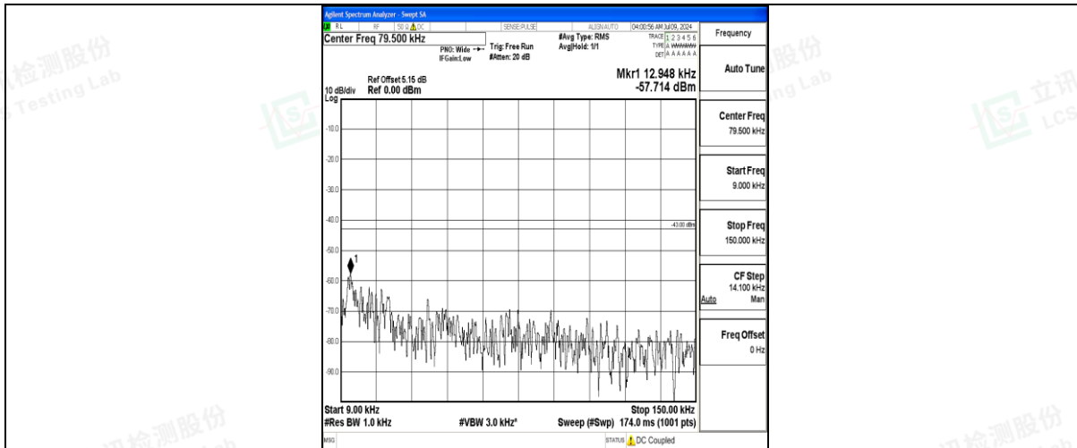
Band25_10MHz_16QAM_26090_1RB#0_0.009~0.15_0.009~0.15
