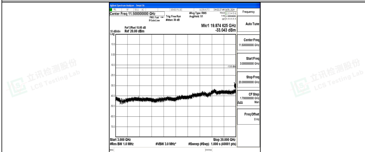
Band25_10MHz_16QAM_26365_1RB#0_3000~20000_3000~20000
