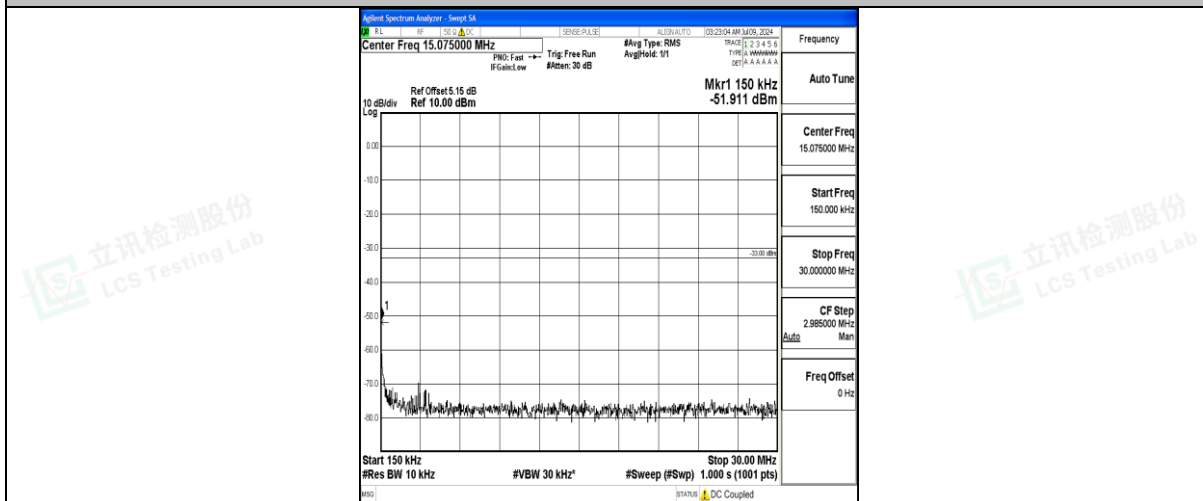
Band25_3MHz_16QAM_26365_1RB#0_0.15~30_0.15~30
