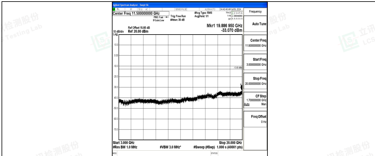
Band25_20MHz_QPSK_26365_1RB#0_3000~20000_3000~20000
