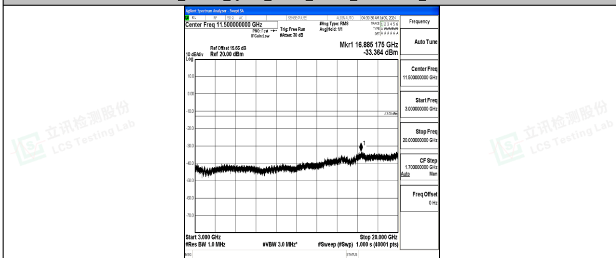
Band25_20MHz_QPSK_26140_1RB#0_3000~20000_3000~20000
