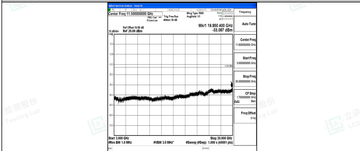
Band25_20MHz_16QAM_26140_1RB#0_3000~20000_3000~20000
