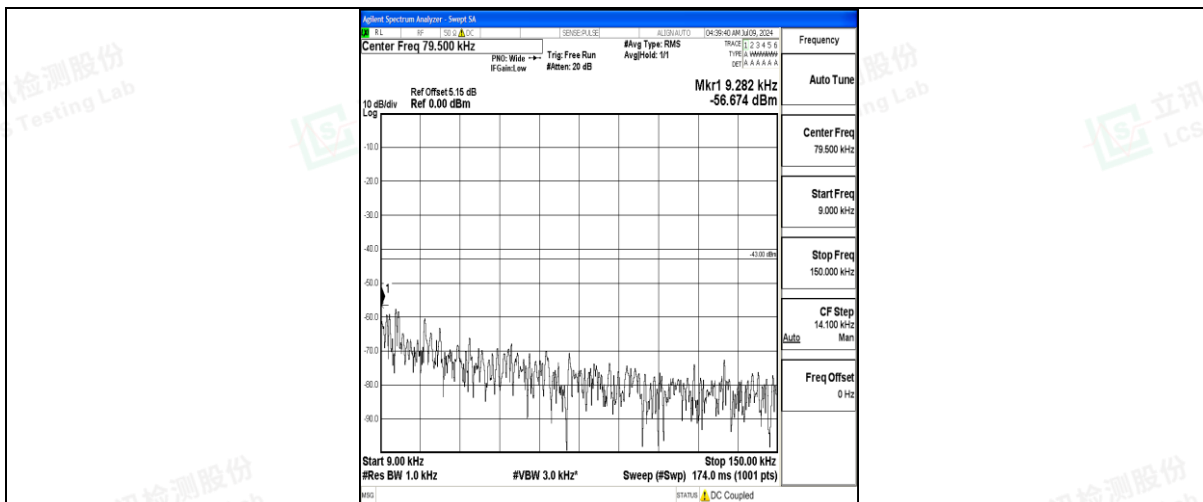
Band25_20MHz_16QAM_26140_1RB#0_0.009~0.15_0.009~0.15
