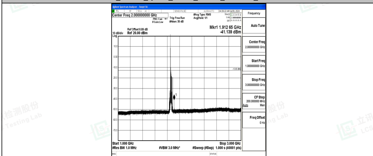
Band25_20MHz_QPSK_26140_1RB#0_1000~3000_1000~3000
