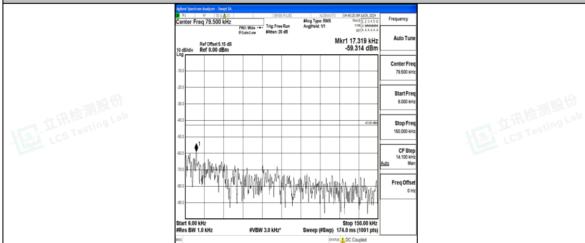
Band25_20MHz_QPSK_26365_1RB#0_0.009~0.15_0.009~0.15
