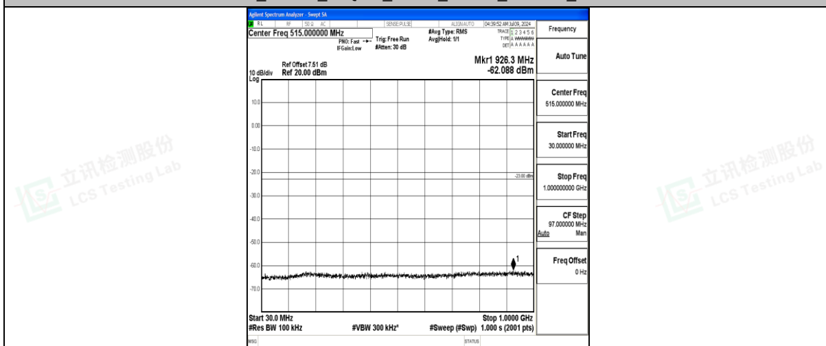
Band25_20MHz_16QAM_26140_1RB#0_30~1000_30~1000
