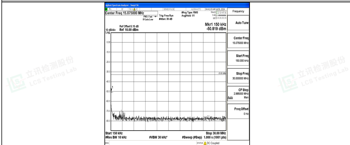
Band25_20MHz_16QAM_26365_1RB#0_0.15~30_0.15~30
