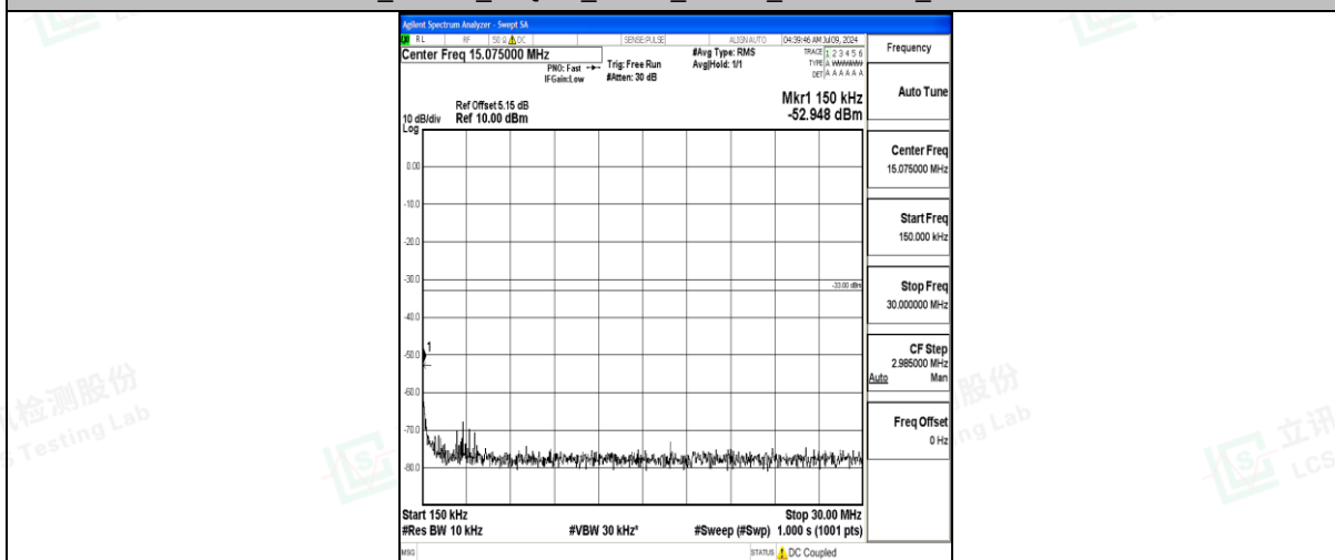
Band25_20MHz_16QAM_26140_1RB#0_0.15~30_0.15~30
