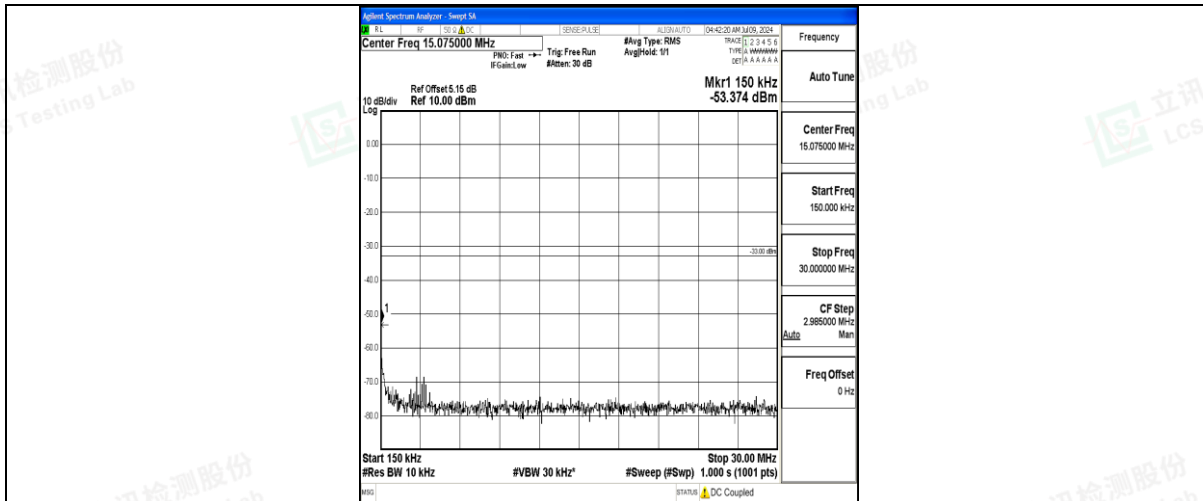
Band25_20MHz_16QAM_26590_1RB#0_0.15~30_0.15~30
