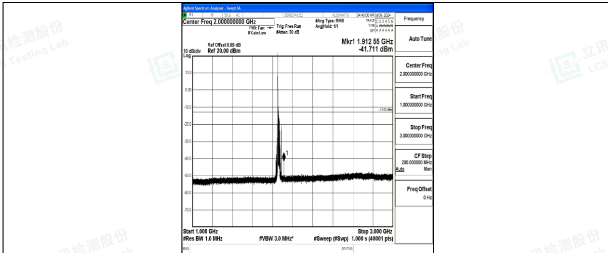
Band25_20MHz_16QAM_26140_1RB#0_1000~3000_1000~3000
