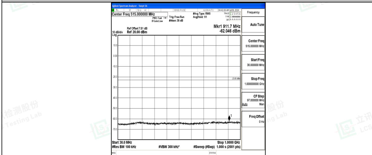
Band25_20MHz_16QAM_26590_1RB#0_30~1000_30~1000
