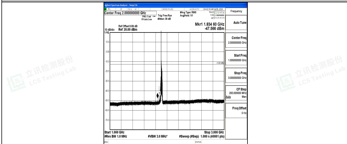
Band25_20MHz_16QAM_26590_1RB#0_1000~3000_1000~3000
