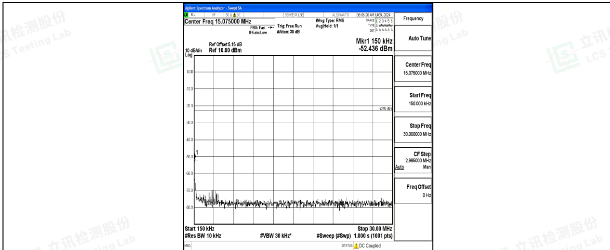
Band26_10MHz_QPSK_26740_1RB#0_0.15~30_0.15~30
