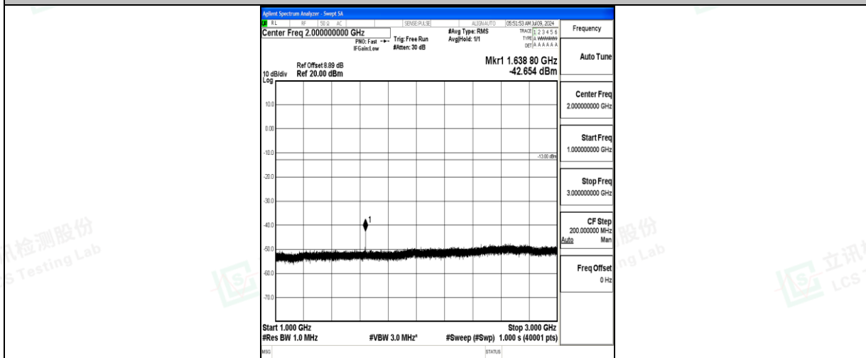
Band26_5MHz_QPSK_26765_1RB#0_1000~3000_1000~3000
