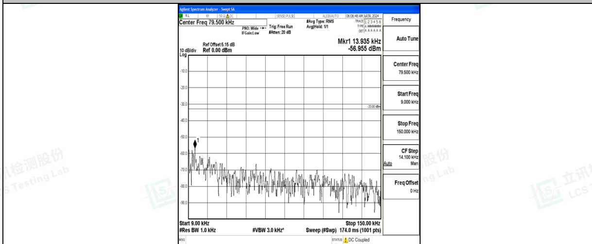
Band26_10MHz_16QAM_26740_1RB#0_0.009~0.15_0.009~0.15
