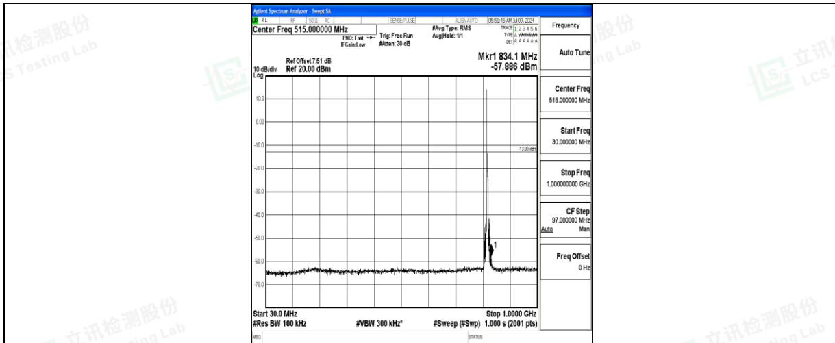
Band26_5MHz_QPSK_26765_1RB#0_30~1000_30~1000
