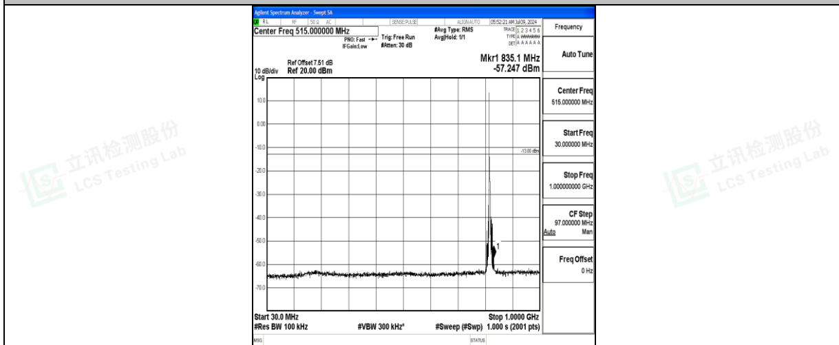
Band26_5MHz_16QAM_26765_1RB#0_30~1000_30~1000
