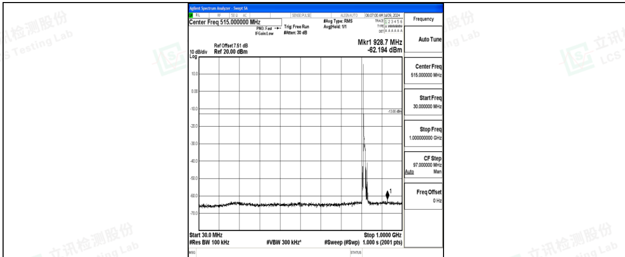
Band26_10MHz_16QAM_26740_1RB#0_30~1000_30~1000
