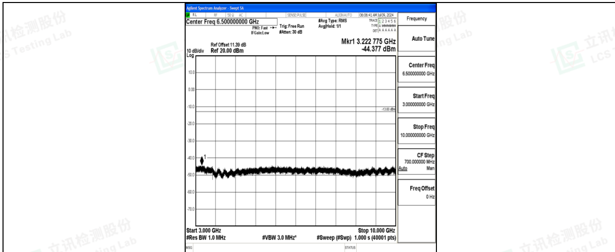
Band26_10MHz_QPSK_26740_1RB#0_3000~10000_3000~10000
