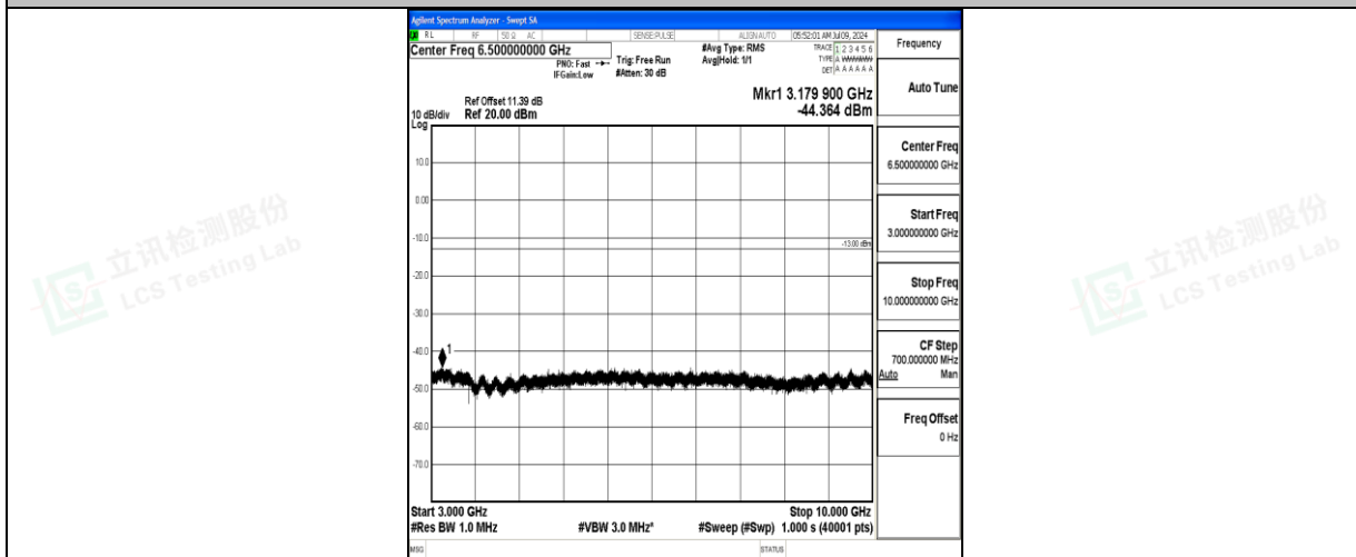
Band26_5MHz_QPSK_26765_1RB#0_3000~10000_3000~10000
