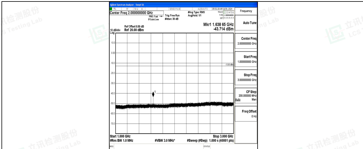
Band26_5MHz_16QAM_26765_1RB#0_1000~3000_1000~3000
