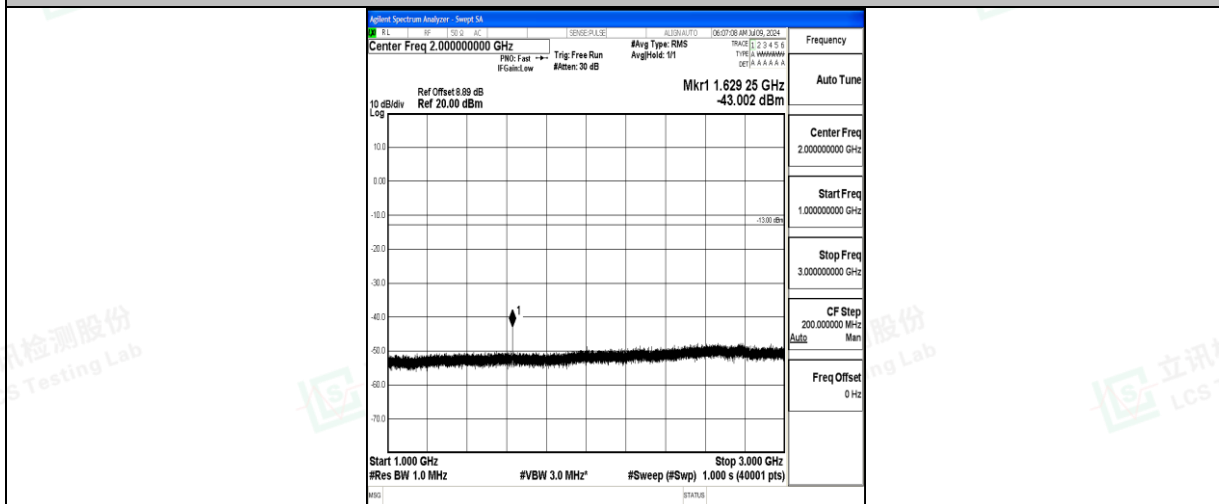
Band26_10MHz_16QAM_26740_1RB#0_1000~3000_1000~3000
