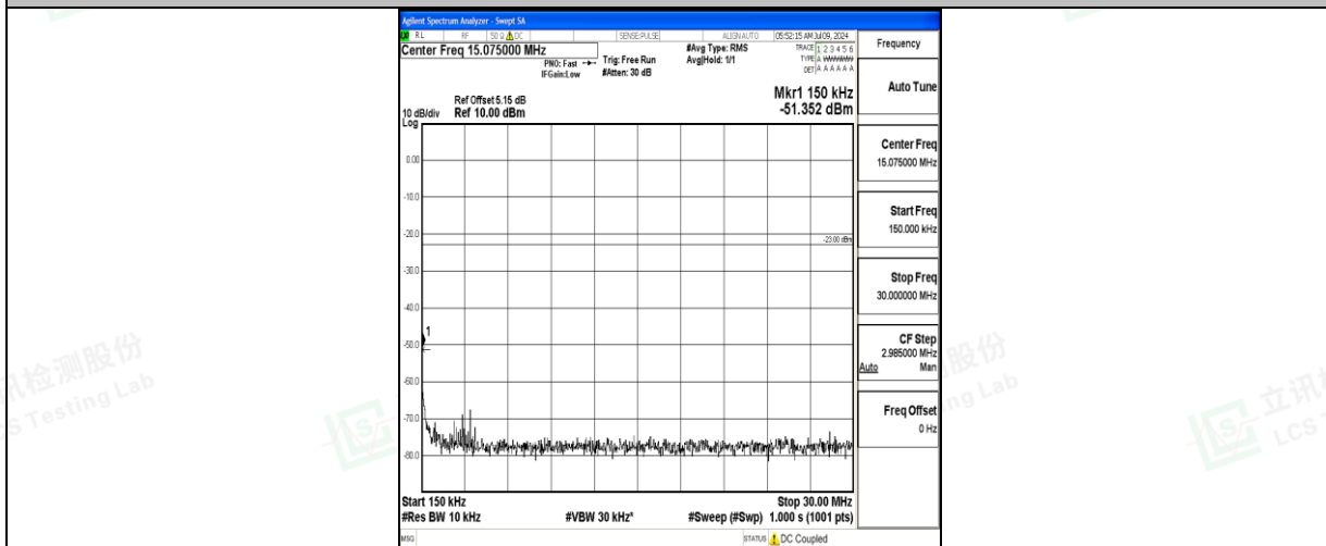
Band26_5MHz_16QAM_26765_1RB#0_0.15~30_0.15~30
