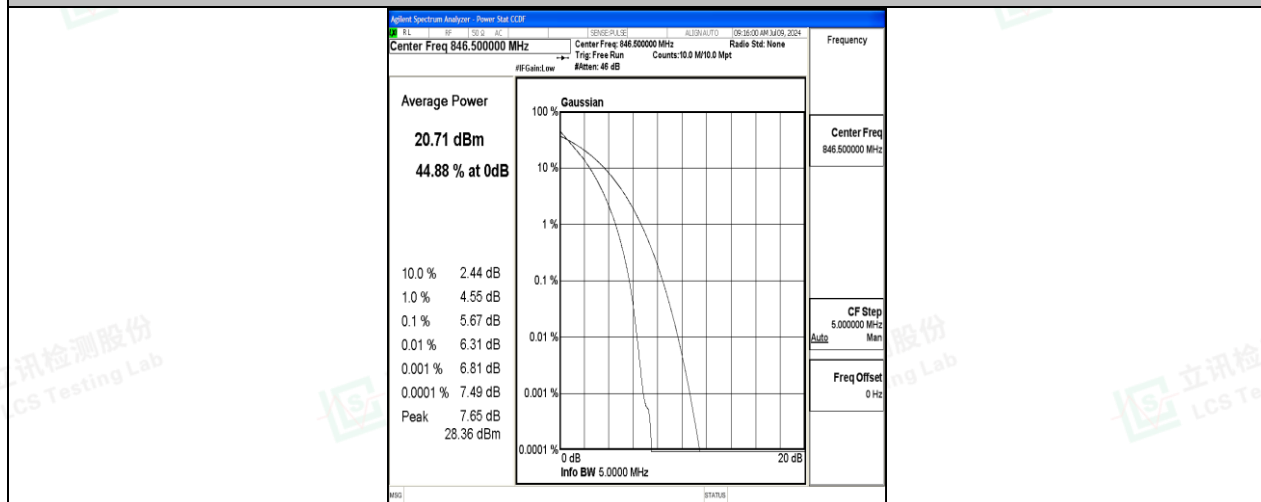
26(824-849)-5MHz-QPSK-27015-25RB#0-PASS
