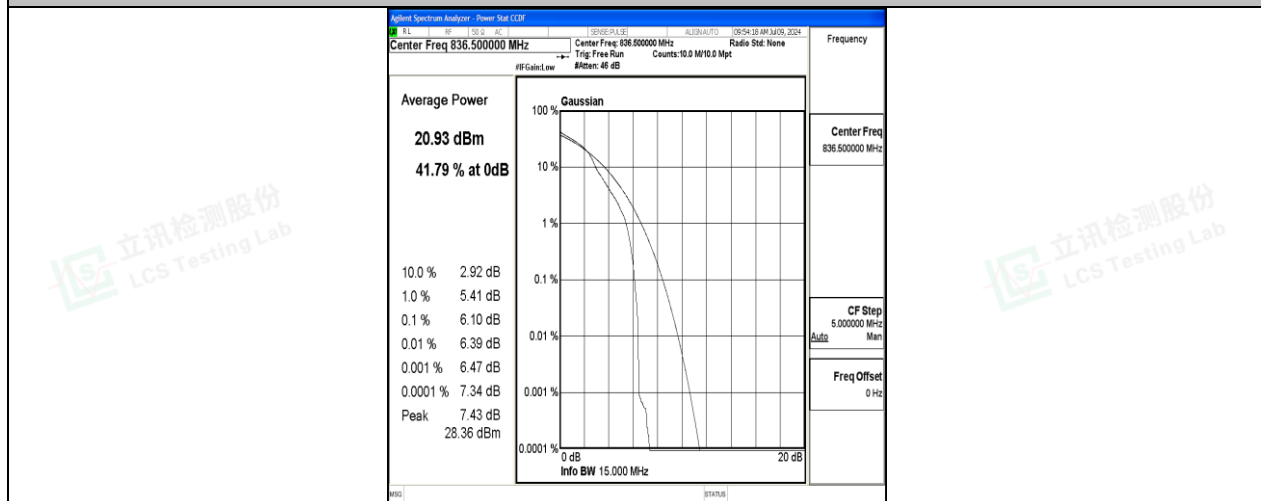
26(824-849)-15MHz-16QAM-26915-1RB#0-PASS
