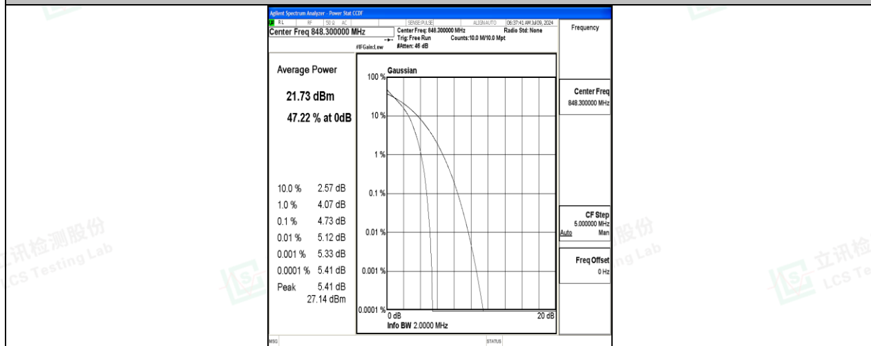
26(824-849)-1.4MHz-QPSK-27033-6RB#0-PASS
