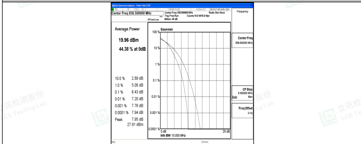
26(824-849)-10MHz-16QAM-26915-50RB#0-PASS
