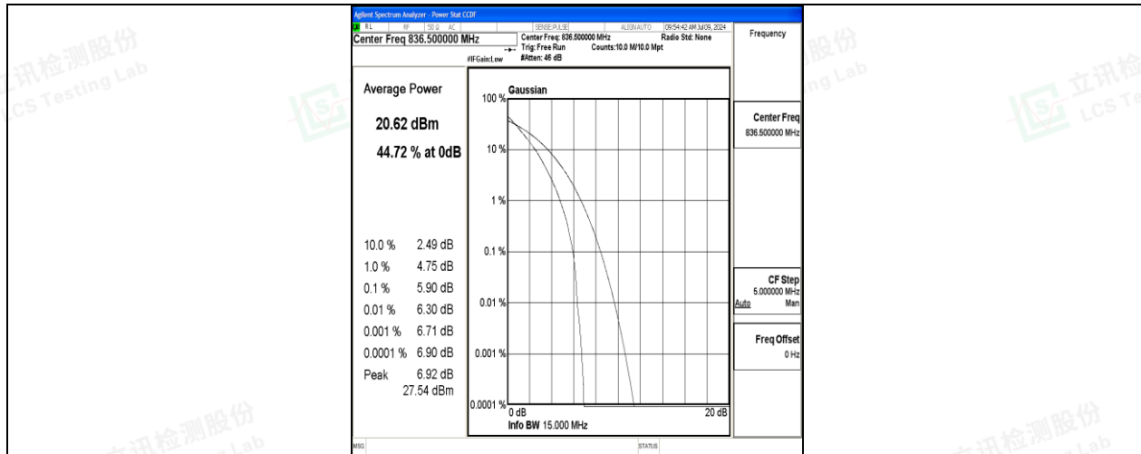
26(824-849)-15MHz-QPSK-26915-75RB#0-PASS
