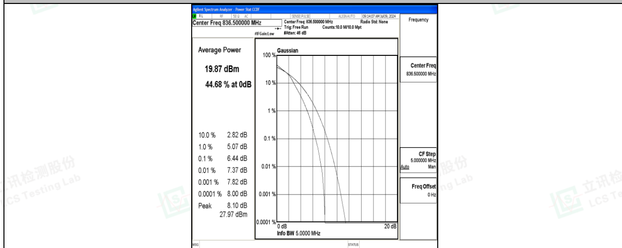
26(824-849)-5MHz-16QAM-26915-25RB#0-PASS
