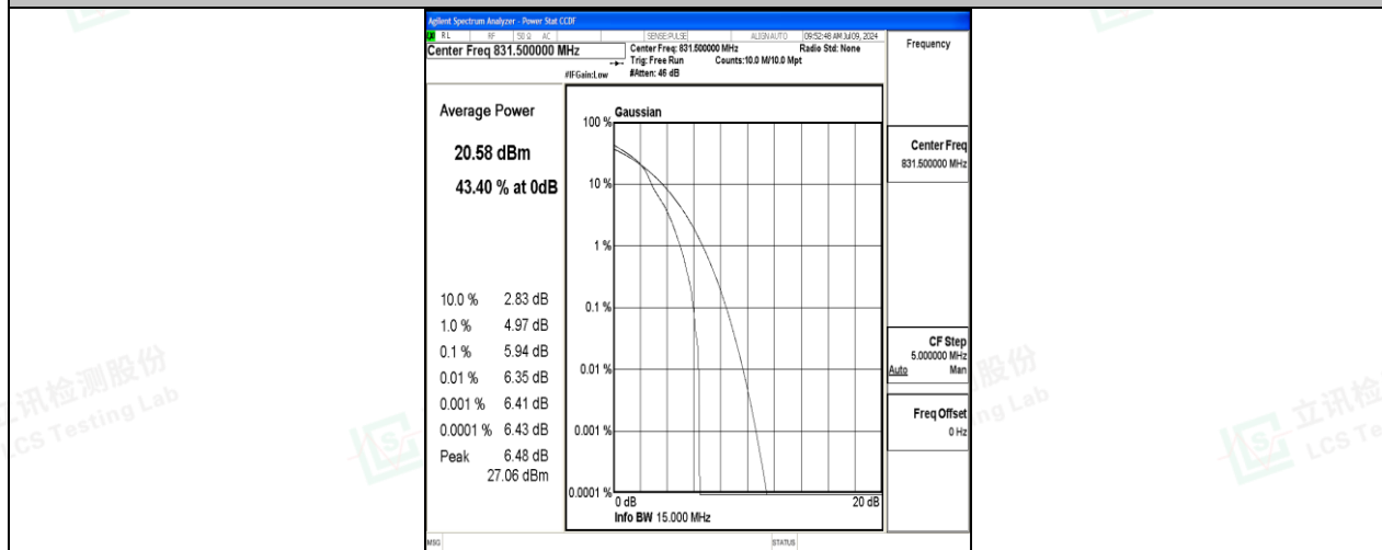
26(824-849)-15MHz-16QAM-26865-1RB#0-PASS
