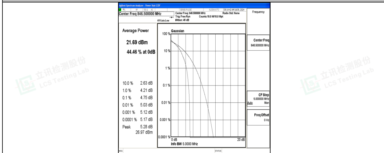
26(824-849)-5MHz-QPSK-27015-1RB#0-PASS
