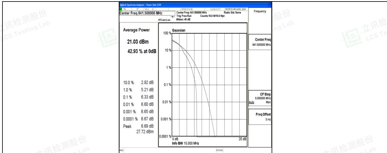
26(824-849)-15MHz-16QAM-26965-1RB#0-PASS
