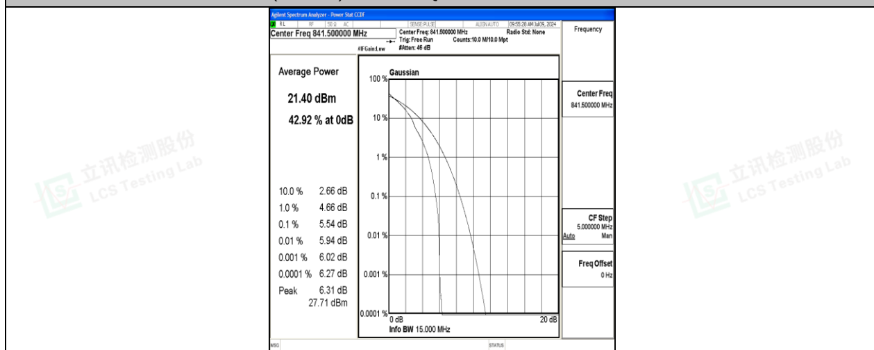
26(824-849)-15MHz-QPSK-26965-1RB#0-PASS
