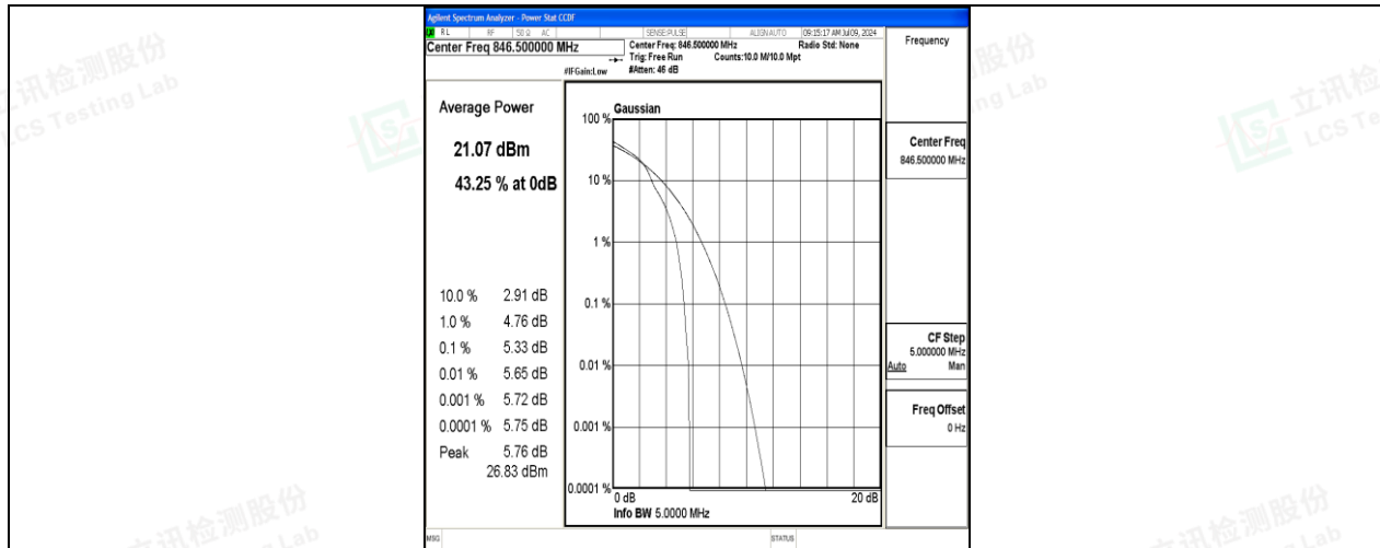
26(824-849)-5MHz-16QAM-27015-1RB#0-PASS
