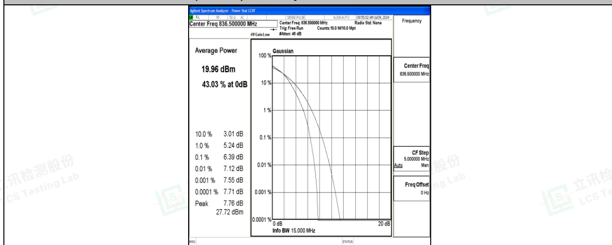
26(824-849)-15MHz-16QAM-26915-75RB#0-PASS
