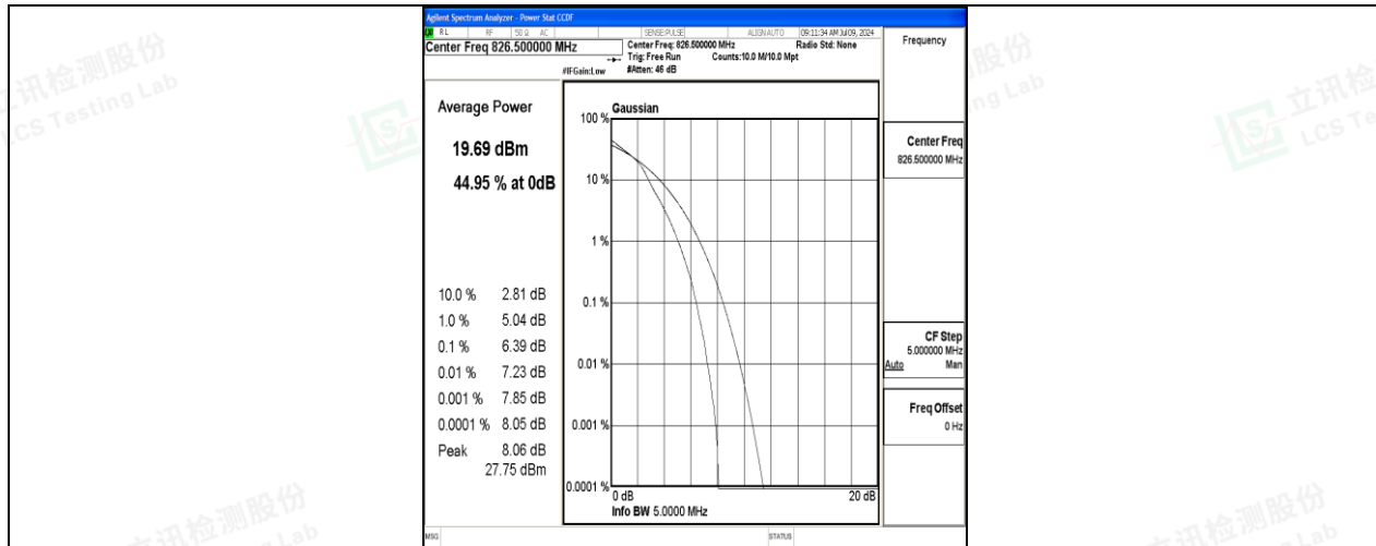
26(824-849)-5MHz-16QAM-26815-25RB#0-PASS
