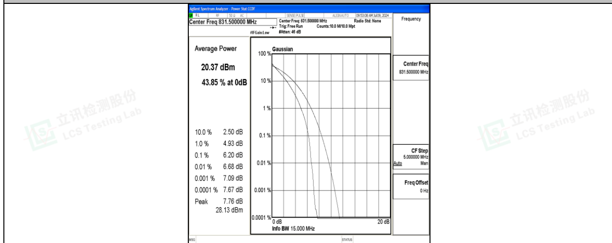
26(824-849)-15MHz-QPSK-26865-75RB#0-PASS
