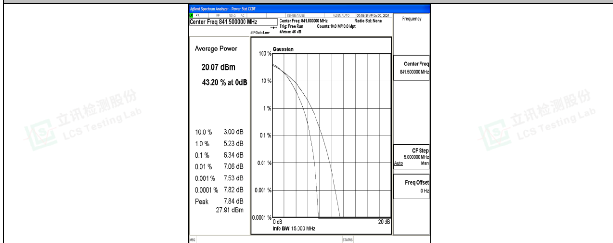
26(824-849)-15MHz-16QAM-26965-75RB#0-PASS
