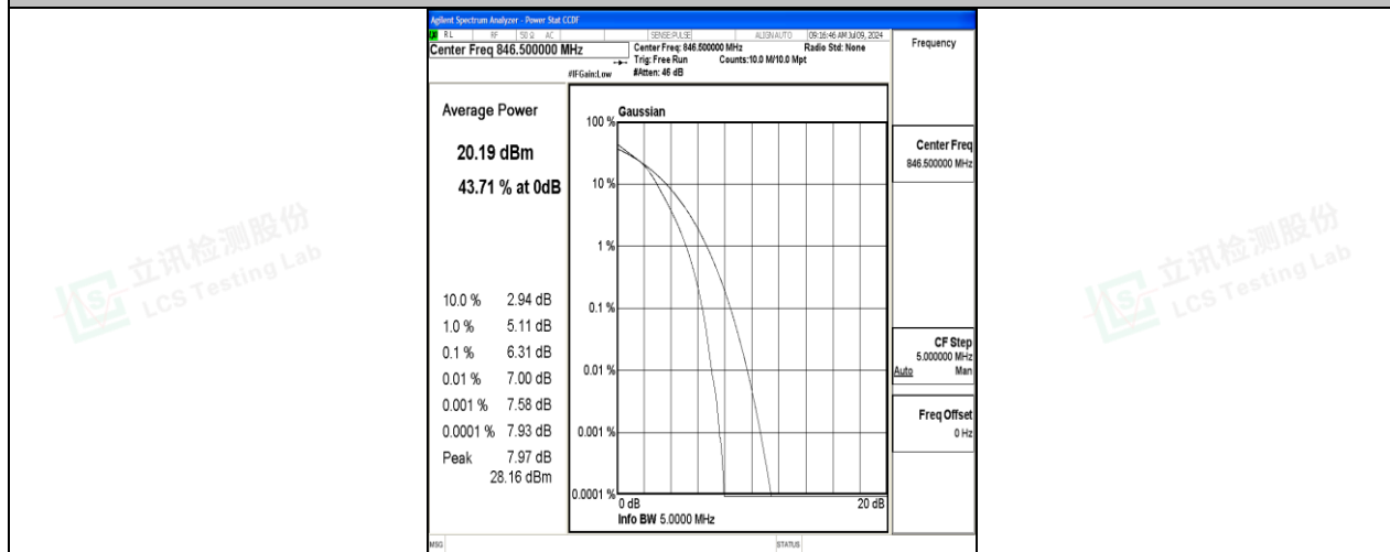
26(824-849)-5MHz-16QAM-27015-25RB#0-PASS
