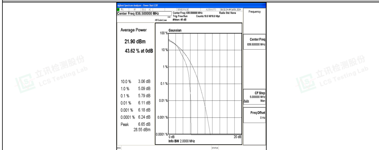
26(824-849)-1.4MHz-16QAM-26915-1RB#0-PASS
