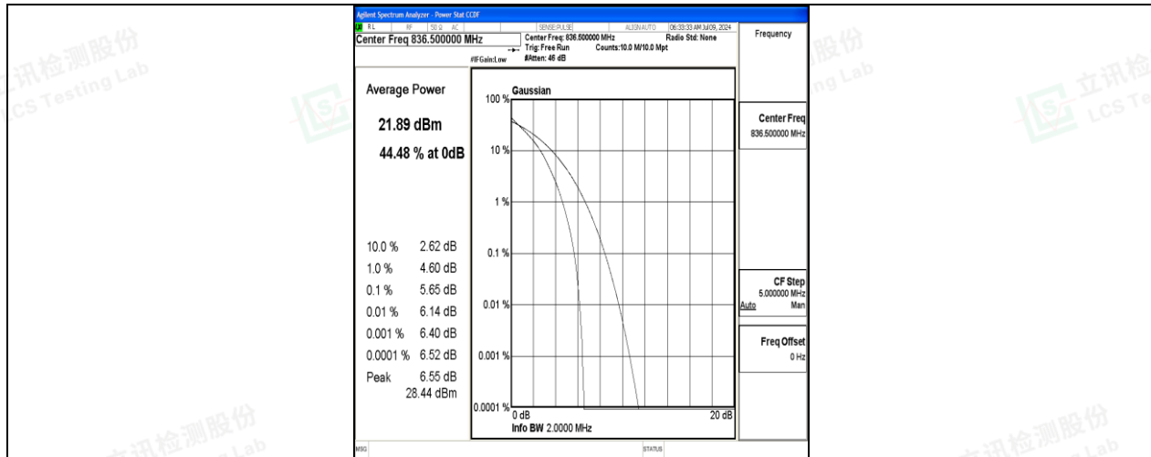
26(824-849)-1.4MHz-QPSK-26915-6RB#0-PASS
