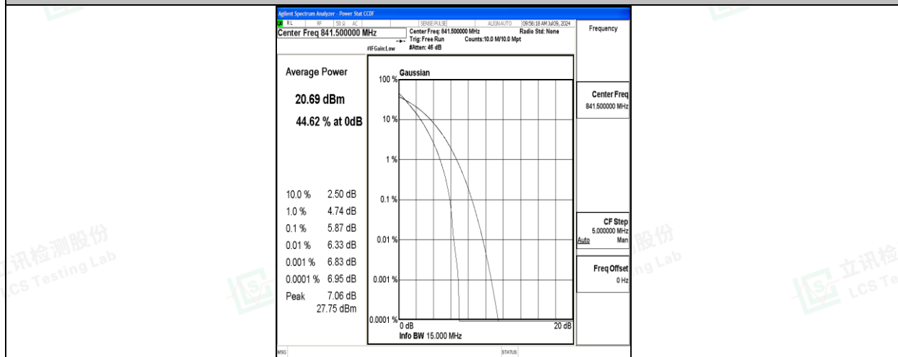
26(824-849)-15MHz-QPSK-26965-75RB#0-PASS
