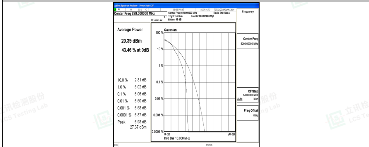
26(824-849)-10MHz-16QAM-26840-1RB#0-PASS
