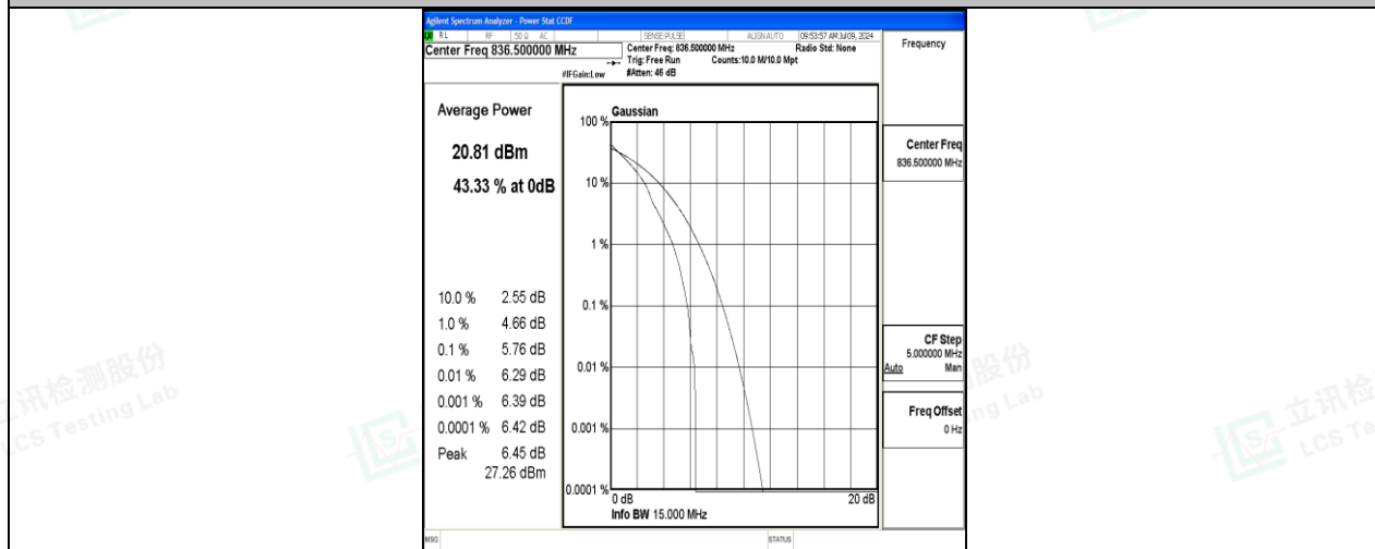
26(824-849)-15MHz-QPSK-26915-1RB#0-PASS
