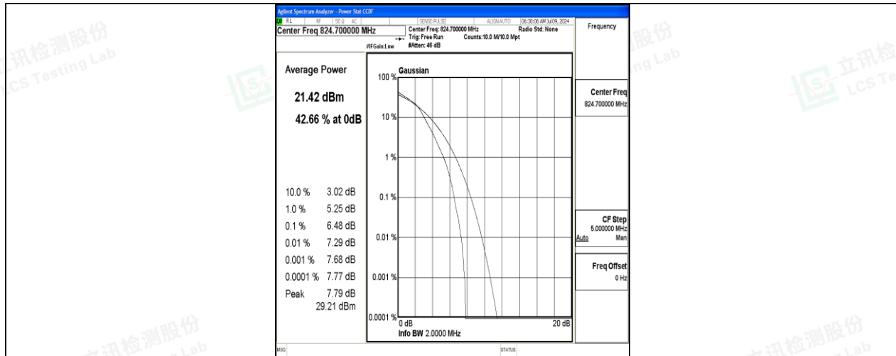
26(824-849)-1.4MHz-16QAM-26797-6RB#0-PASS
