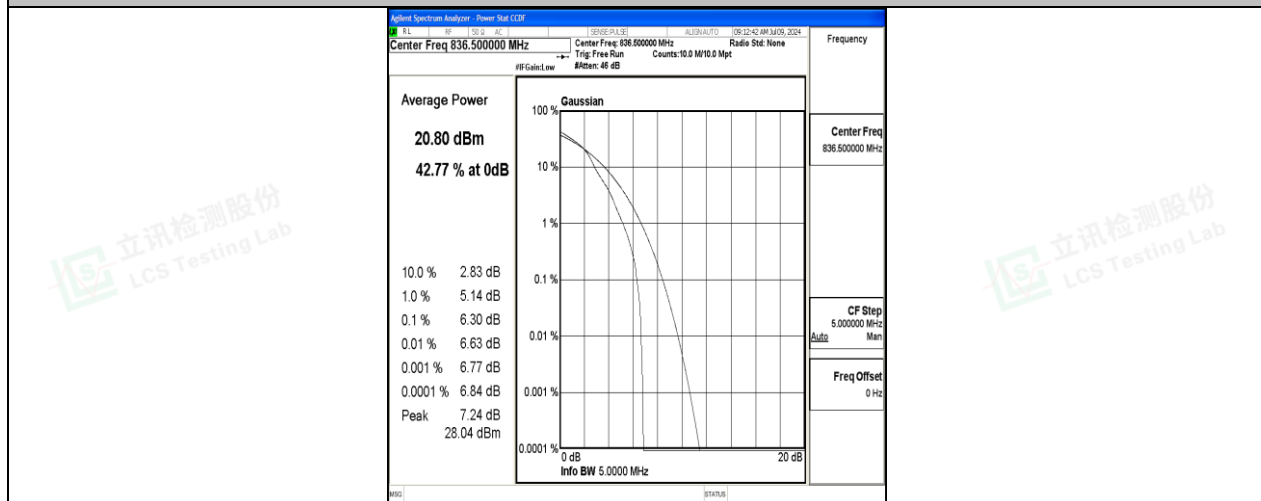
26(824-849)-5MHz-16QAM-26915-1RB#0-PASS
