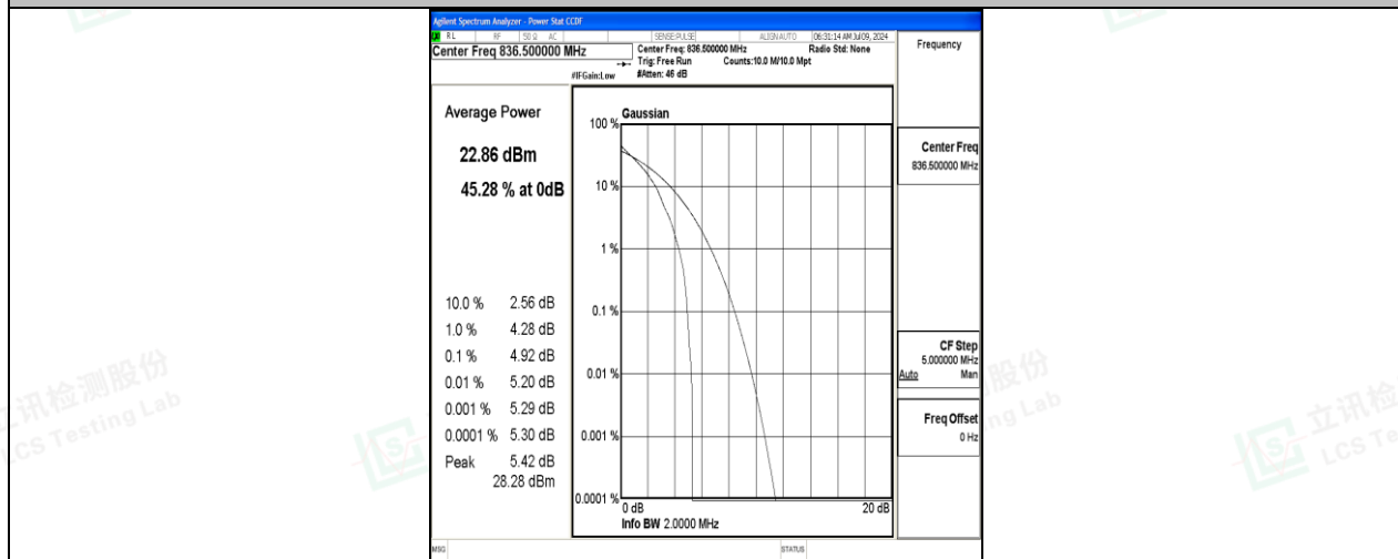
26(824-849)-1.4MHz-QPSK-26915-1RB#0-PASS
