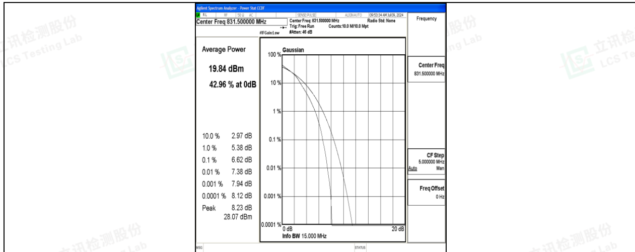
26(824-849)-15MHz-16QAM-26865-75RB#0-PASS
