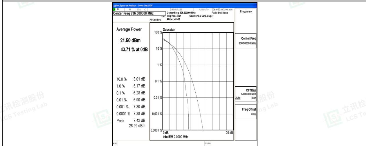
26(824-849)-1.4MHz-16QAM-26915-6RB#0-PASS
