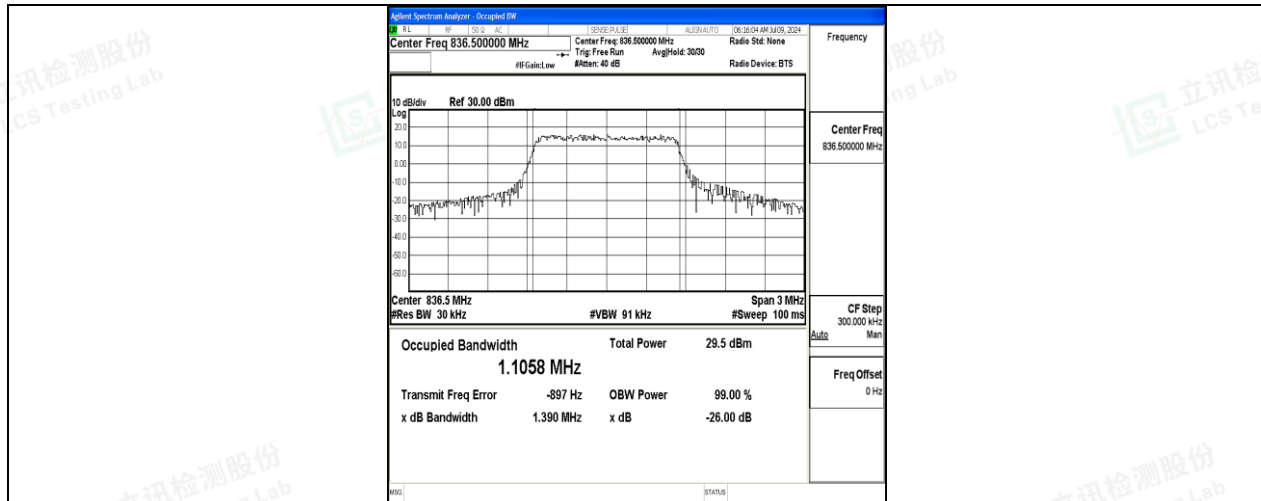
26(824-849)-1.4MHz-16QAM-26915-6RB#0-PASS
