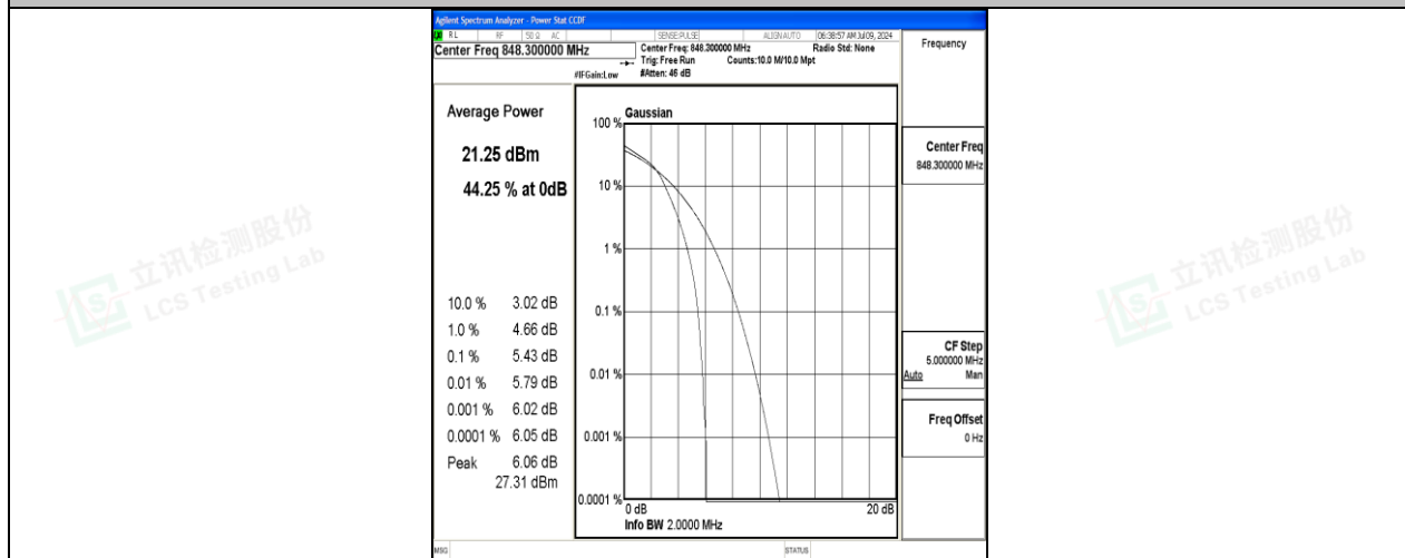
26(824-849)-1.4MHz-16QAM-27033-6RB#0-PASS
