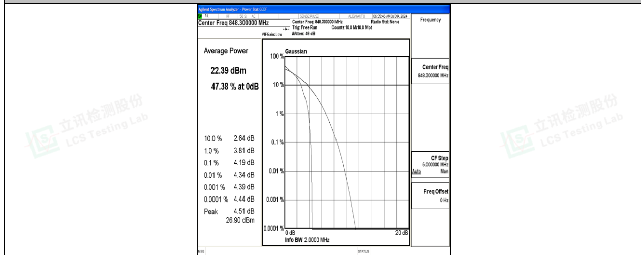
26(824-849)-1.4MHz-QPSK-27033-1RB#0-PASS
