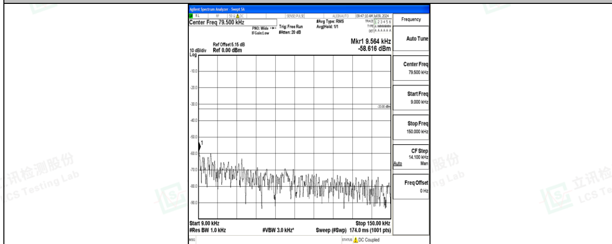
Band26_15MHz_16QAM_26965_1RB#0_0.009~0.15_0.009~0.15
