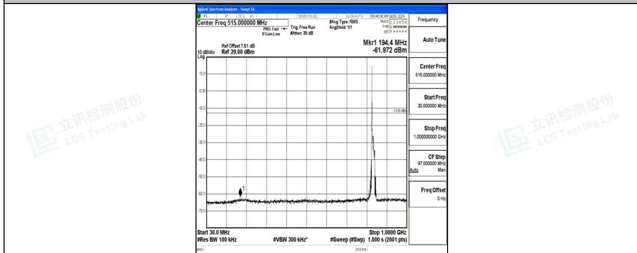
Band26_15MHz_16QAM_26915_1RB#0_30~1000_30~1000
