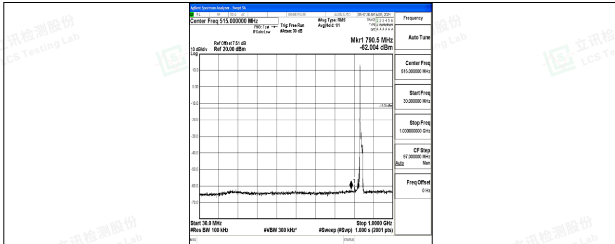
Band26_15MHz_16QAM_26965_1RB#0_30~1000_30~1000
