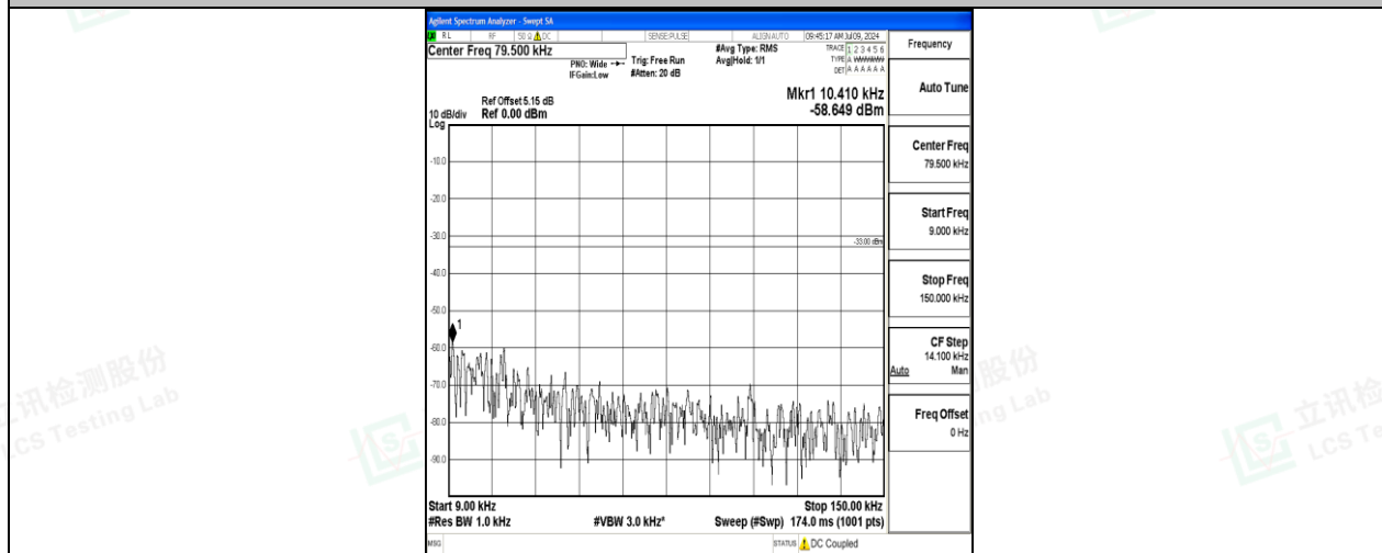
Band26_15MHz_QPSK_26915_1RB#0_0.009~0.15_0.009~0.15
