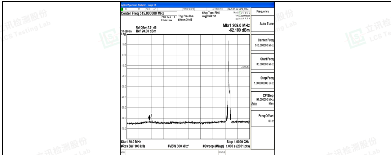
Band26_15MHz_QPSK_26915_1RB#0_30~1000_30~1000
