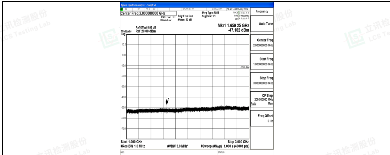
Band26_15MHz_16QAM_26915_1RB#0_1000~3000_1000~3000
