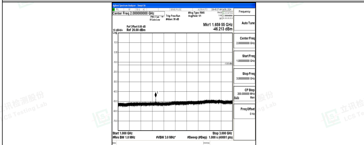
Band26_15MHz_QPSK_26915_1RB#0_1000~3000_1000~3000
