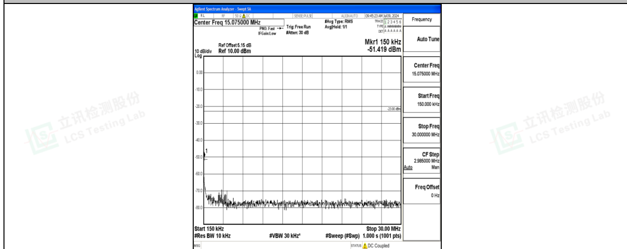
Band26_15MHz_QPSK_26915_1RB#0_0.15~30_0.15~30
