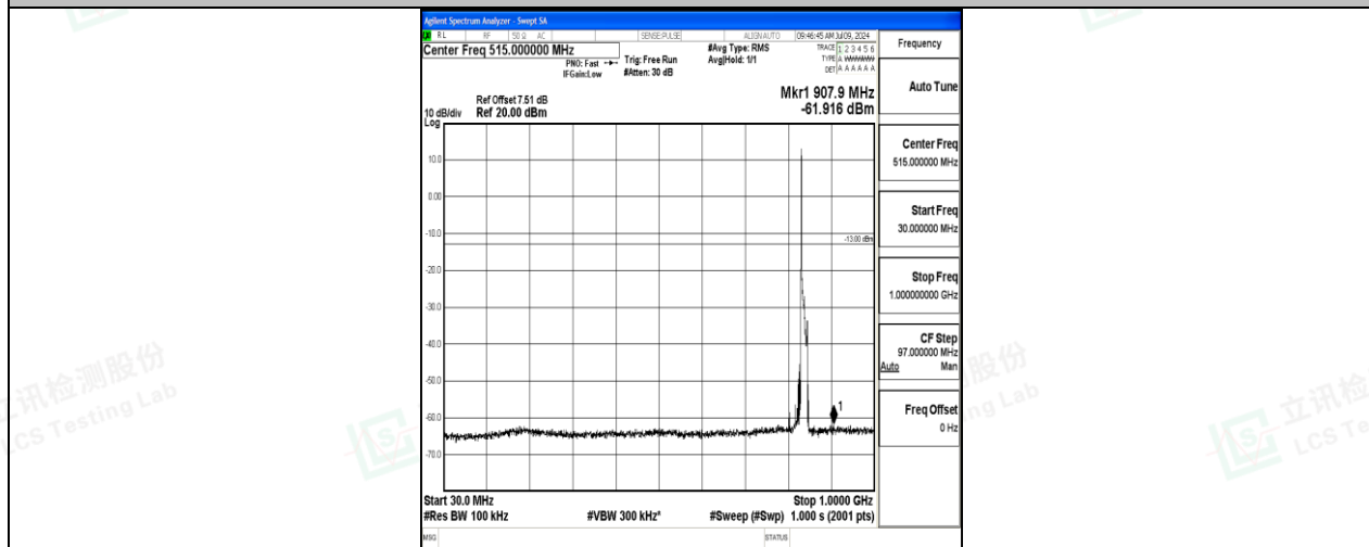
Band26_15MHz_QPSK_26965_1RB#0_30~1000_30~1000
