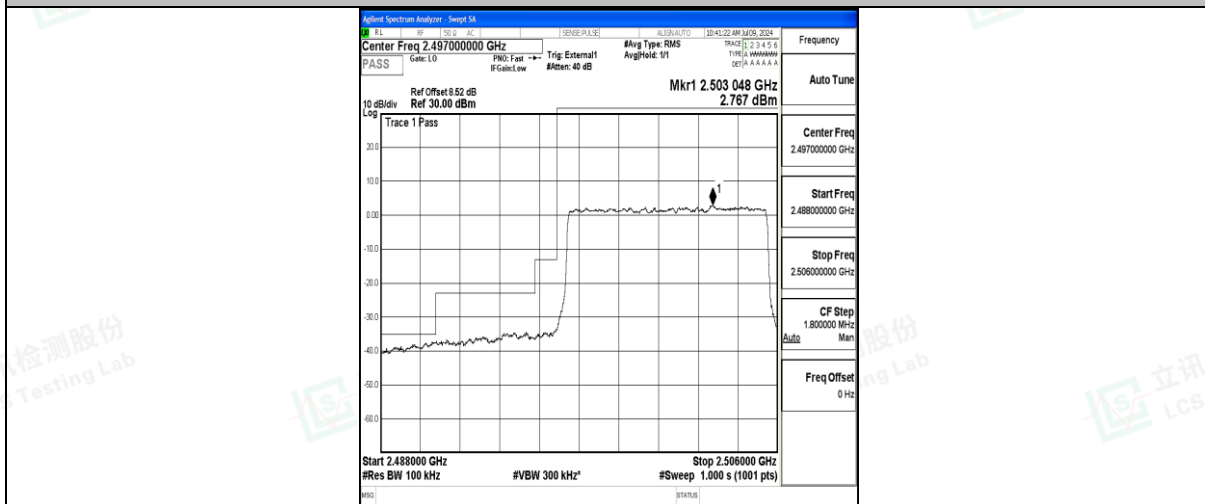
Band41_10MHz_16QAM_39700_50RB#0
