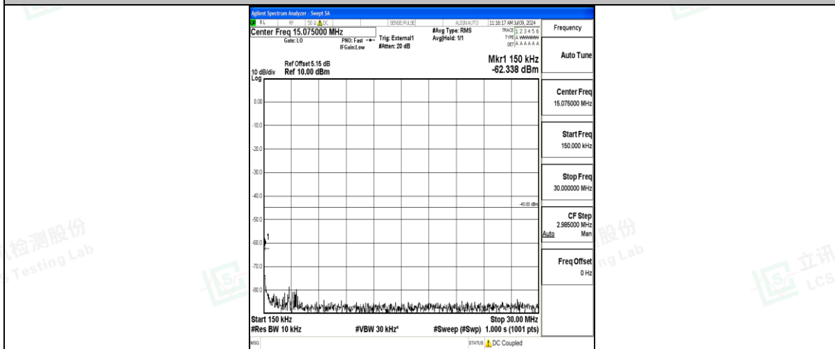
Band41_15MHz_QPSK_39725_1RB#0_0.15~30_0.15~30
