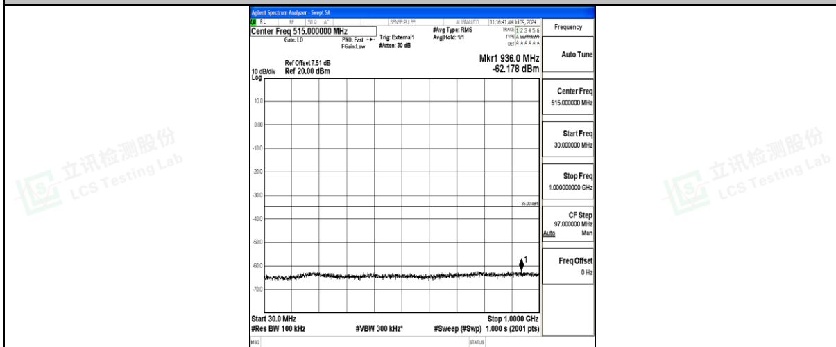
Band41_15MHz_QPSK_39725_1RB#0_30~1000_30~1000
