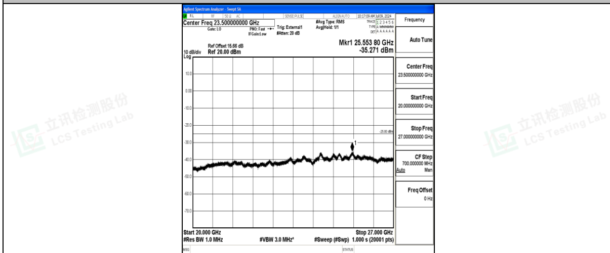
Band41_5MHz_16QAM_41565_1RB#0_20000~27000_20000~27000
