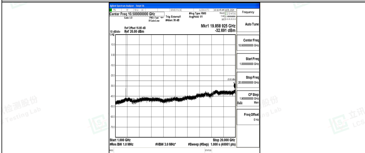
Band41_5MHz_16QAM_41565_1RB#0_1000~20000_1000~20000
