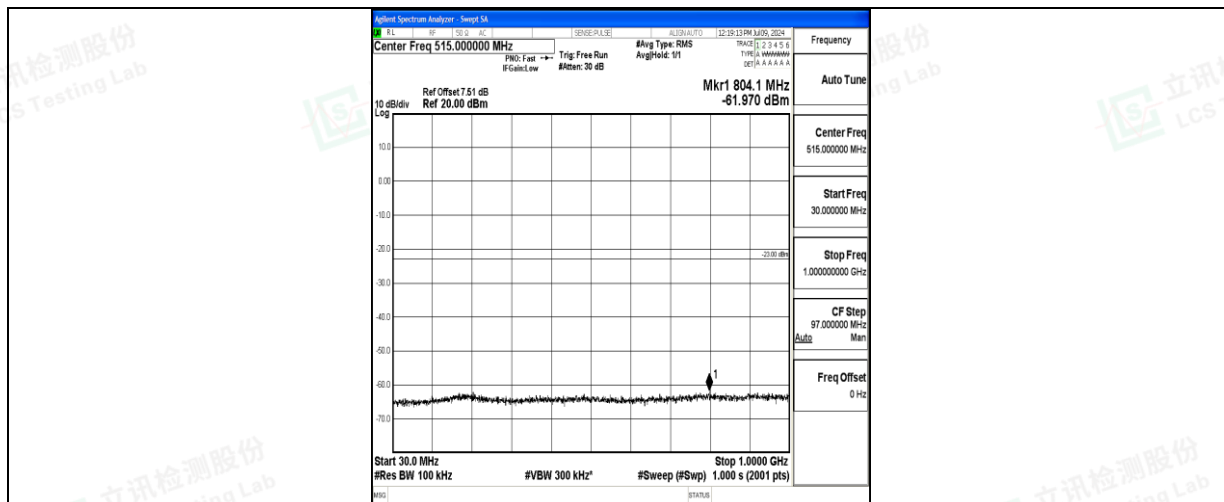
Band66_1.4MHz_QPSK_132665_1RB#0_30~1000_30~1000
