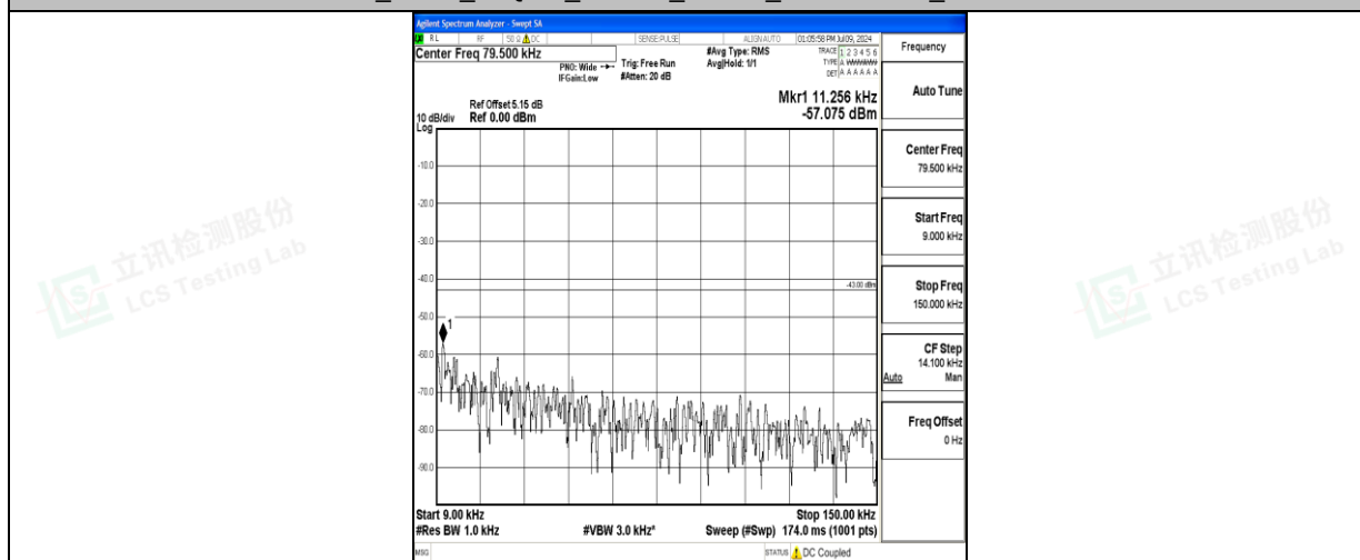
Band66_5MHz_QPSK_131997_1RB#0_0.009~0.15_0.009~0.15
