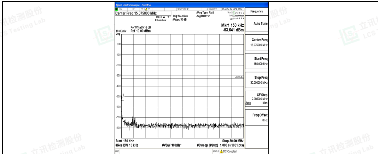
Band66_3MHz_QPSK_131987_1RB#0_0.15~30_0.15~30
