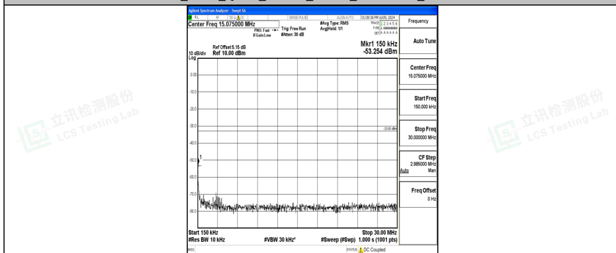
Band66_5MHz_QPSK_132647_1RB#0_0.15~30_0.15~30
