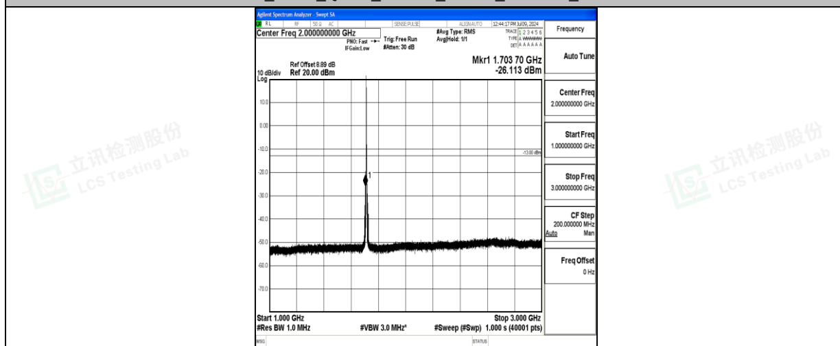
Band66_3MHz_QPSK_131987_1RB#0_1000~3000_1000~3000
