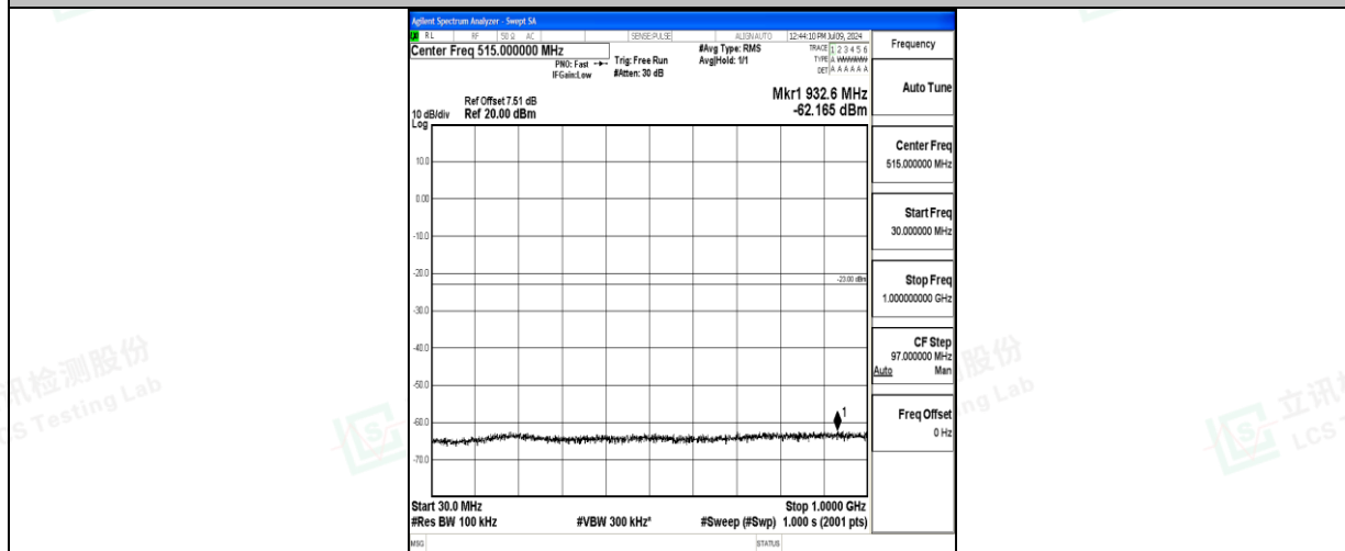
Band66_3MHz_QPSK_131987_1RB#0_30~1000_30~1000
