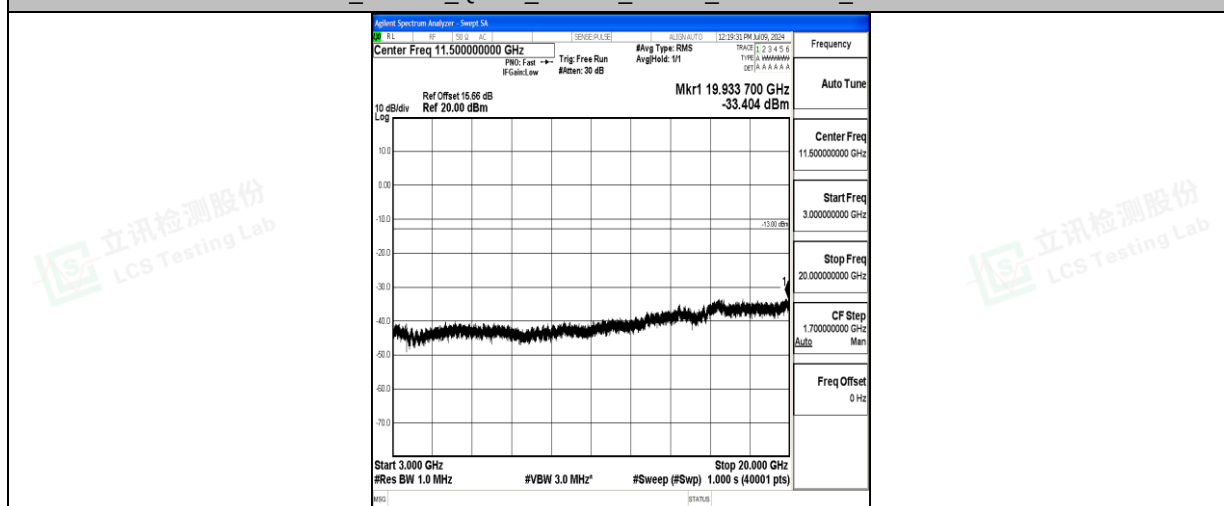
Band66_1.4MHz_QPSK_132665_1RB#0_3000~20000_3000~20000
