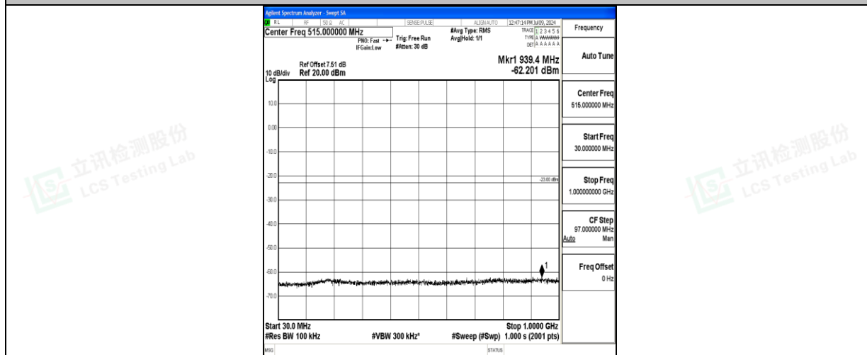
Band66_3MHz_16QAM_132657_1RB#0_30~1000_30~1000
