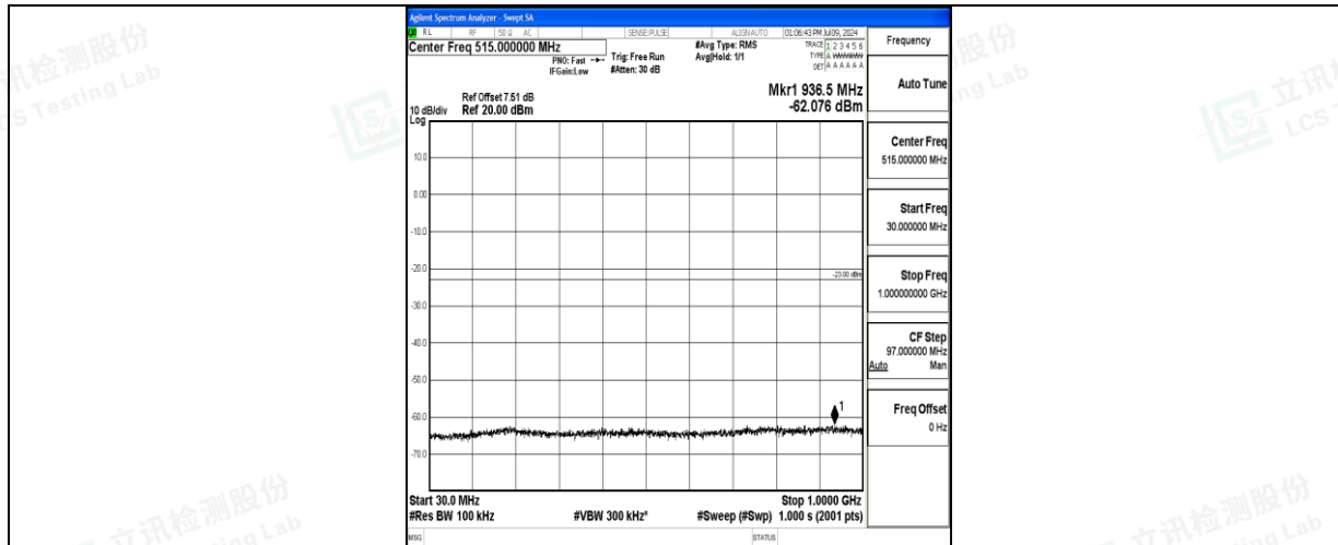
Band66_5MHz_16QAM_131997_1RB#0_30~1000_30~1000
