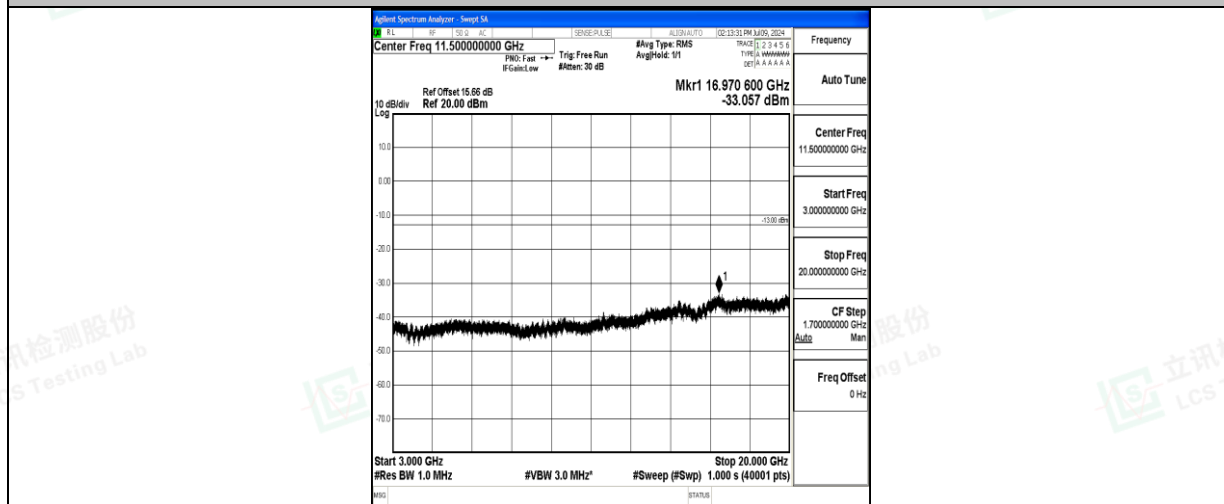
Band66_20MHz_16QAM_132572_1RB#0_3000~20000_3000~20000
