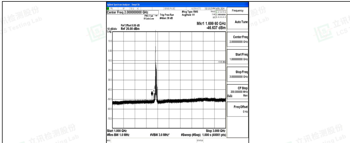
Band66_20MHz_16QAM_132572_1RB#0_1000~3000_1000~3000
