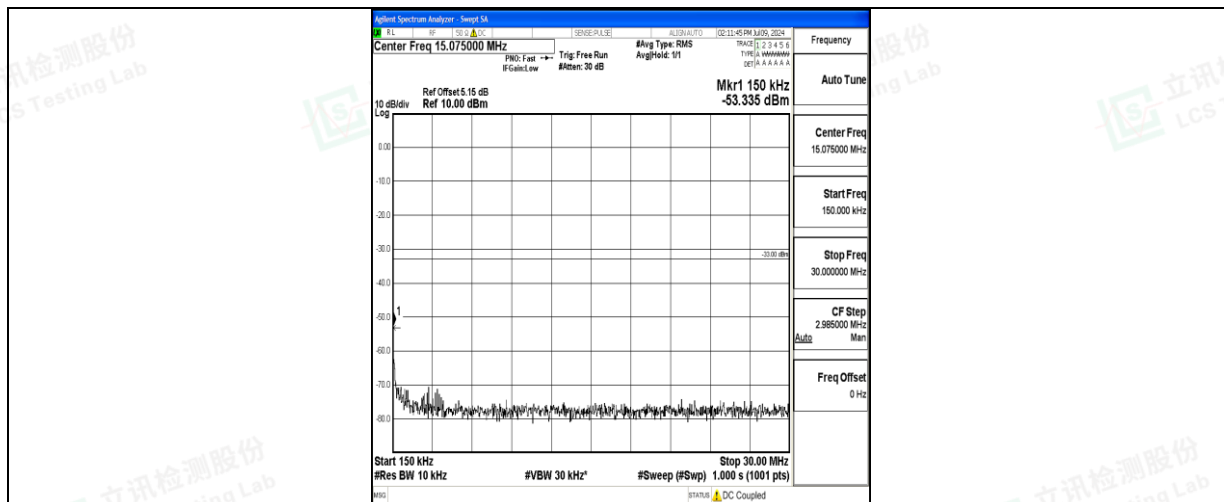
Band66_20MHz_16QAM_132322_1RB#0_0.15~30_0.15~30
