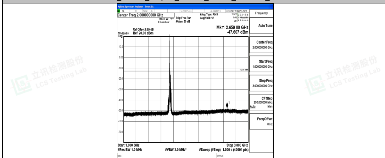
Band66_20MHz_16QAM_132322_1RB#0_1000~3000_1000~3000
