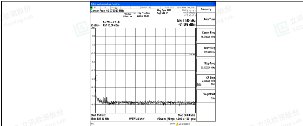
Band71_10MHz_QPSK_133422_1RB#0_0.15~30_0.15~30
