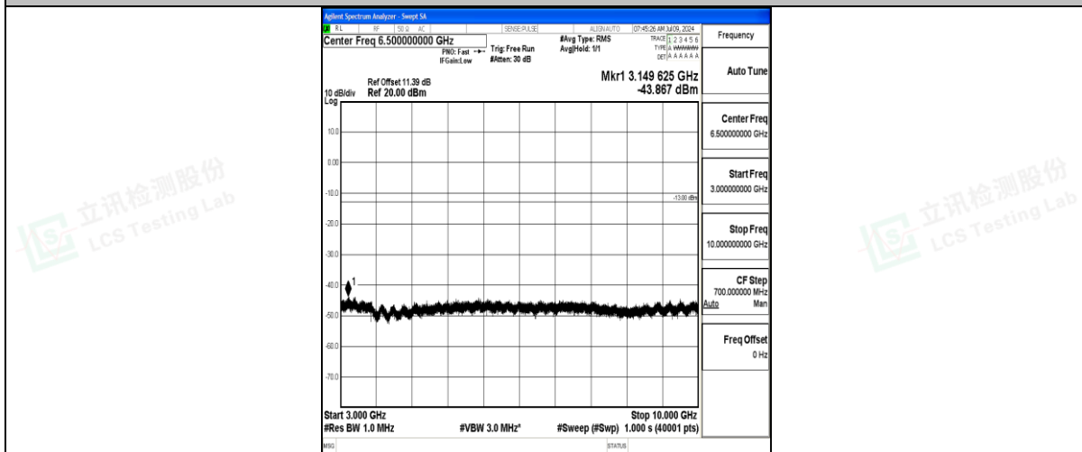
Band71_10MHz_QPSK_133297_1RB#0_3000~10000_3000~10000
