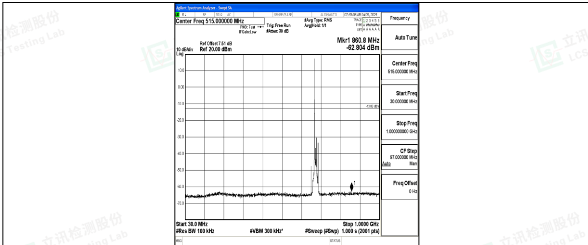
Band71_10MHz_QPSK_133297_1RB#0_30~1000_30~1000
