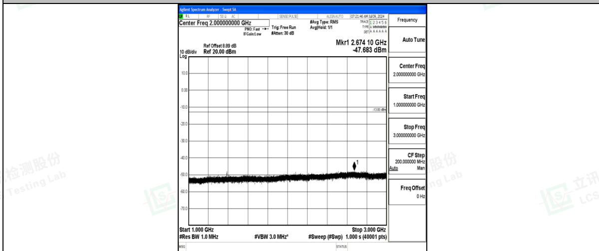
Band71_5MHz_16QAM_133447_1RB#0_1000~3000_1000~3000
