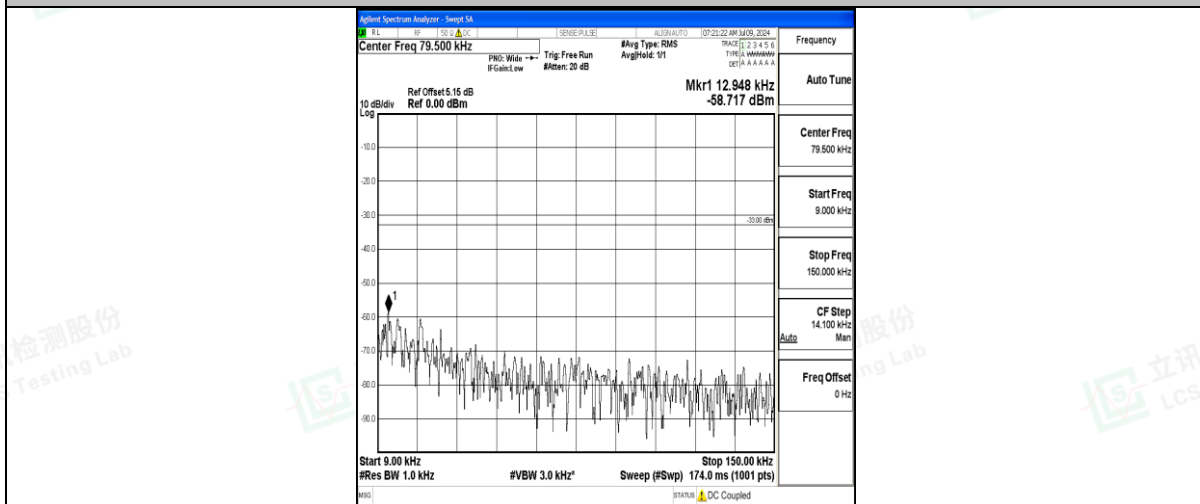
Band71_5MHz_16QAM_133447_1RB#0_0.009~0.15_0.009~0.15
