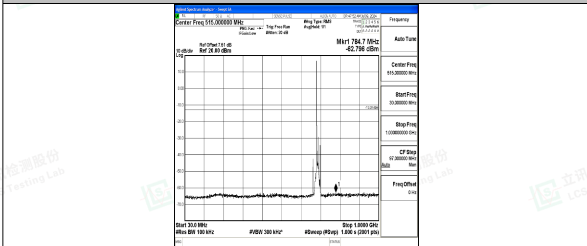
Band71_10MHz_QPSK_133422_1RB#0_30~1000_30~1000
