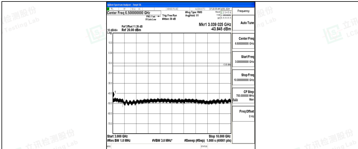
Band71_5MHz_QPSK_133447_1RB#0_3000~10000_3000~10000
