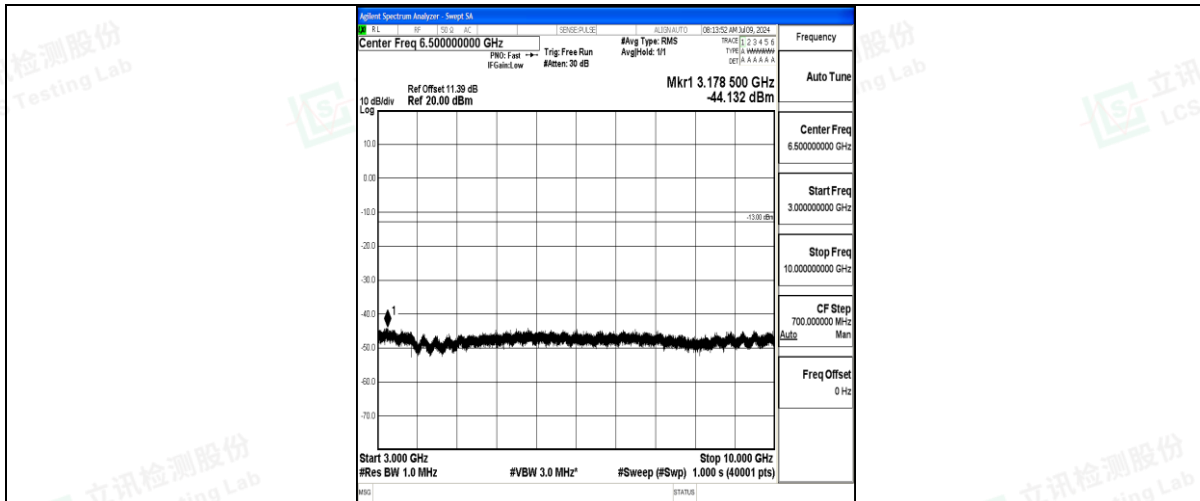
Band71_15MHz_QPSK_133397_1RB#0_3000~10000_3000~10000
