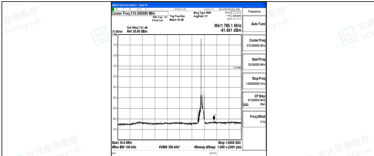
Band71_15MHz_16QAM_133397_1RB#0_30~1000_30~1000
