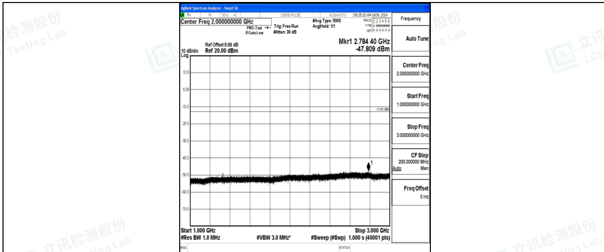
Band71_20MHz_16QAM_133222_1RB#0_1000~3000_1000~3000
