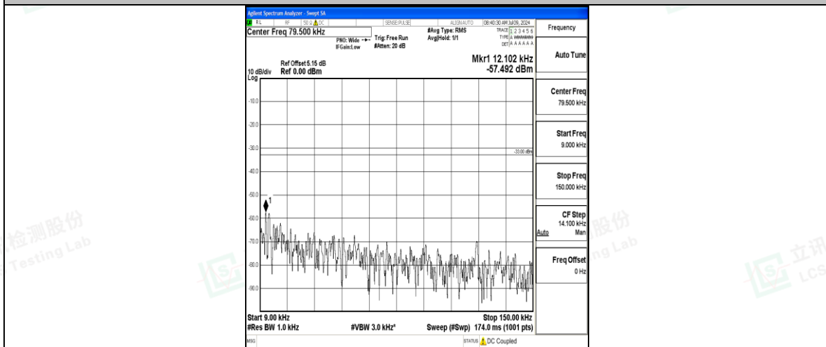
Band71_20MHz_16QAM_133372_1RB#0_0.009~0.15_0.009~0.15
