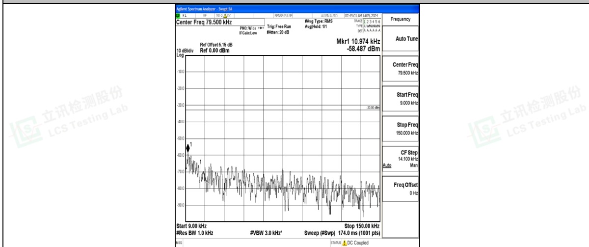
Band71_10MHz_16QAM_133422_1RB#0_0.009~0.15_0.009~0.15
