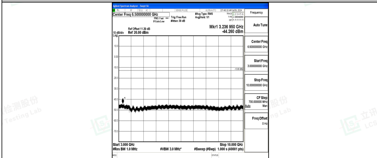
Band71_10MHz_QPSK_133422_1RB#0_3000~10000_3000~10000
