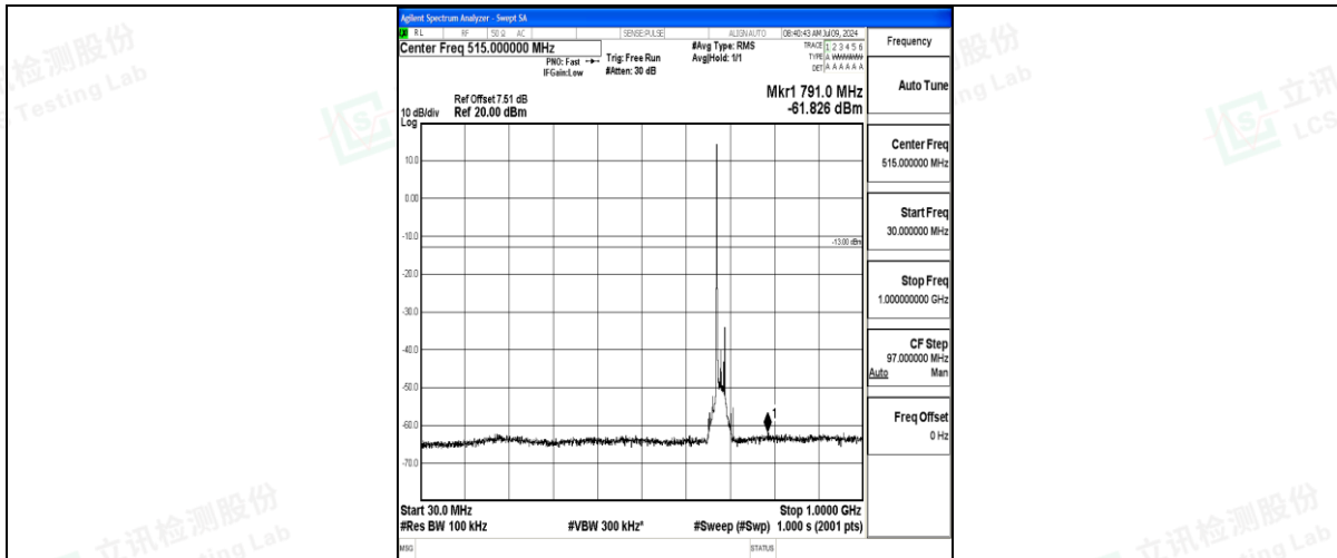
Band71_20MHz_16QAM_133372_1RB#0_30~1000_30~1000
