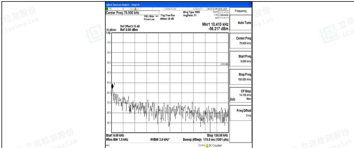
Band71_20MHz_QPSK_133222_1RB#0_0.009~0.15_0.009~0.15
