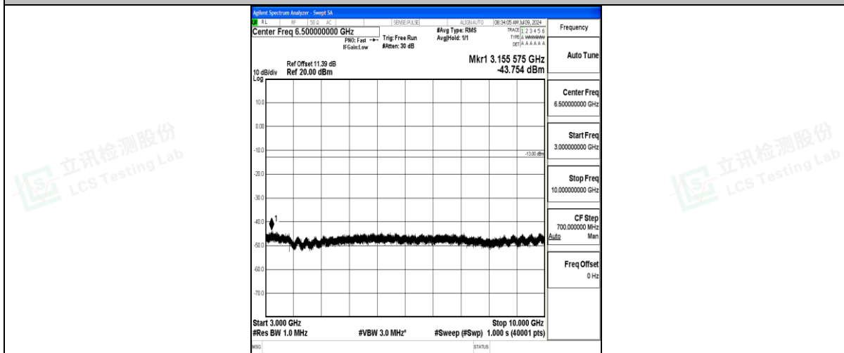
Band71_20MHz_QPSK_133222_1RB#0_3000~10000_3000~10000
