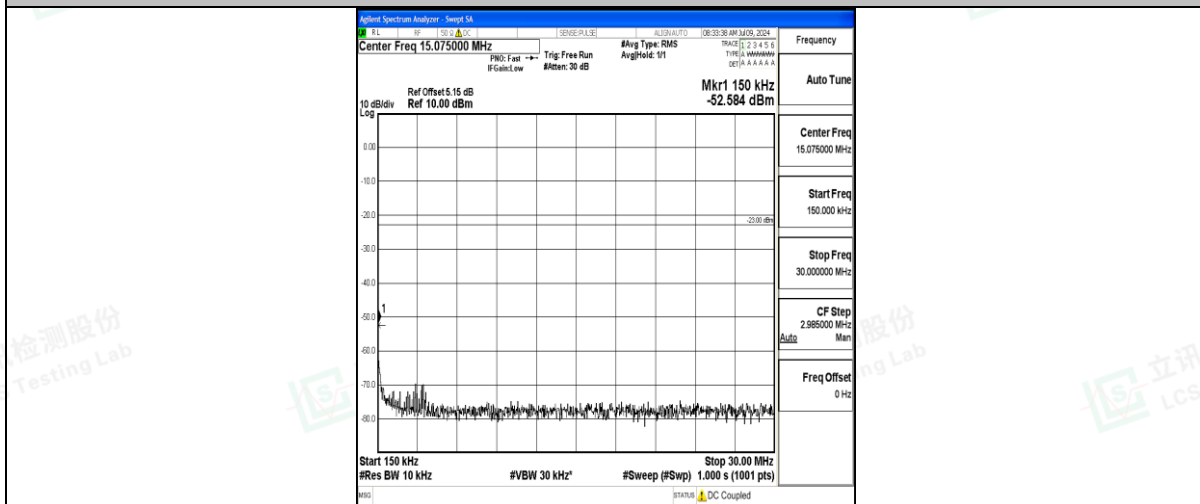
Band71_20MHz_QPSK_133222_1RB#0_0.15~30_0.15~30
