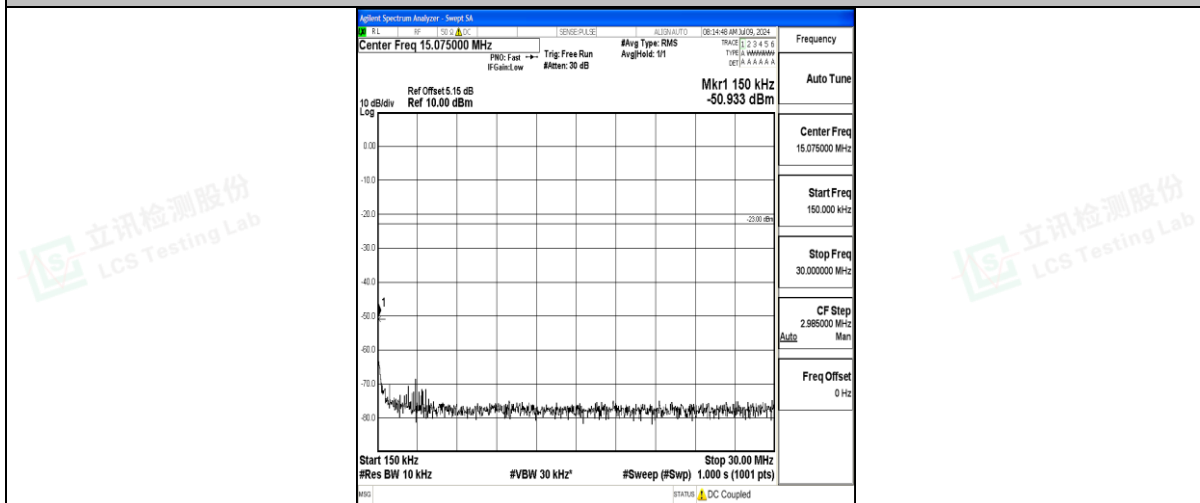
Band71_15MHz_16QAM_133397_1RB#0_0.15~30_0.15~30
