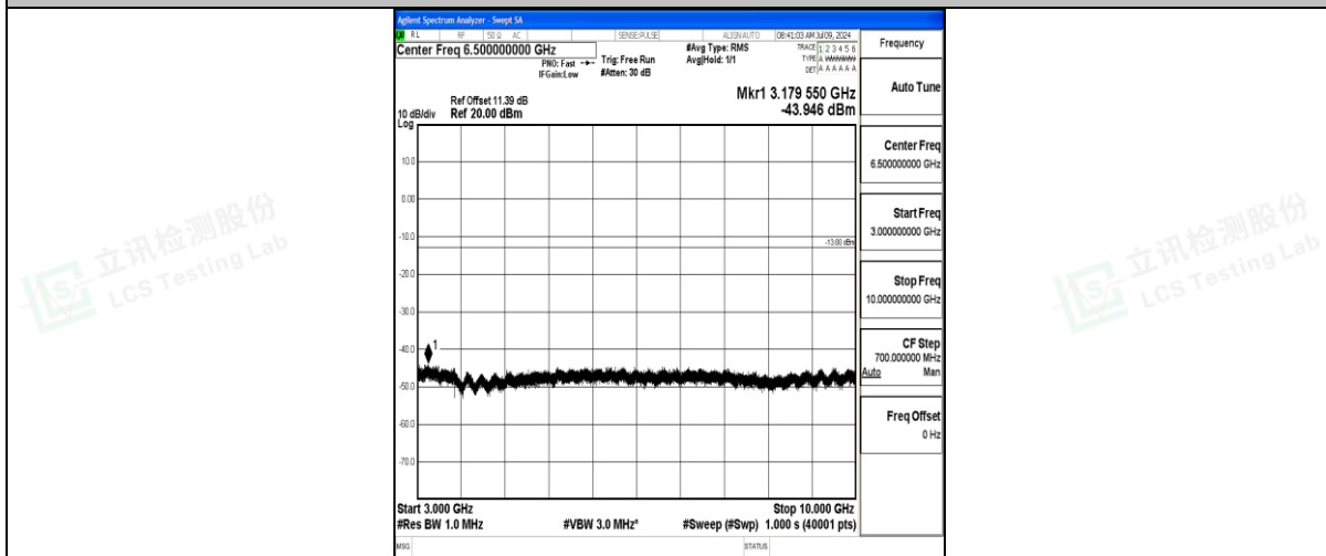
Band71_20MHz_16QAM_133372_1RB#0_3000~10000_3000~10000
