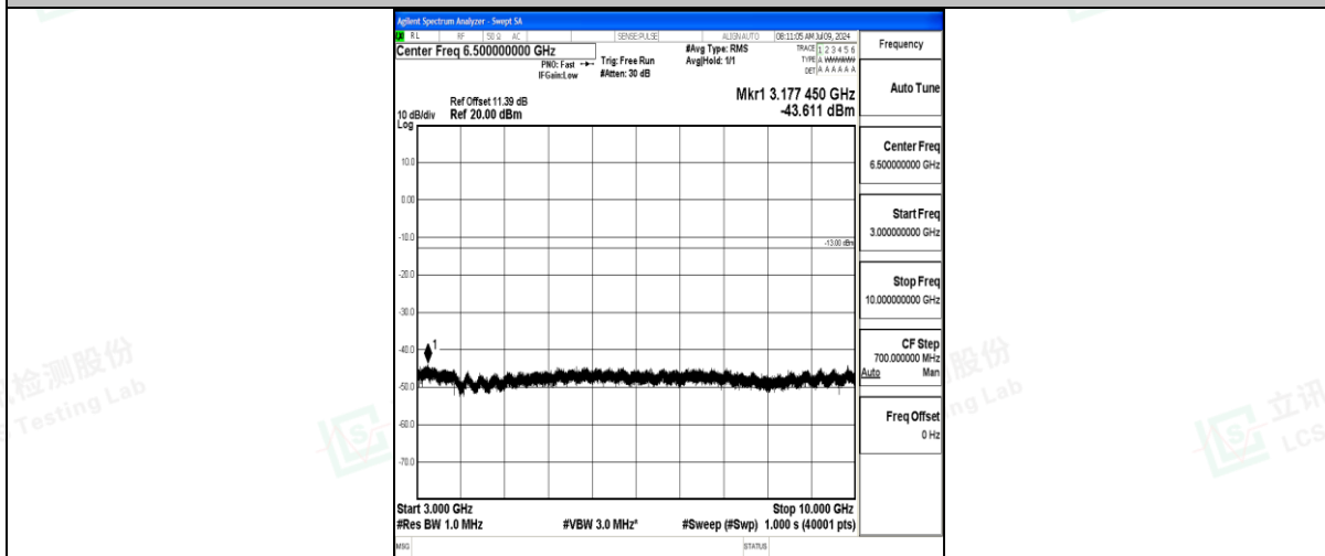
Band71_15MHz_QPSK_133297_1RB#0_3000~10000_3000~10000
