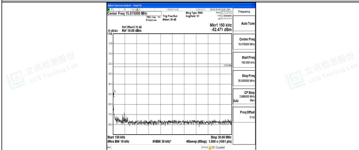
Band71_20MHz_16QAM_133372_1RB#0_0.15~30_0.15~30
