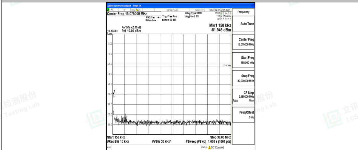
Band71_20MHz_16QAM_133322_1RB#0_0.15~30_0.15~30
