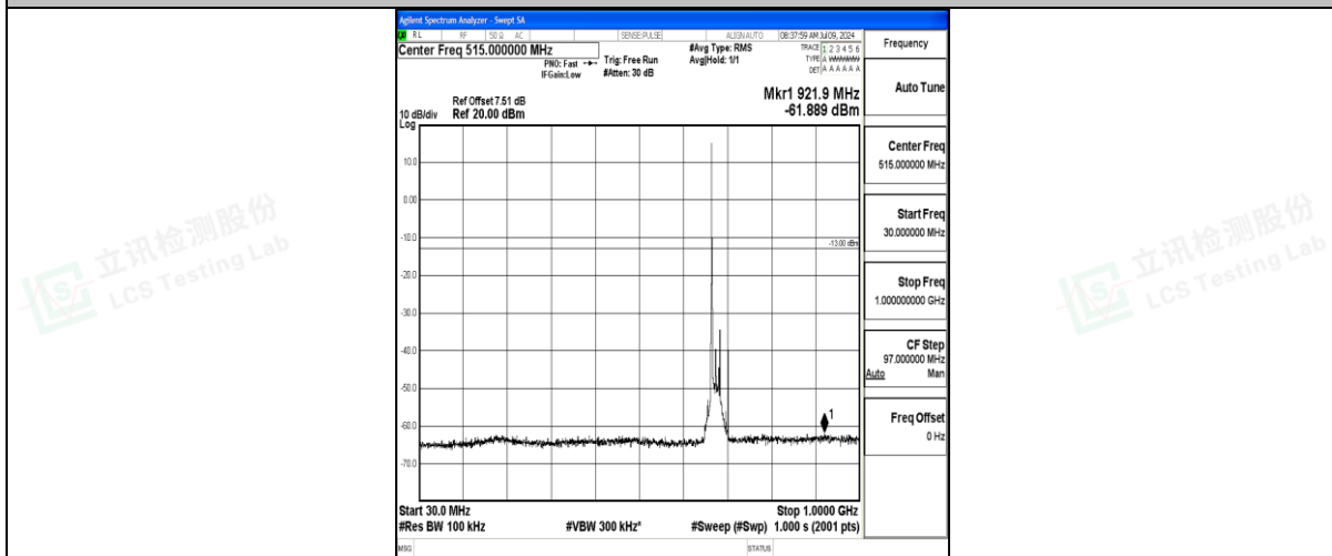
Band71_20MHz_16QAM_133322_1RB#0_30~1000_30~1000
