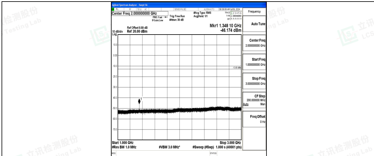
Band71_20MHz_16QAM_133322_1RB#0_1000~3000_1000~3000
