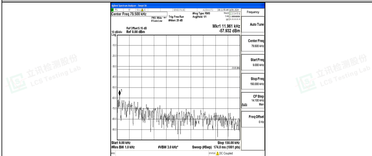
Band71_15MHz_16QAM_133297_1RB#0_0.009~0.15_0.009~0.15
