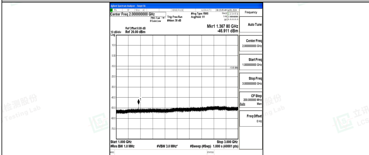
Band71_15MHz_16QAM_133397_1RB#0_1000~3000_1000~3000
