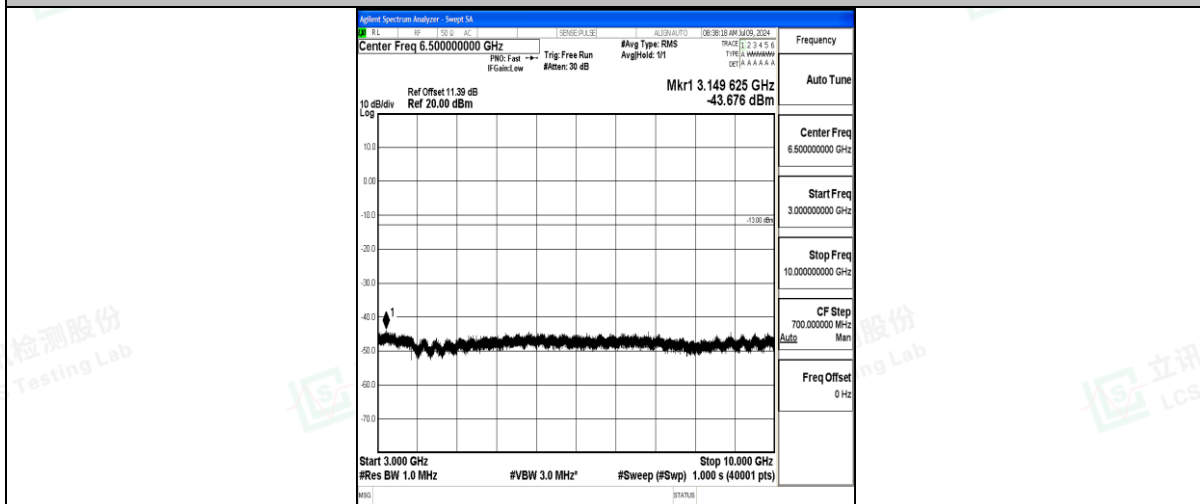
Band71_20MHz_16QAM_133322_1RB#0_3000~10000_3000~10000
