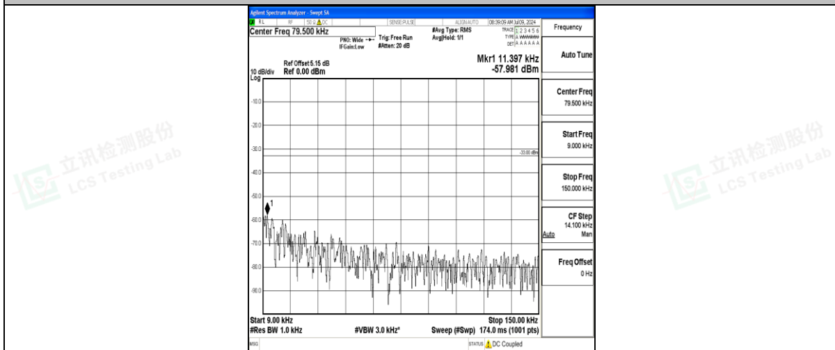
Band71_20MHz_QPSK_133372_1RB#0_0.009~0.15_0.009~0.15
