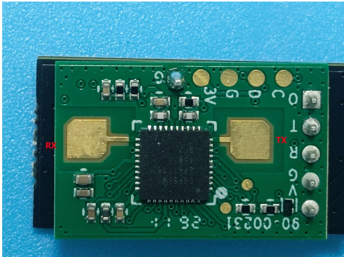
24G Radar Antenna
