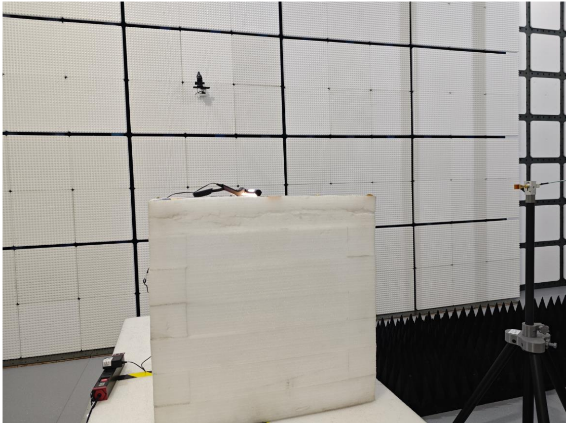
Radiated Emission 90-100GHz View
