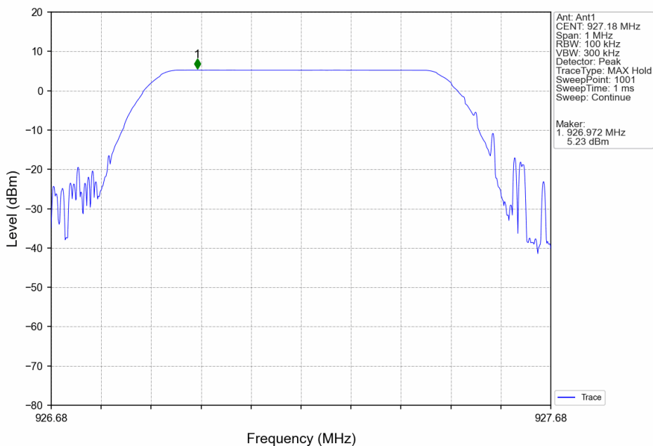
915_HCH_927.18MHz_Ant1_NTNV
