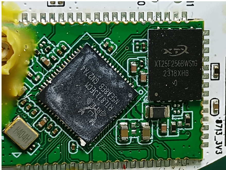
2.4G Wi-Fi/BLE Radio 2 Chip
