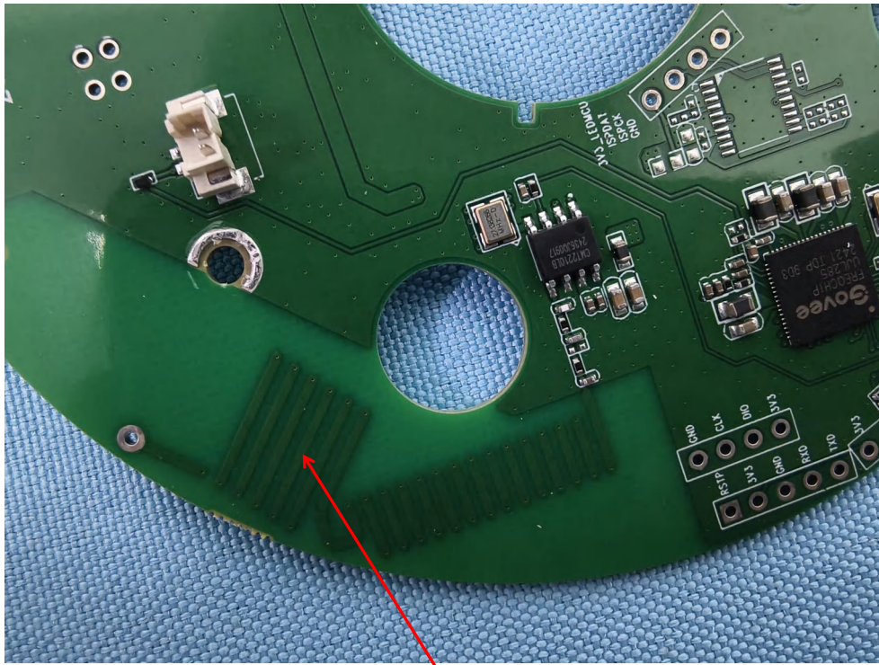
433.92MHz-RX-ANT
