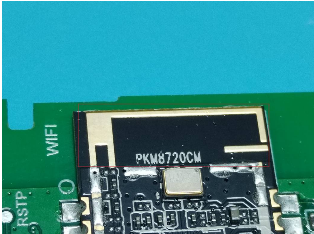
Wi-Fi Antenna
