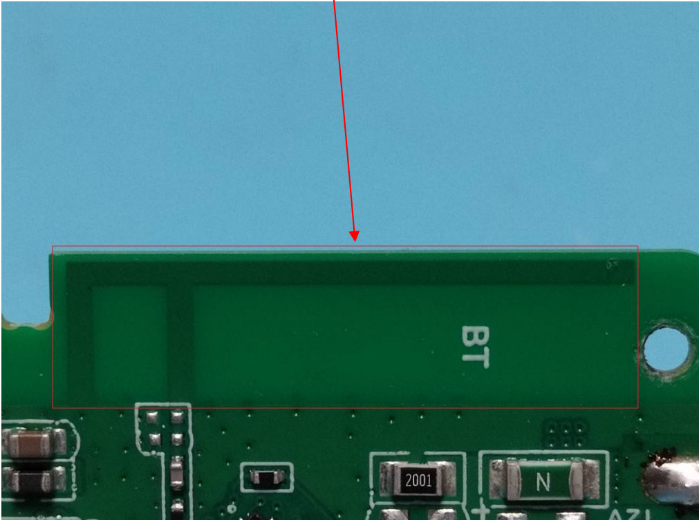
BT Antenna
