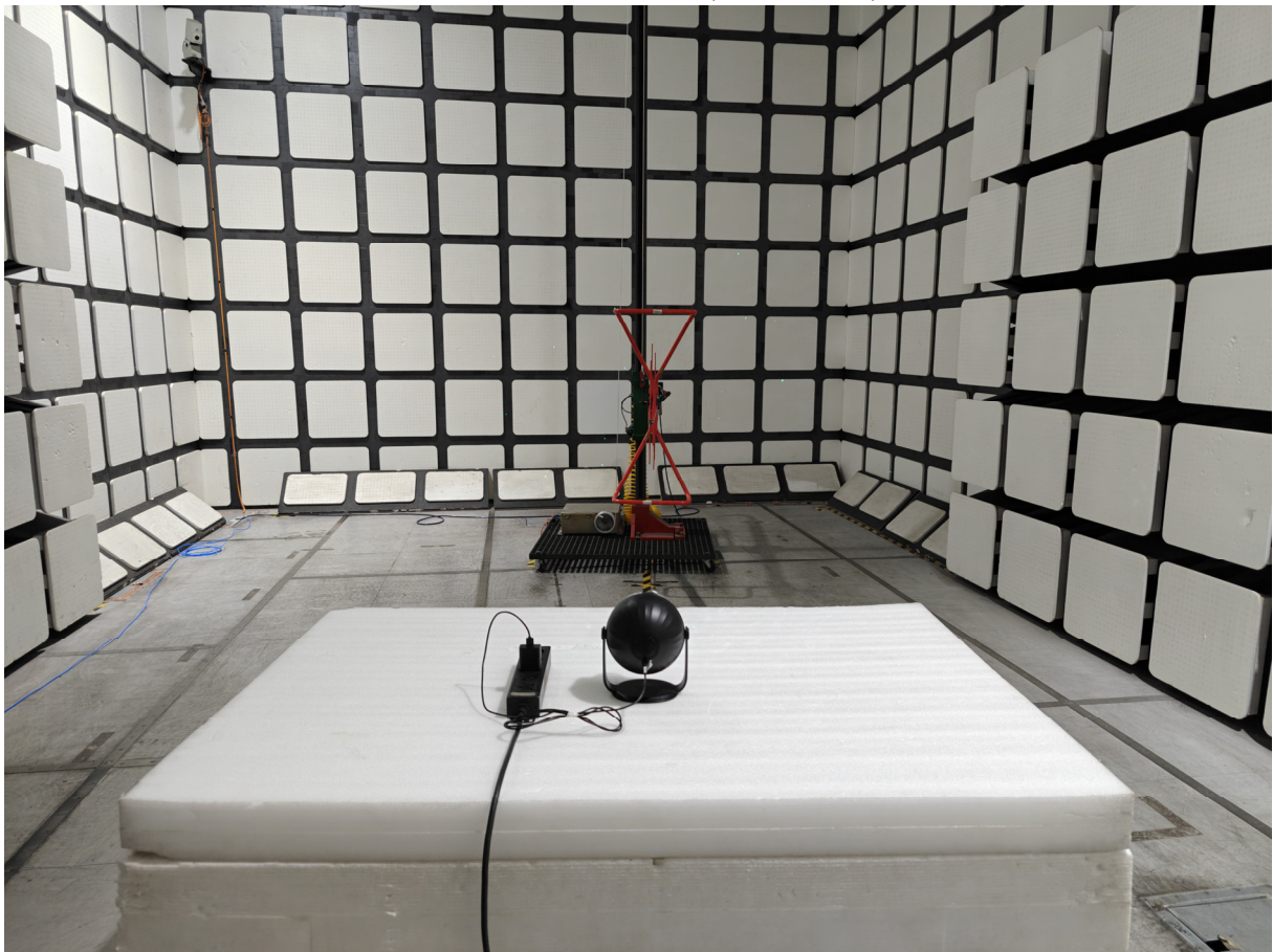
Radiated Emissions View (Below 1 GHz)
