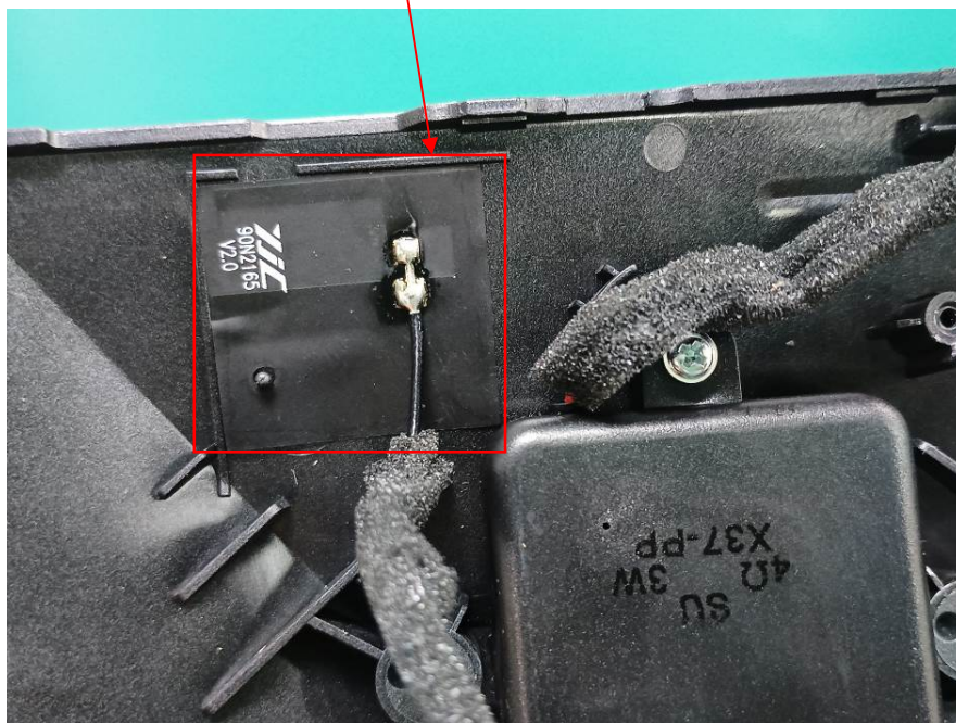
BLE&2.4WIFI ANT
