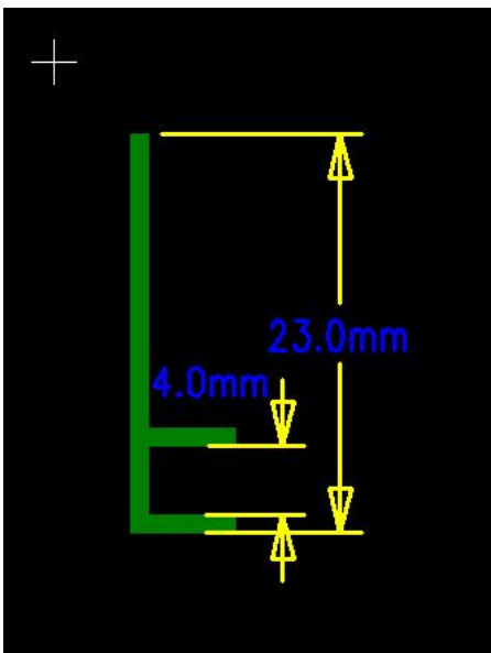
5. WIFI Antenna Physical Size
