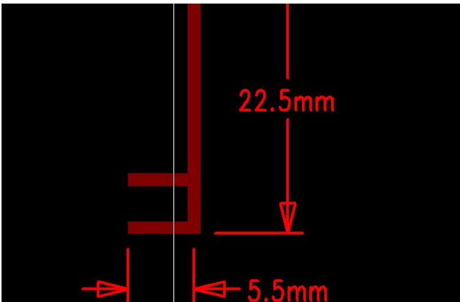
5. WIFI Antenna Physical Size
