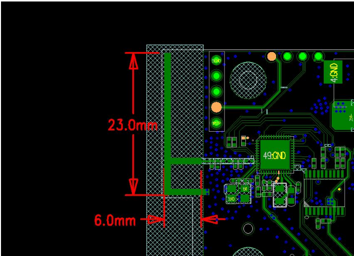
5. WIFI Antenna Physical Size
