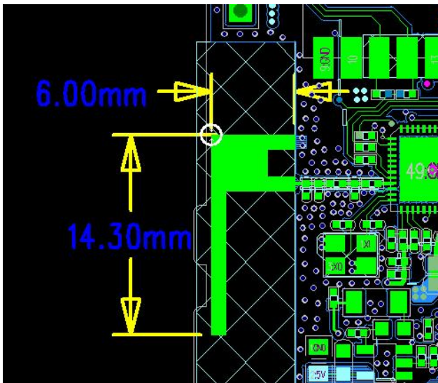
4. Bluetooth Antenna Physical Size
