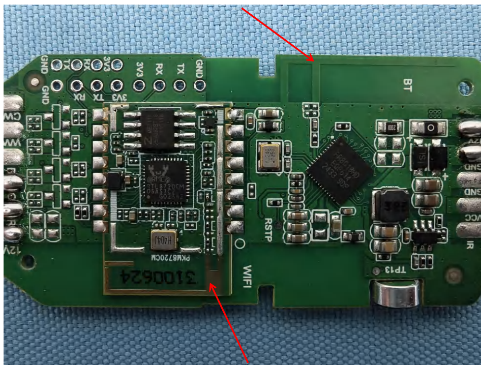
WiFi-ANT
