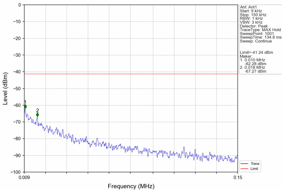
1M_LCH_2402MHz_Ant1_NTNV
