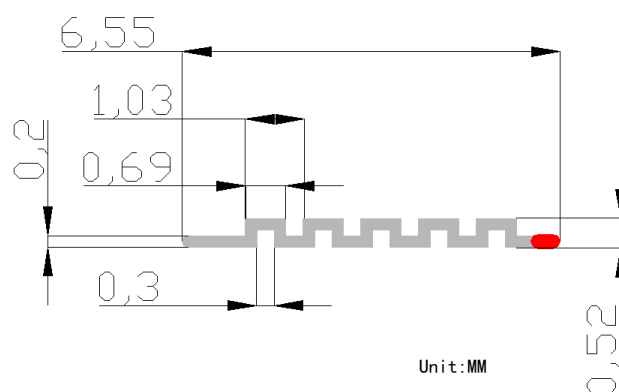
Figure 2: Specification and size of Bluetooth antenna
