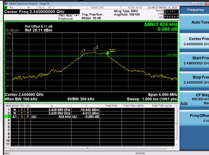
BLE_1M-Ant1-2440-PASS
