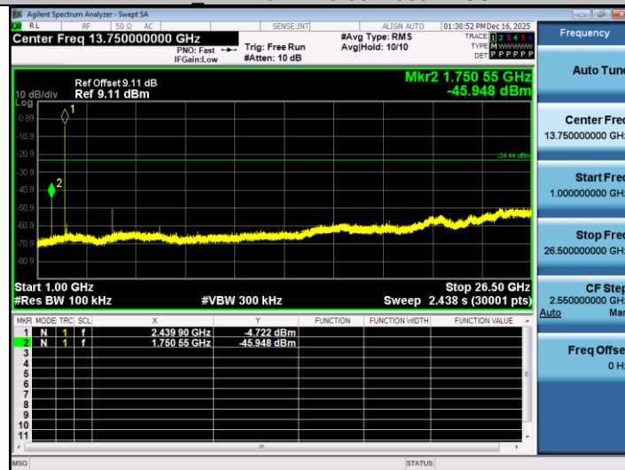
BLE_1M-Ant1-2440-1000~26500-PASS
