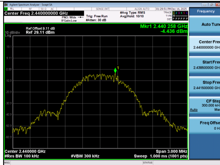
BLE_1M-Ant1-2440-0-Reference-PASS
