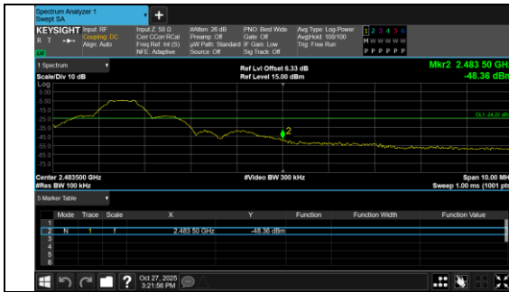
Out Of Band Emission BLE 1M_Channel 39
