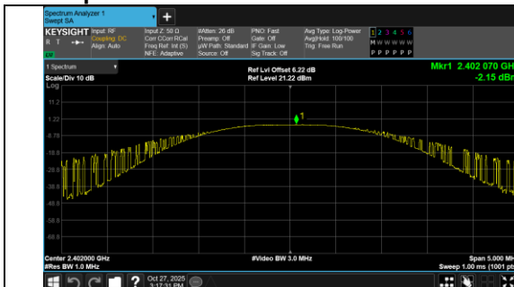
Peak Output Power BLE 1M_Channel 0
